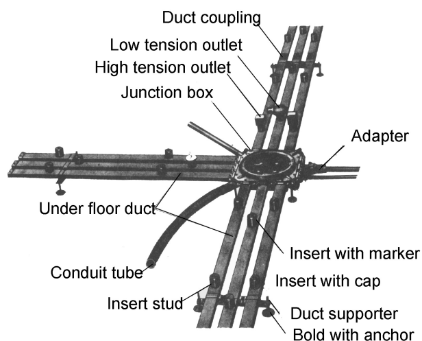
Figure II-5 Outline of under floor duct system
