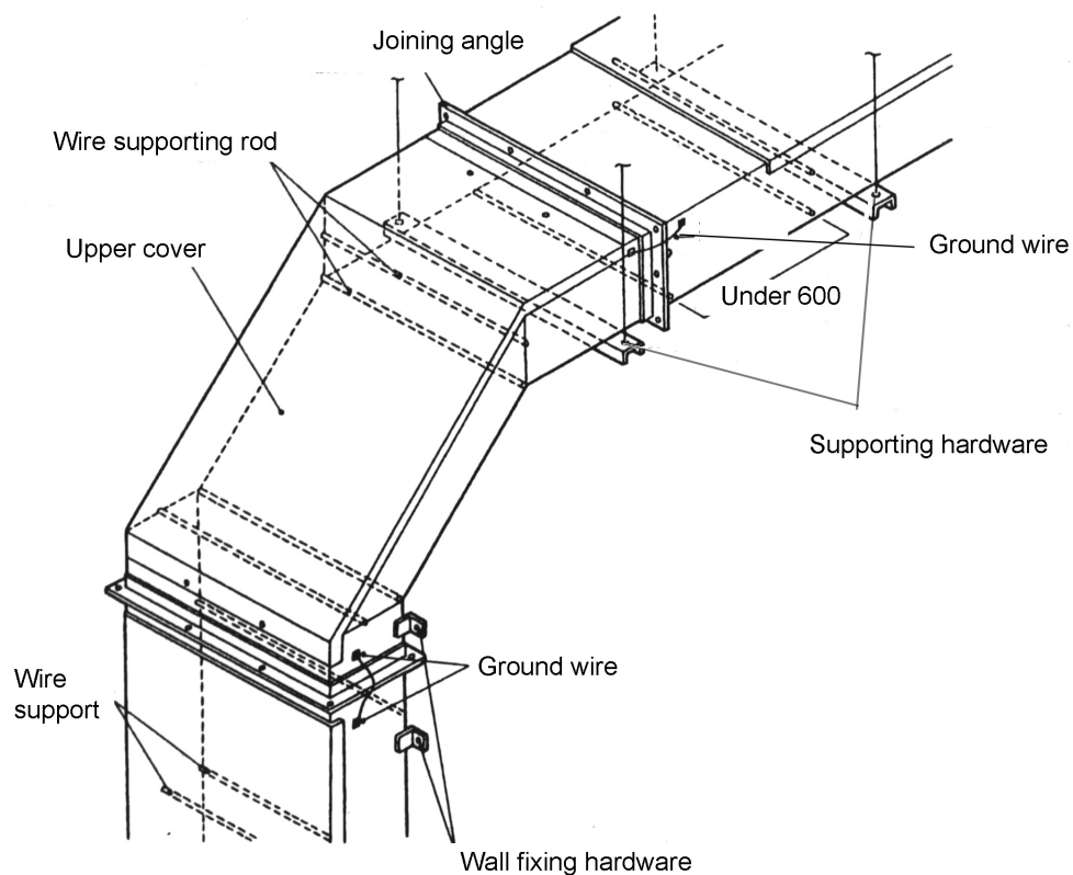
Figure II-2 Metal duct system
