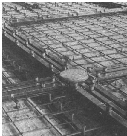
Figure II-6 Example of under floor duct installation
