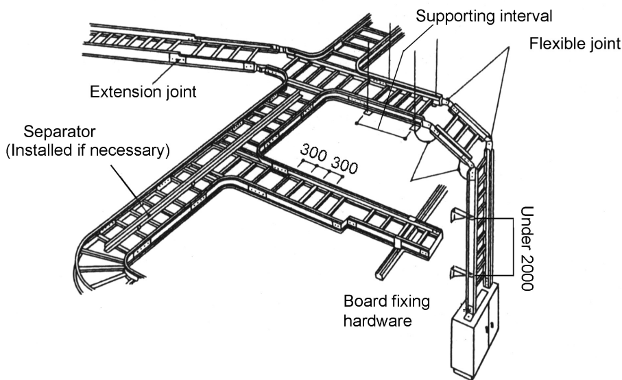
Figure II-1 Example of ladder cable tray system
