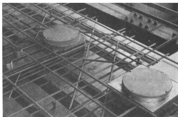
Figure II-8 Example of cellular raceway installation
