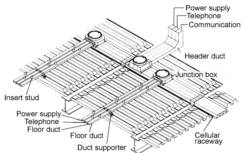
Figure II-7 Outline of cellular raceway system
