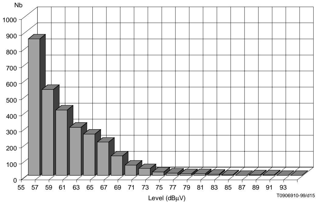
Figure 15 – Number of ingress jammers occurrences at different levels
