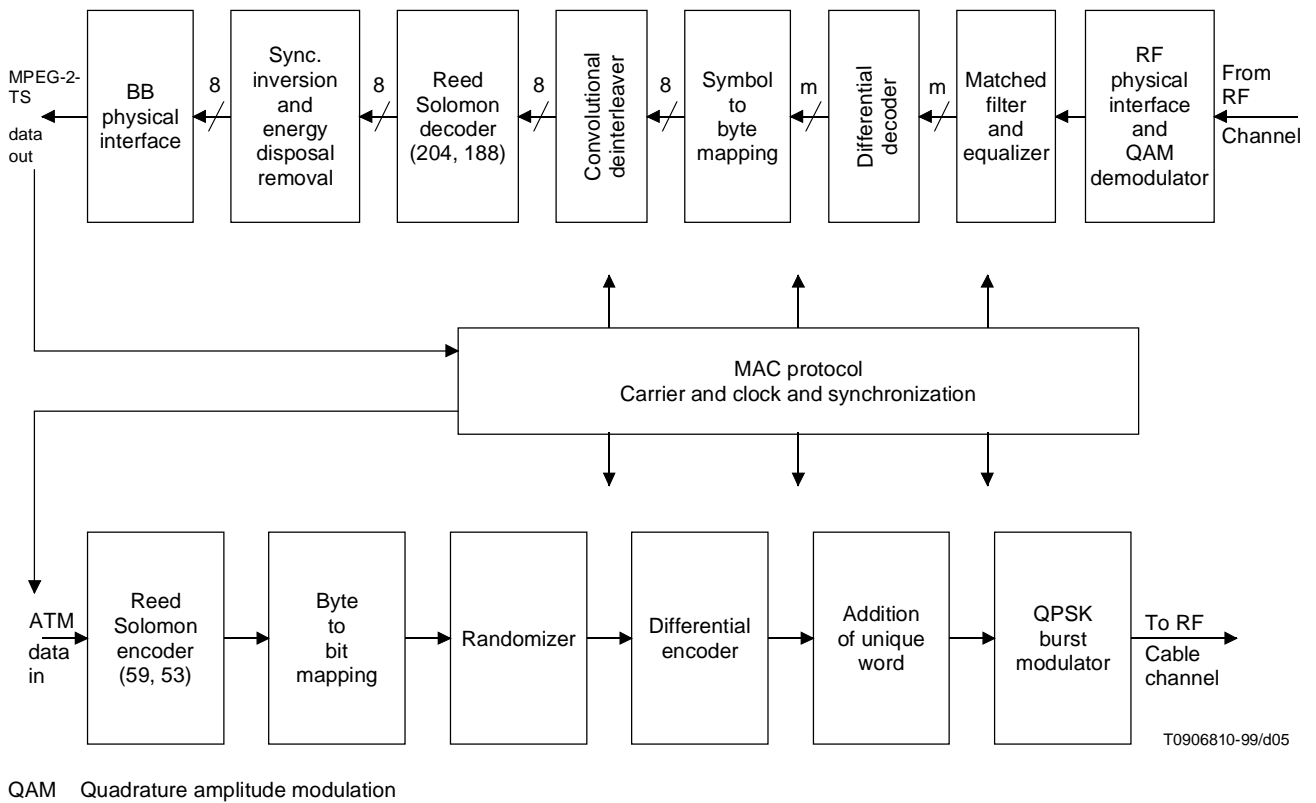
Figure 5 – Conceptual block diagram for the IB NIU transceiver
