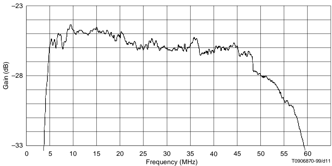
Figure 11 – Typical return path gain
