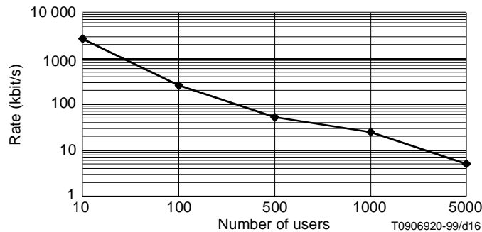
Figure 16 – Estimated average rate per user as a function of the number of users connected
