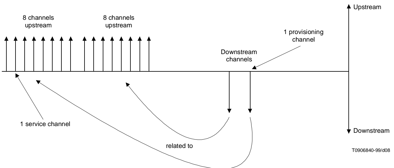
Figure 8 – Example of frequency allocation
