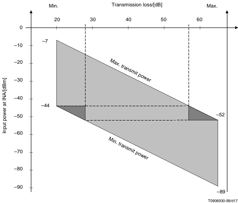
Figure 17 – Possible power range at INA of the upstream signal
