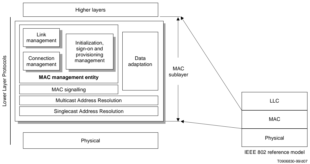
Figure 7 – MAC reference model
