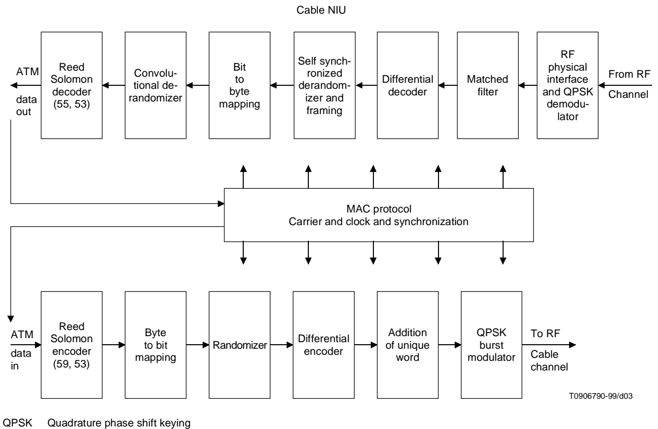
Figure 3 – Conceptual block diagram for the NIU OOB transceiver
