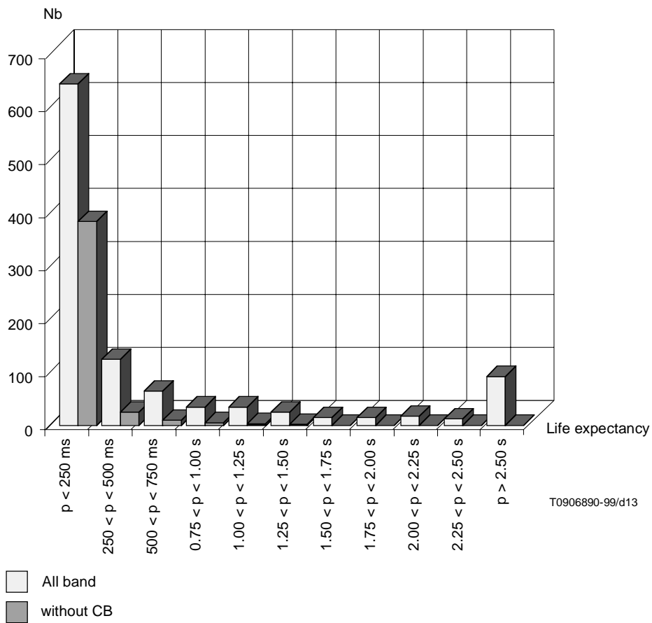
Figure 13 – Life expectancy of ingress jammers taking into account the CB radio band or not
