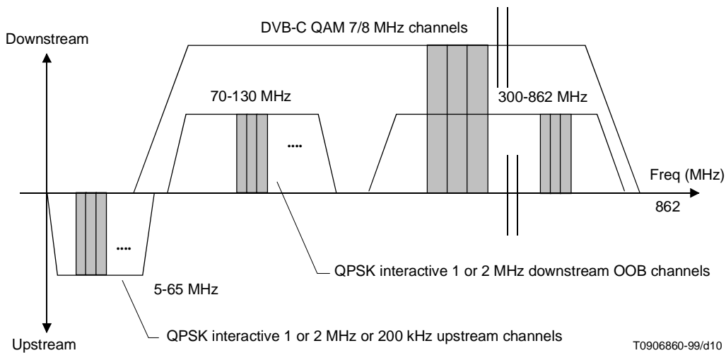
Figure 10 – Preferred frequency ranges for CATV interactive systems
