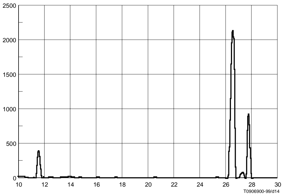
Figure 14 – Number of ingress jammers recorded over a 40-hour period
