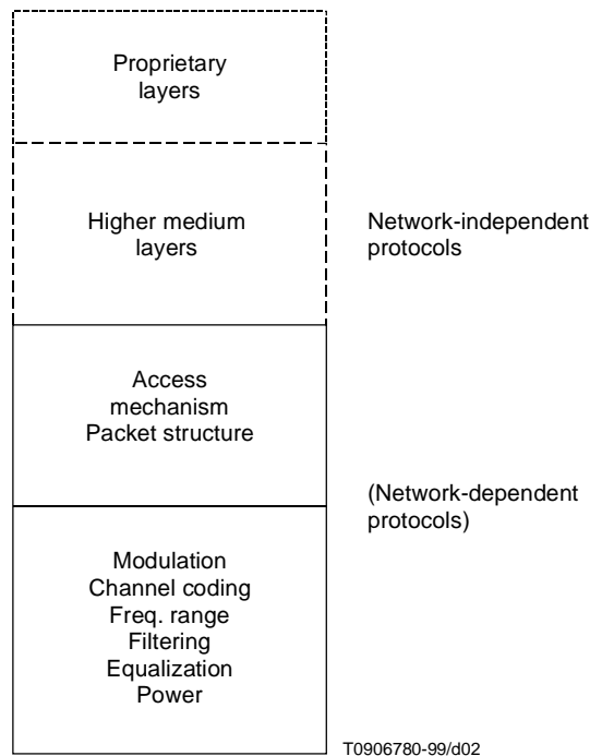
Figure 2 – Layer structure for generic system reference model
