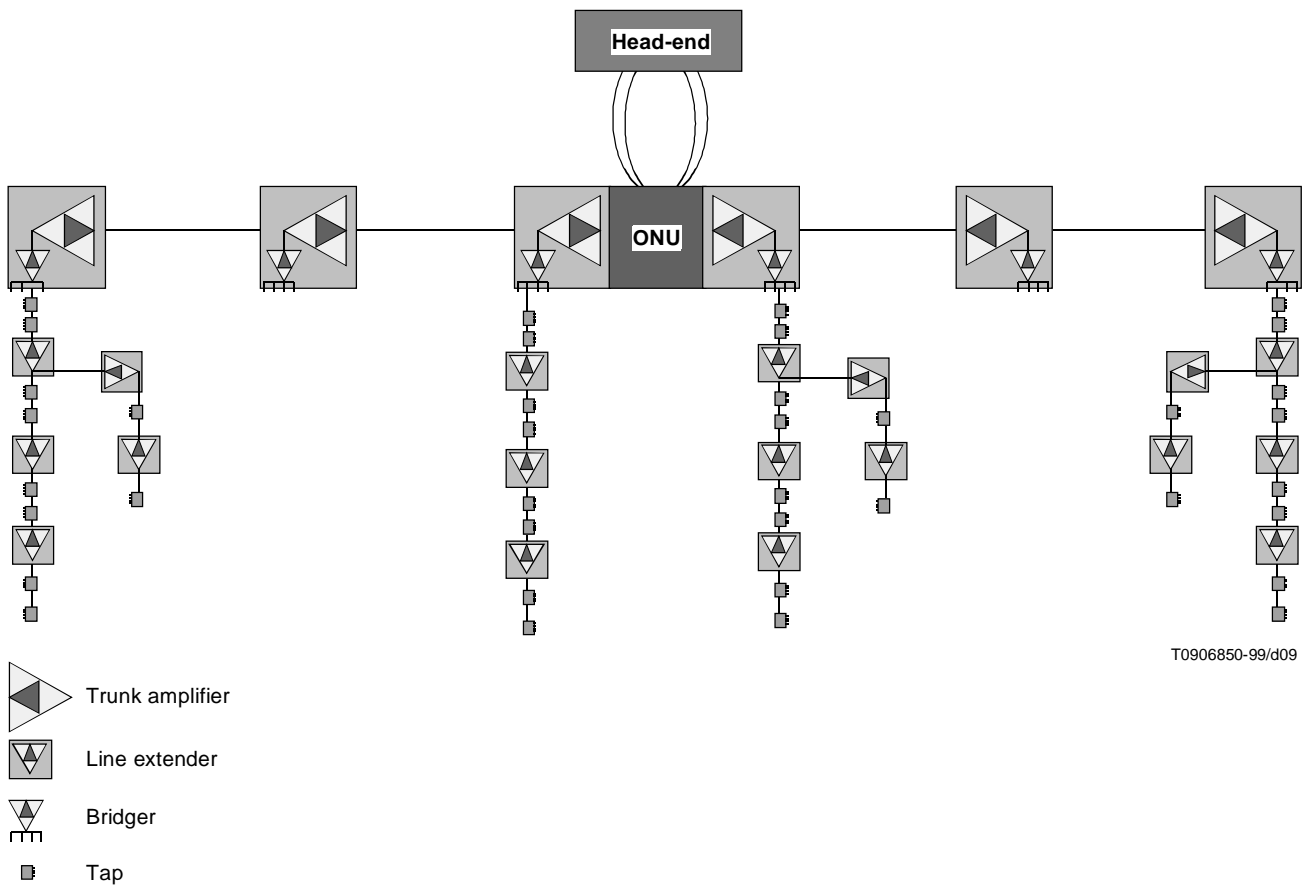
Figure 9 – Typical HFC networks
