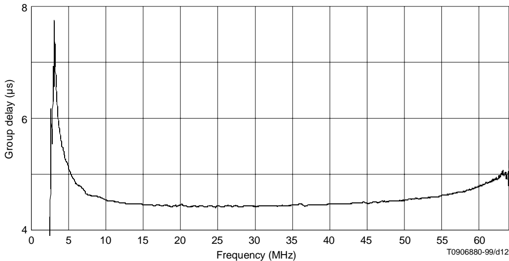
Figure 12 – Typical return path group delay
