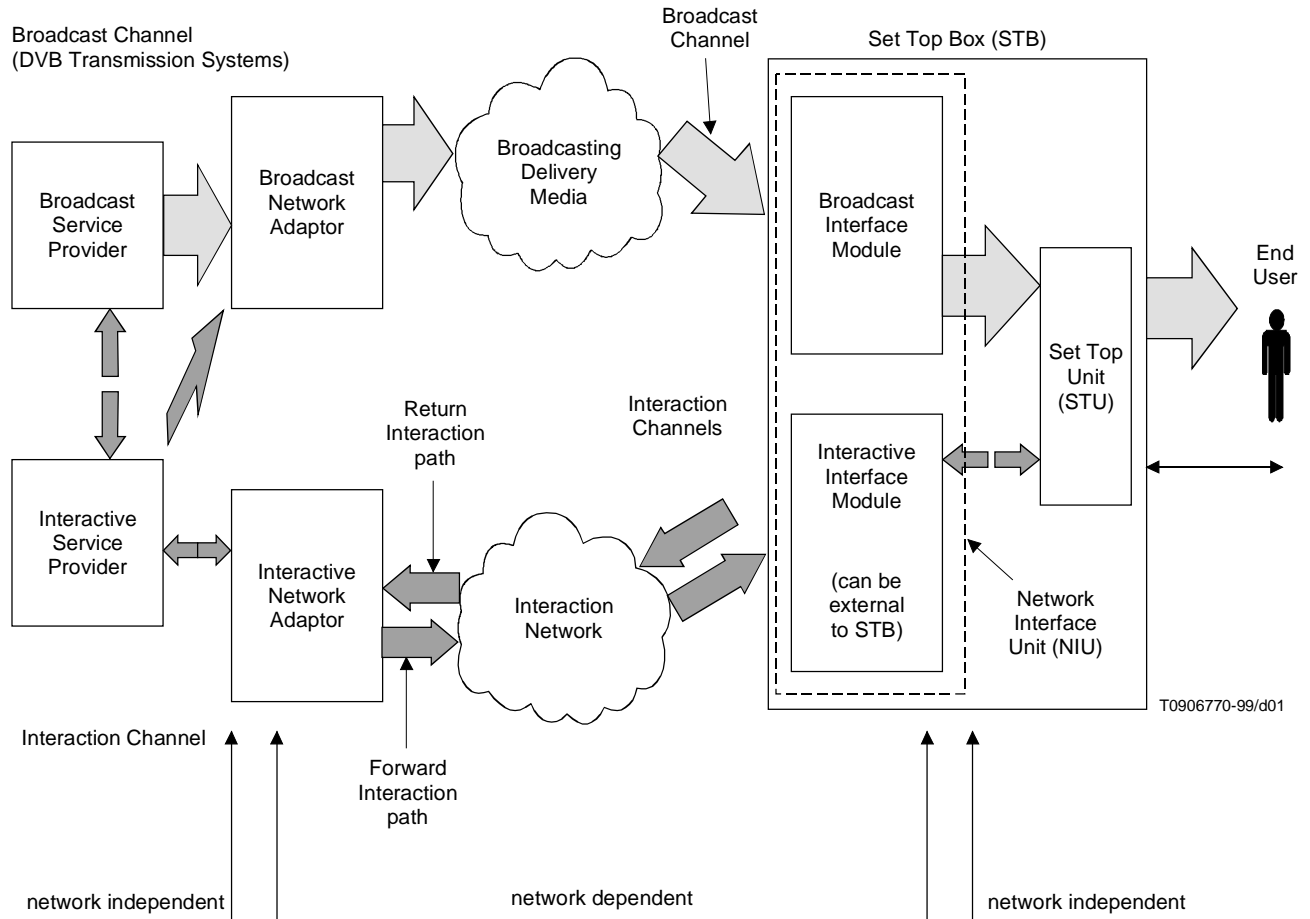
Figure 1 – Generic system reference model for interactive systems
