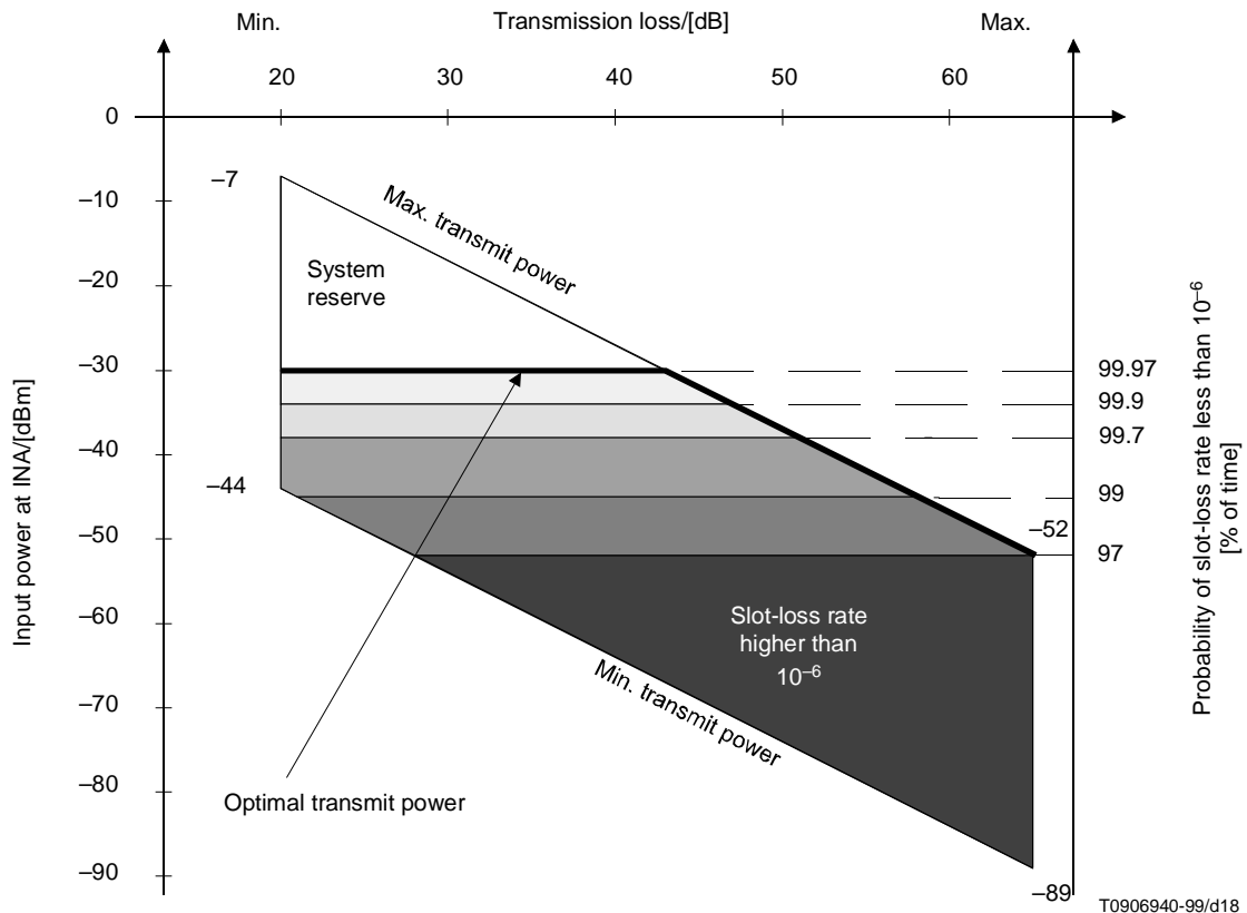
Figure 18 – Possible power range at INA of the upstream signal
