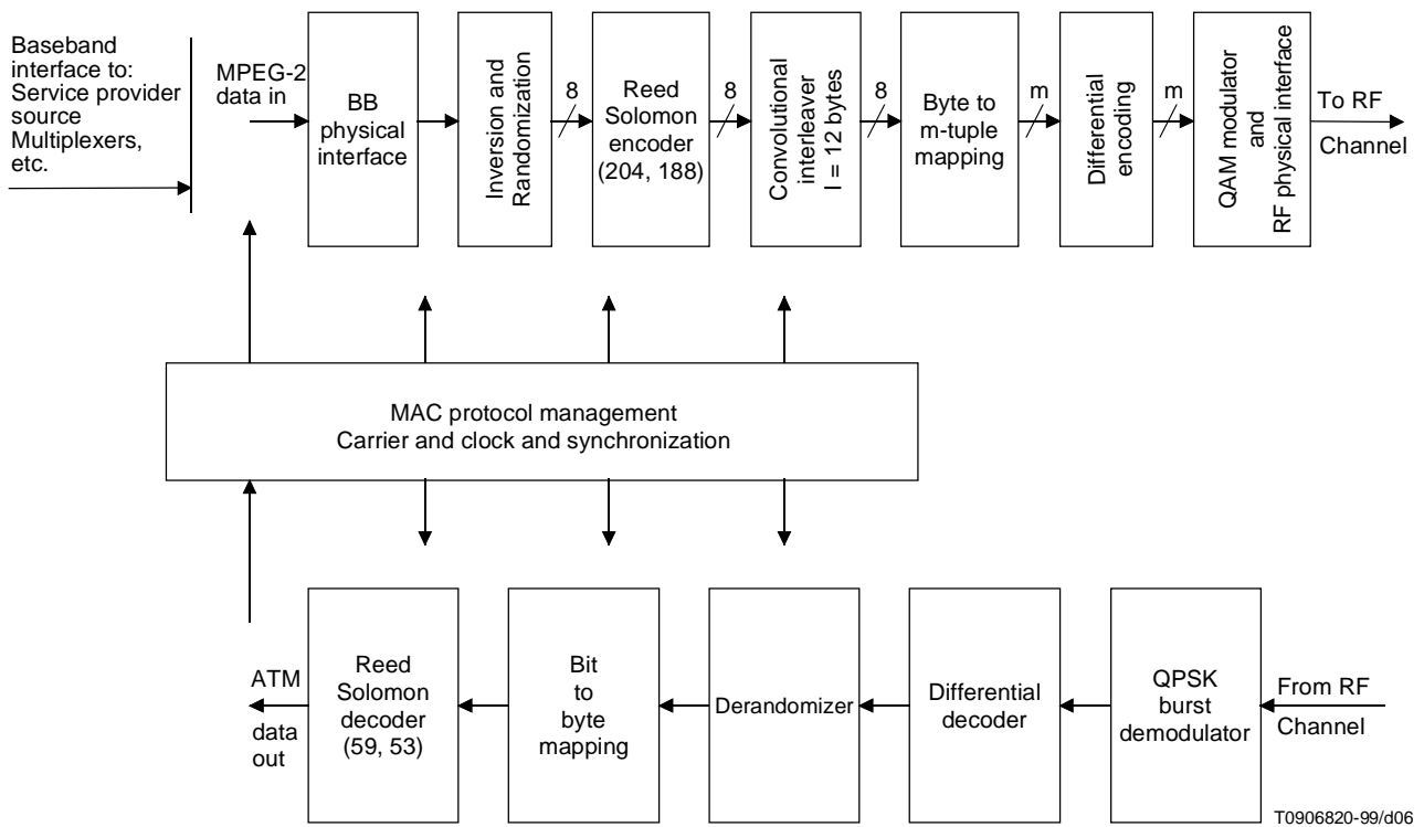
Figure 6 – Conceptual block diagram for the IB head-end transceiver
