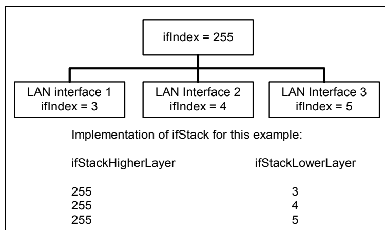
Figure 6-6 ifStack Implementation Example
