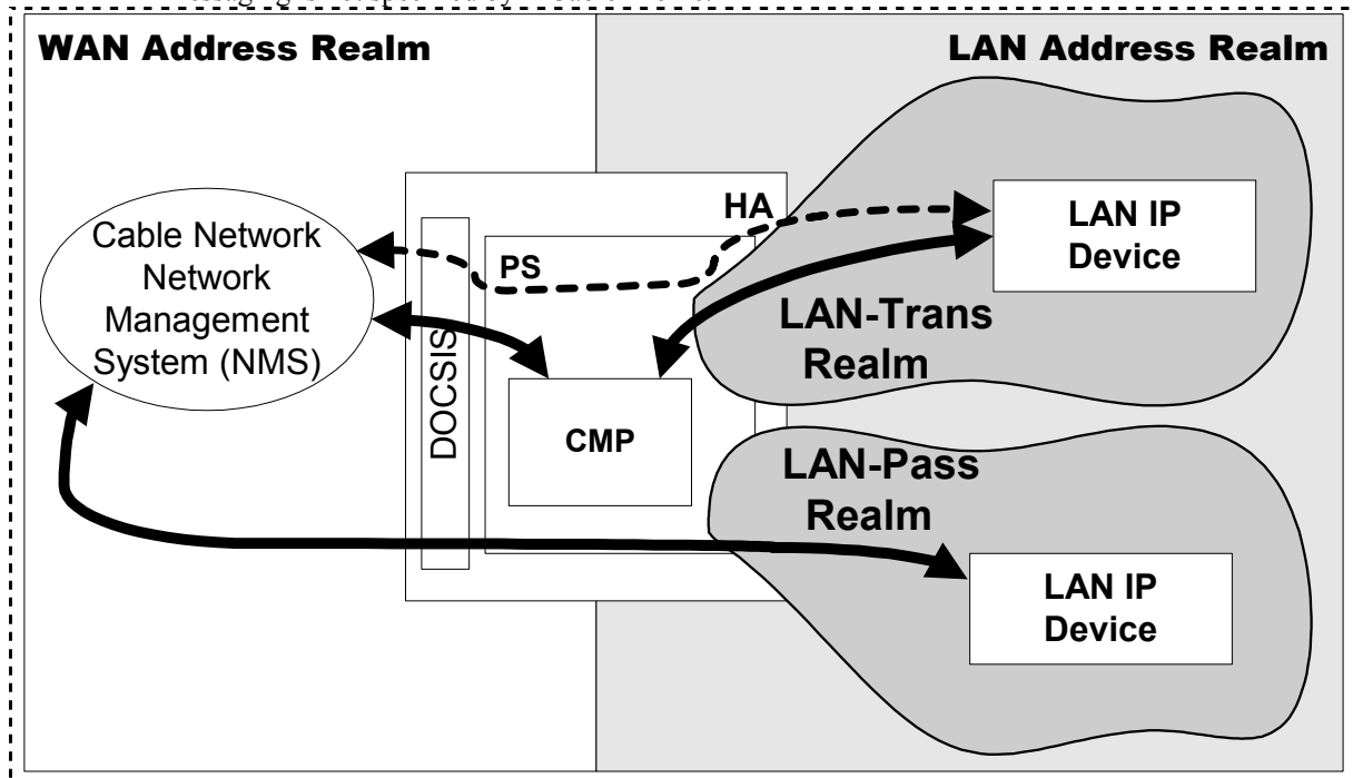
Figure 6-2 Management Message Interfaces
