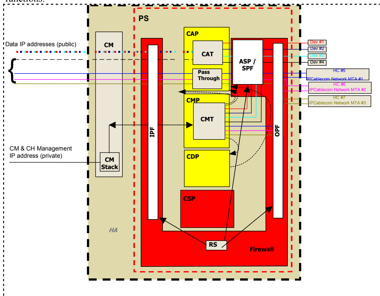
Figure 11-2 Example of a PS Element in an HA Device
