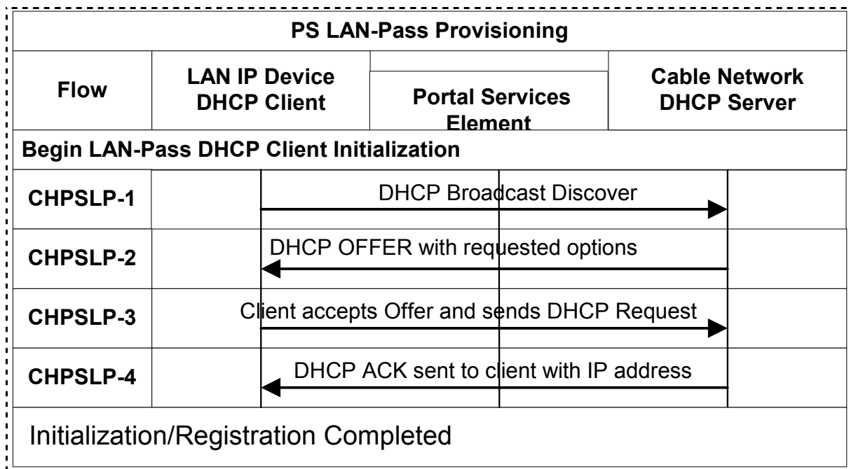
Figure 13-7 Provisioning Process for LAN IP Device in the LAN-Pass Realm
