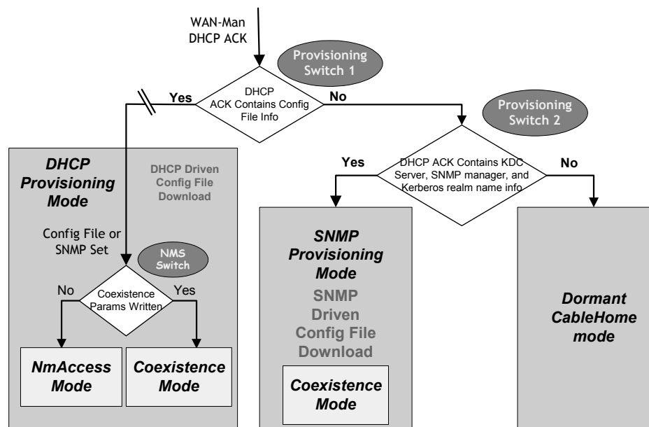
Figure 5-9 PS Operational Modes
