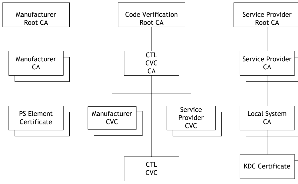
Figure 11-3 IPCable2Home Certificate Hierarchy
