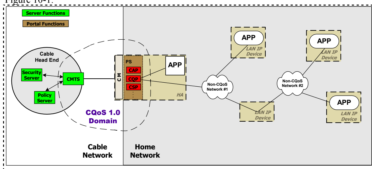
Figure 10-1 Example of CQoS Functional Elements
