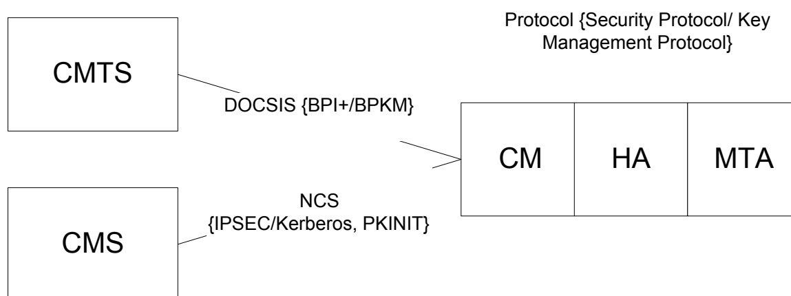
Figure 11-5 Secure CQoS Architecture to the MTA
