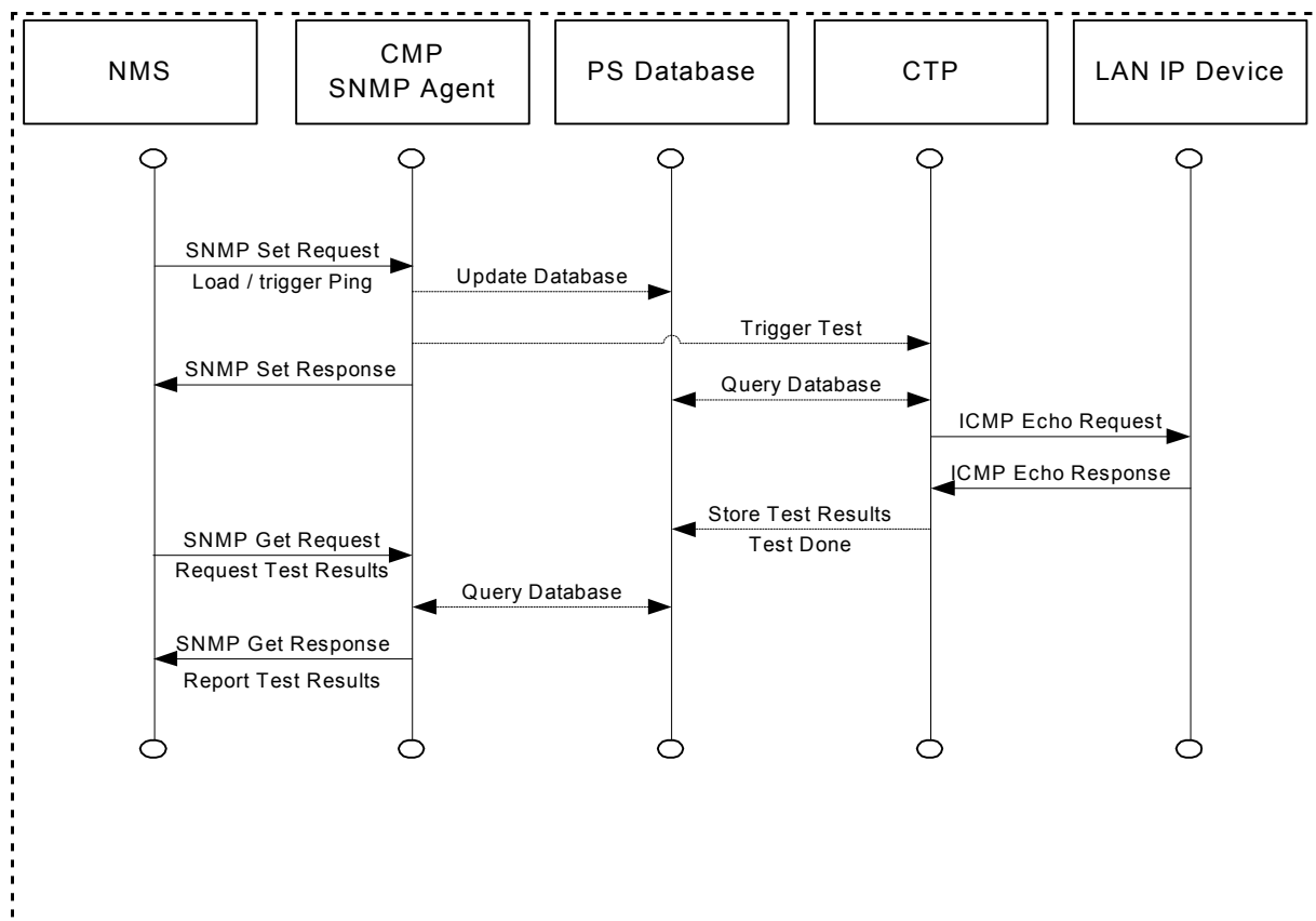
Figure 12-2 Ping Tool Process Sequence Diagram
