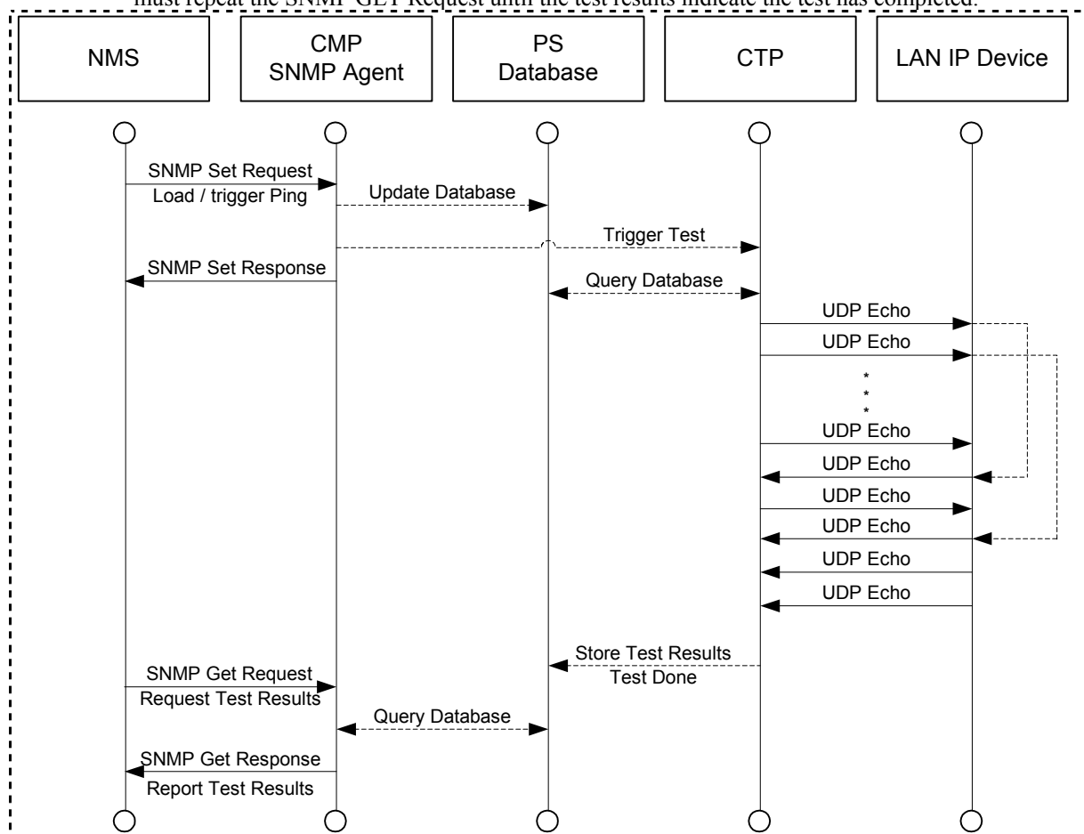
Figure 12-1 Connection Speed Tool Process Sequence Diagram
