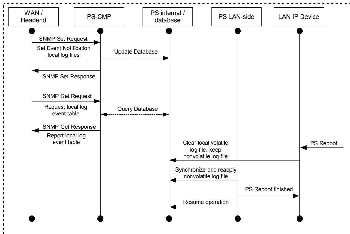
Figure 12-7 PS Configuration (Event Control) Sequence
