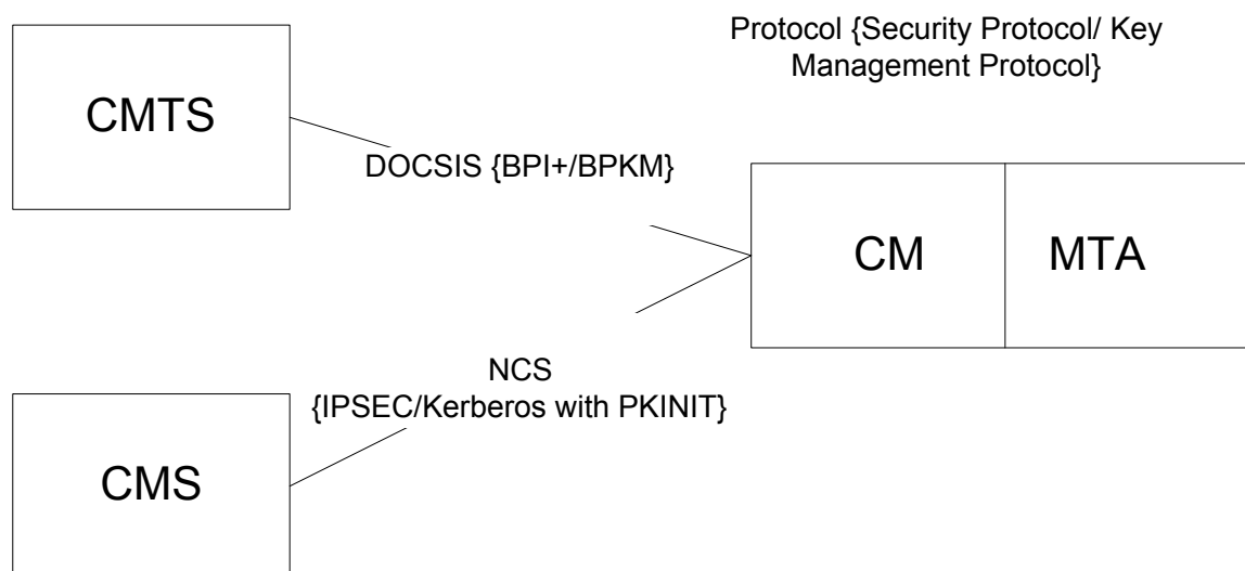
Figure 11-4 Secure DQoS Architecture to the MTA
