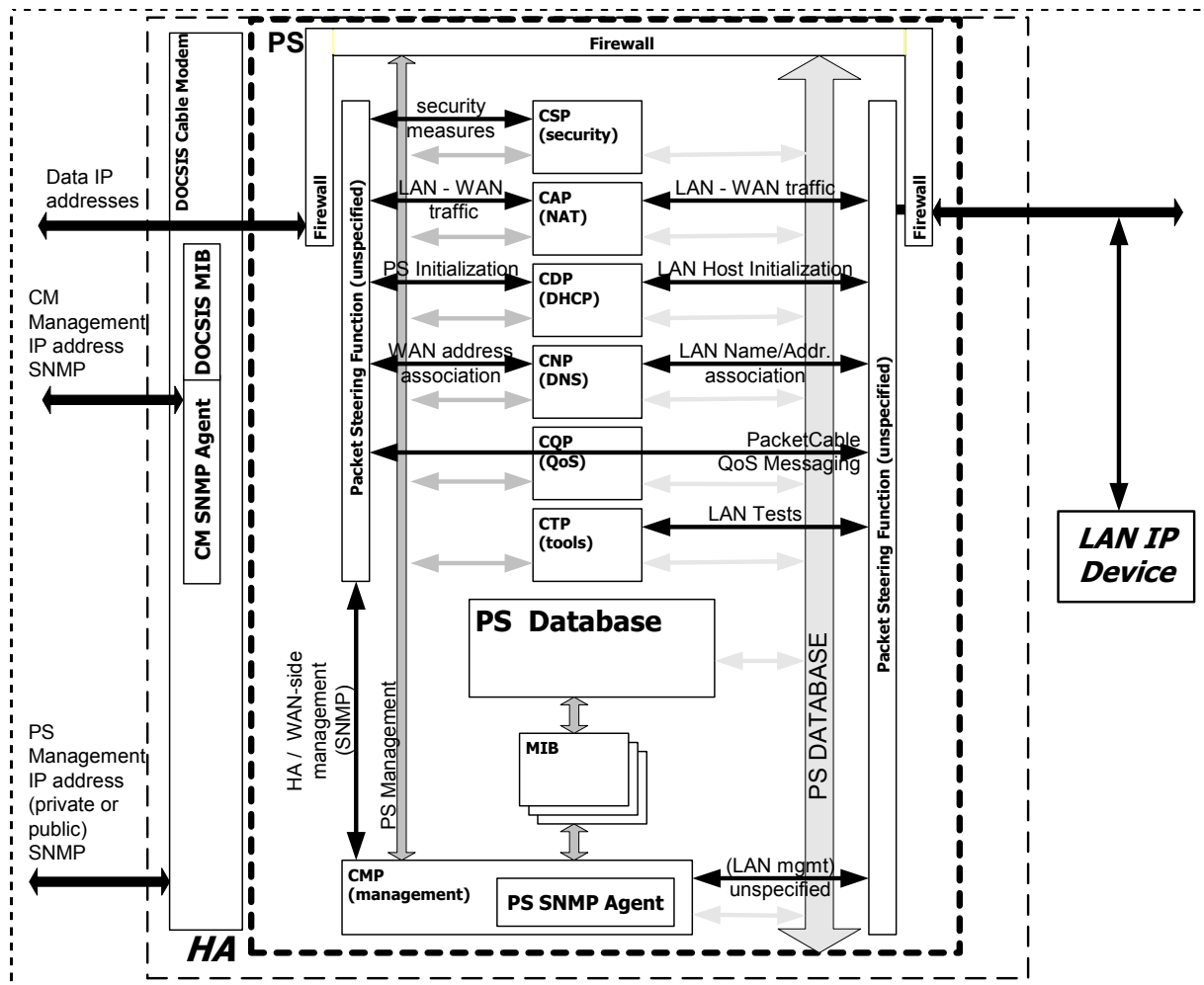
Figure 6-3 PS Block Diagram
