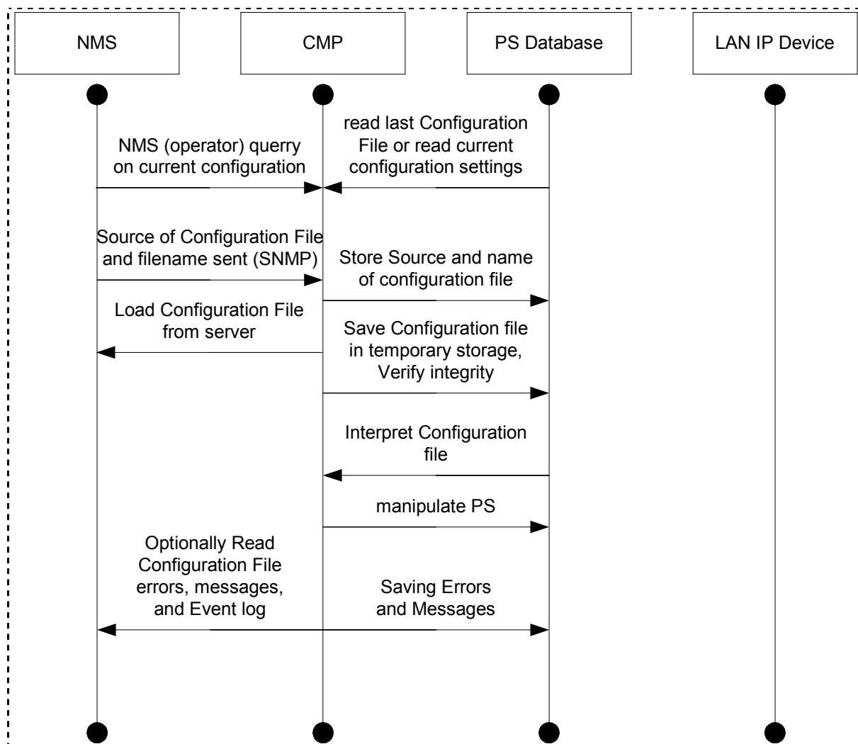
Figure 12-5 PS Reconfiguration (Configuration File Download) Sequence Diagram
