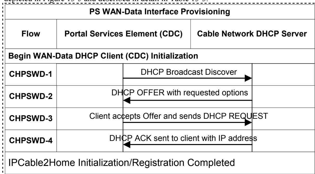
Figure 13-5 PS WAN-Data Provisioning Process
