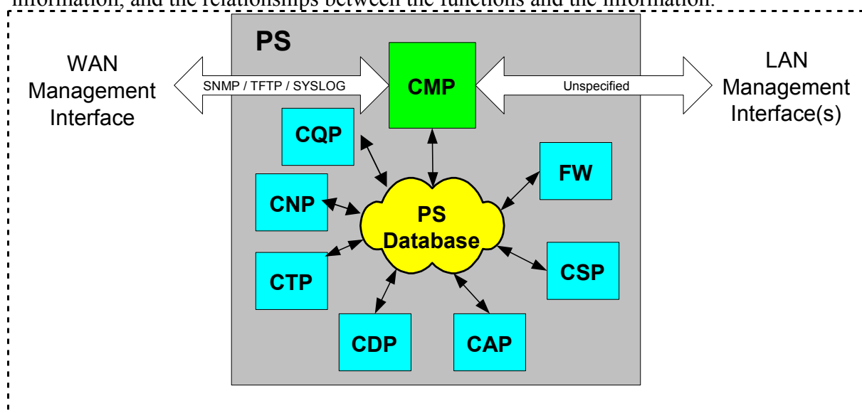
Figure 5-7 PS Function and Database Relationship
