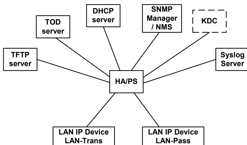
Figure 13-1 Provisioning Functional Elements
