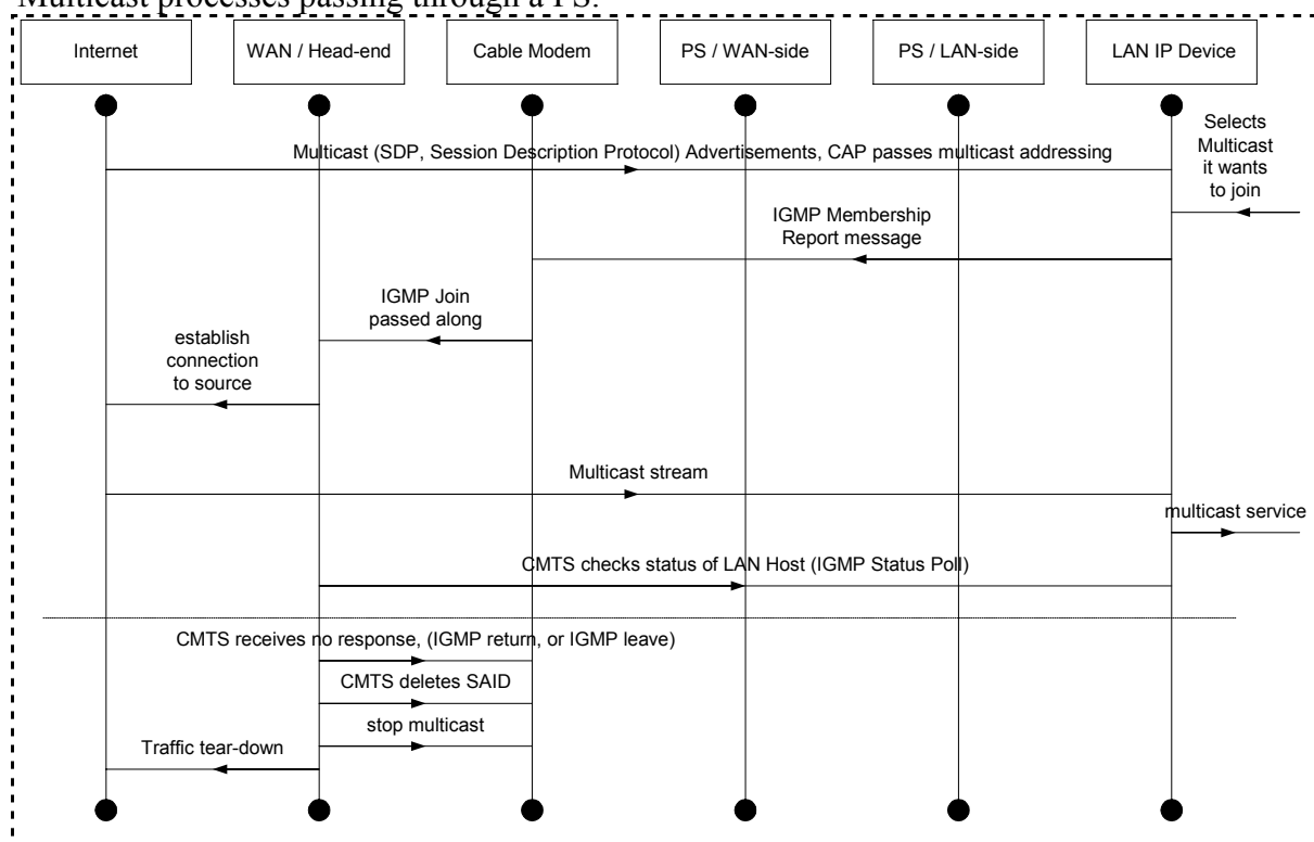
Figure 8-3 Multicast via IGMP Sequence
