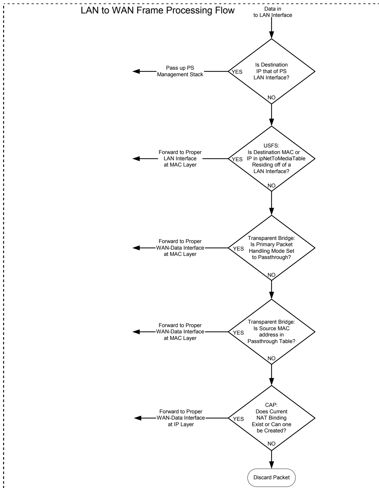
Figure 8-4 LAN-to-WAN Packet Processing Example
