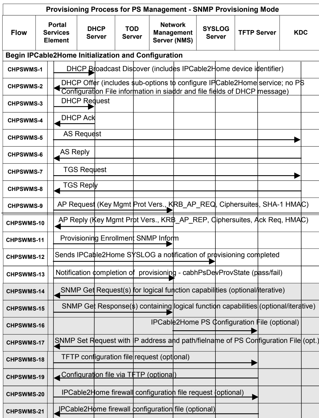
Figure 13-4 Provisioning Process for PS Management - SNMP Provisioning Mode
