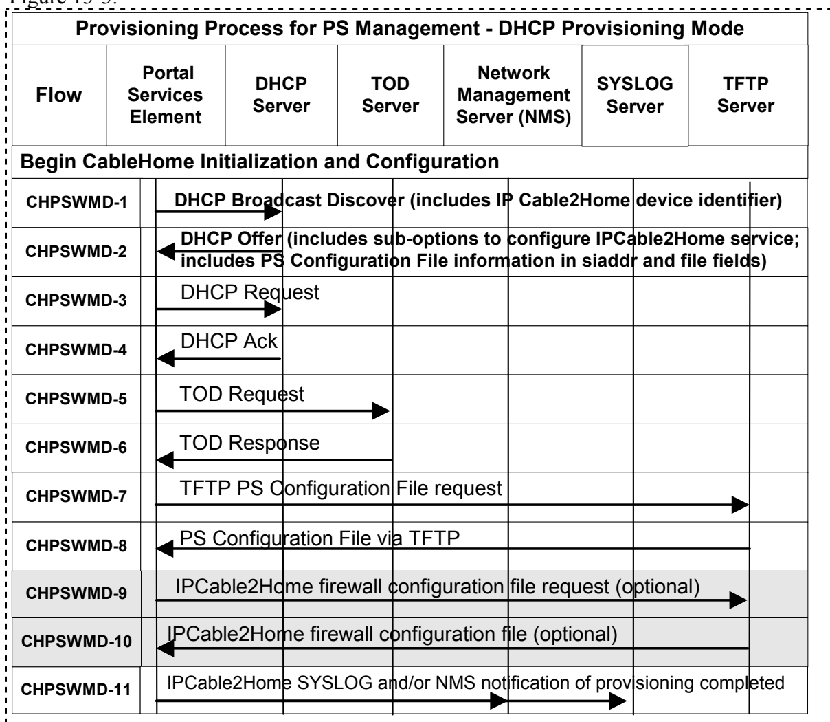
Figure 13-3 Provisioning Process for PS Management - DHCP Provisioning Mode
