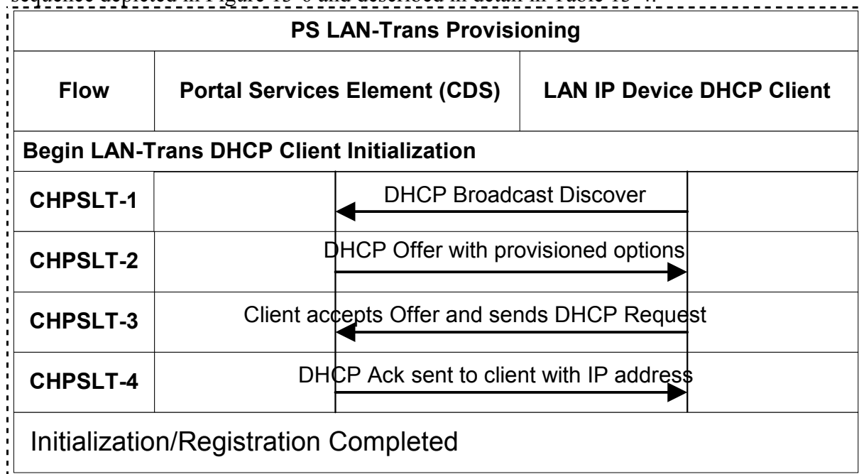
Figure 13-6 Provisioning Process for LAN IP Device in LAN-Trans Realm
