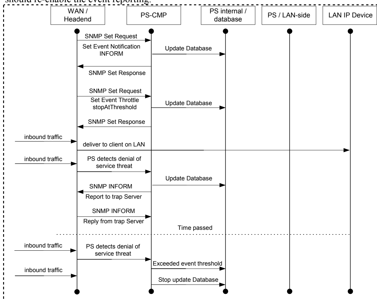
Figure 12-10 CMP Event Throttling and Limiting Operation
