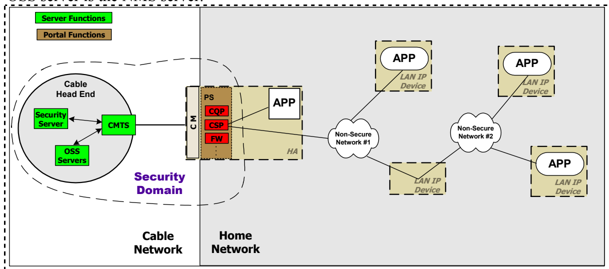
Figure 11-1 IPCable2Home Security Elements
