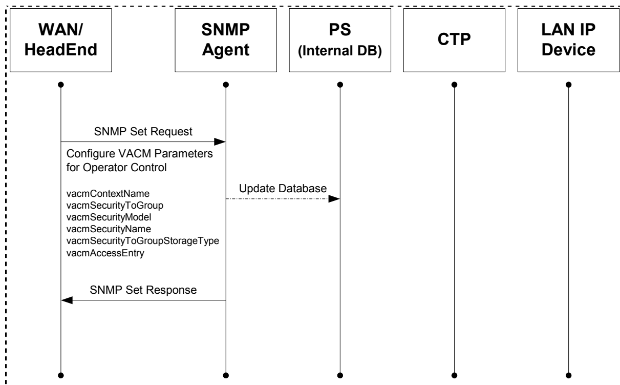
Figure 12-6 PS Configuration (VACM Parameters) Sequence
