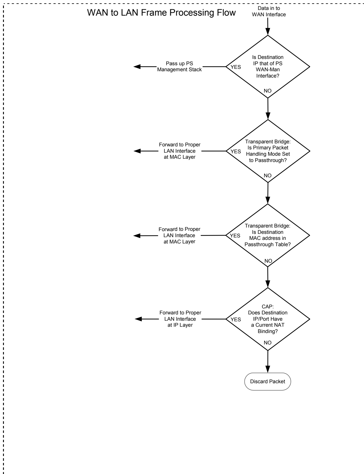
Figure 8-5 WAN-to-LAN Packet Processing Example
