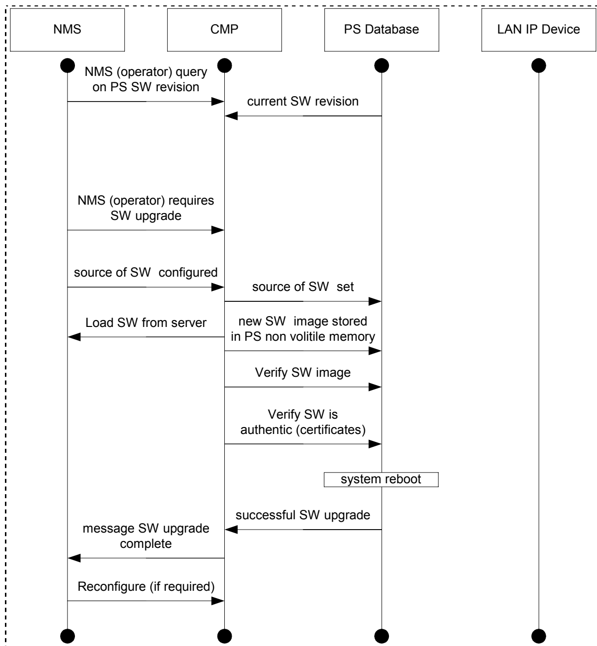
Figure 12-4 PS Software Download Sequence Diagram
