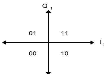
FIGURE 6-1. QPSK symbol mapping
