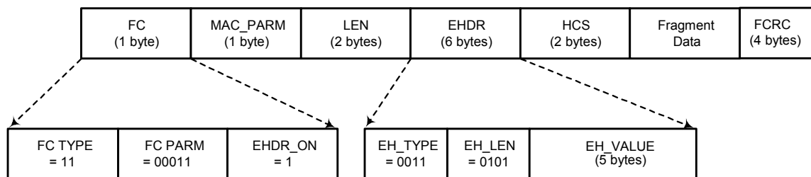
FIGURE 8-9. Fragmentation MAC Header format
