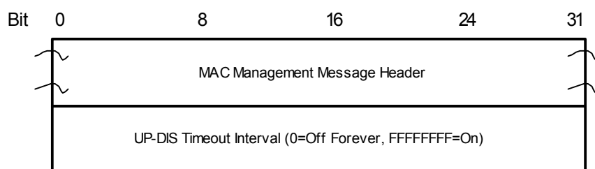
FIGURE 8-44. UP-DIS message format
