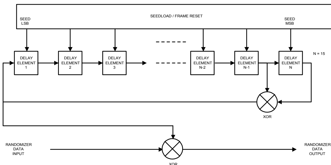
FIGURE 6-4. Scrambler structure
