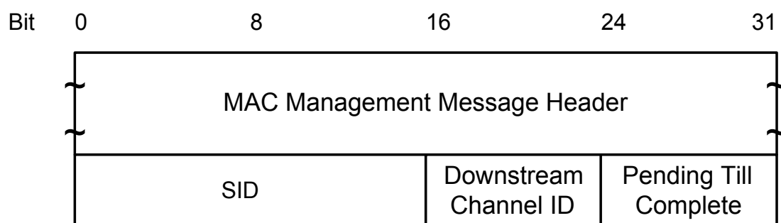
FIGURE 8-21. Packet PDU Following the Timing Header
