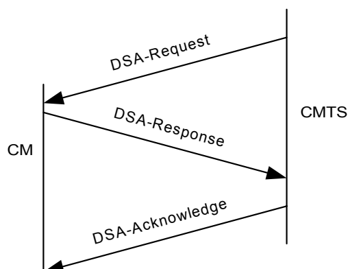
FIGURE 10-7. Dynamic Service Addition Message Flow - CMTS Initiated
