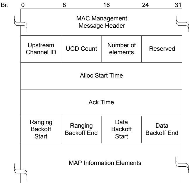
FIGURE 8-19. MAP Format
