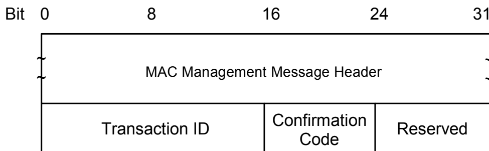
FIGURE 8-38. Dynamic Service Deletion - Response
