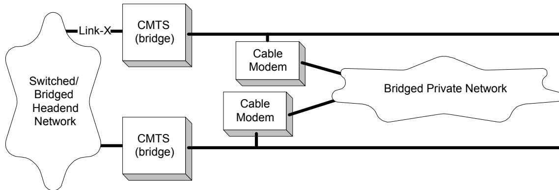
FIGURE I-2. Spanning Tree Across CMTSs
