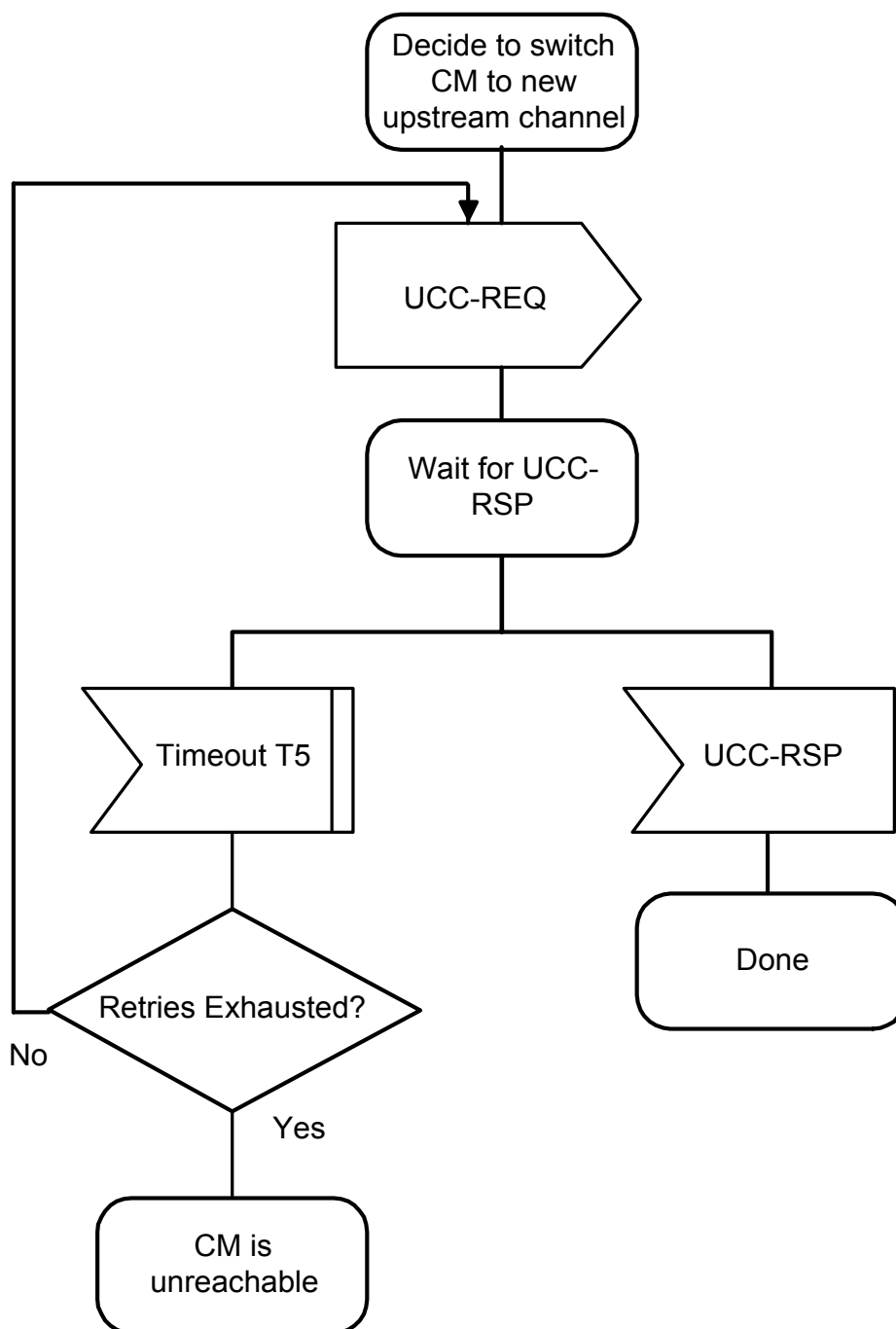
FIGURE 11-18. Changing Upstream Channels: CMTS View
