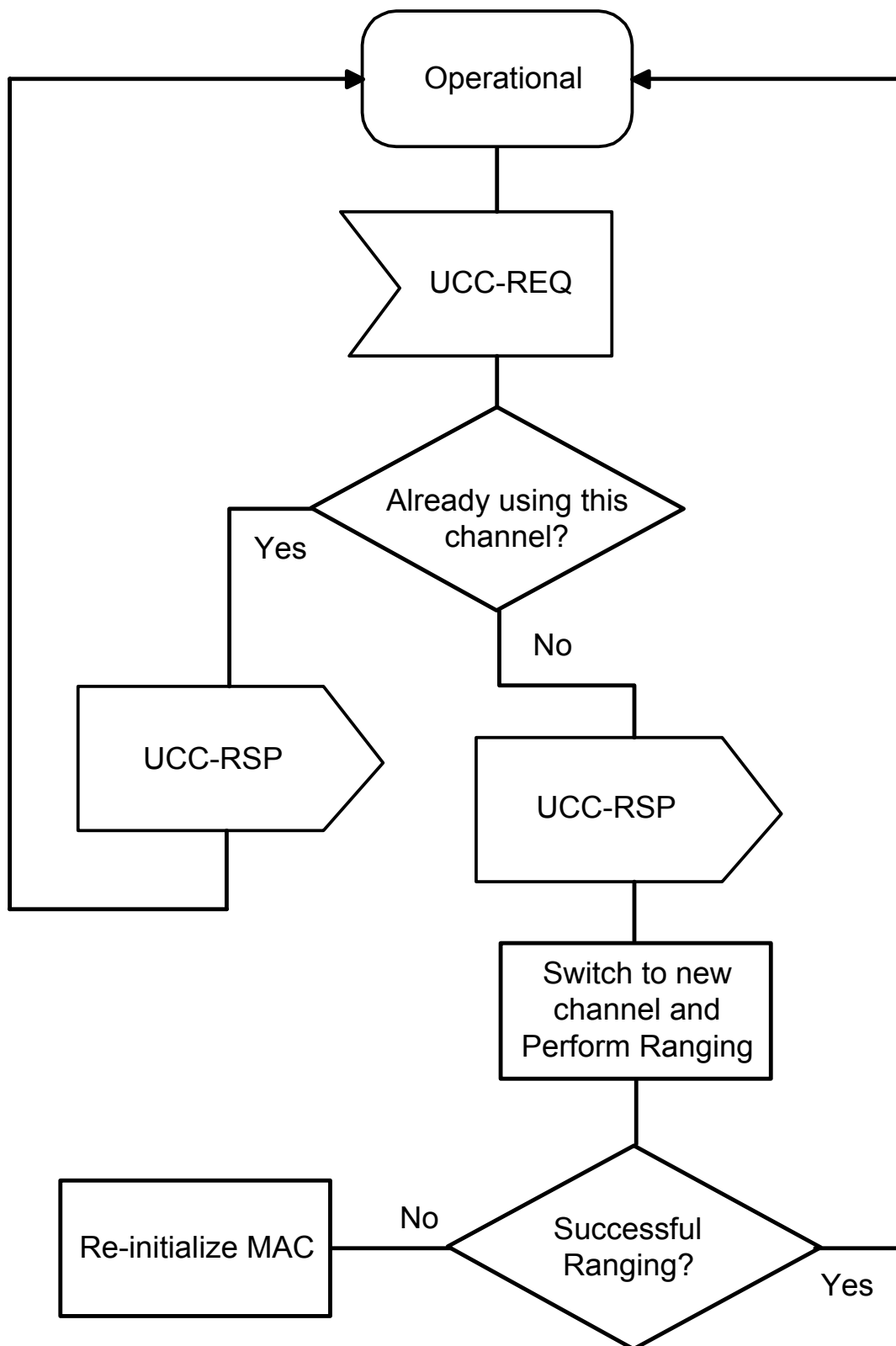
FIGURE 11-19. Changing Upstream Channels: CM View
