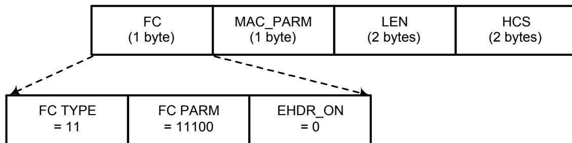
FIGURE 8-11. Concatenation MAC Header Format
