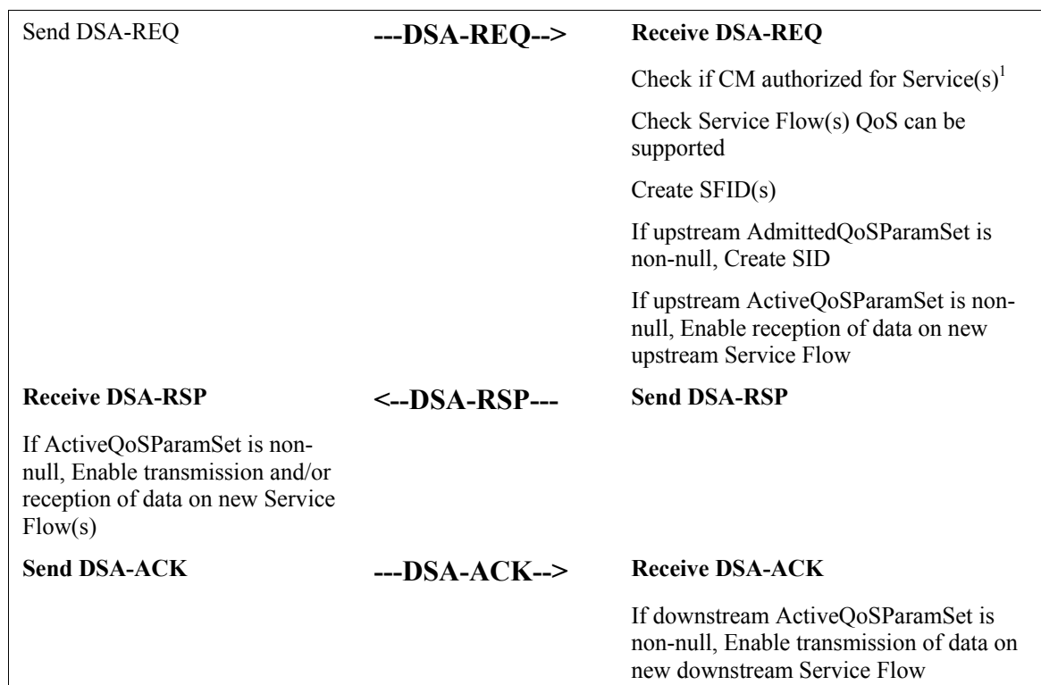
FIGURE 11-28. Dynamic Service Addition Initiated from CM
