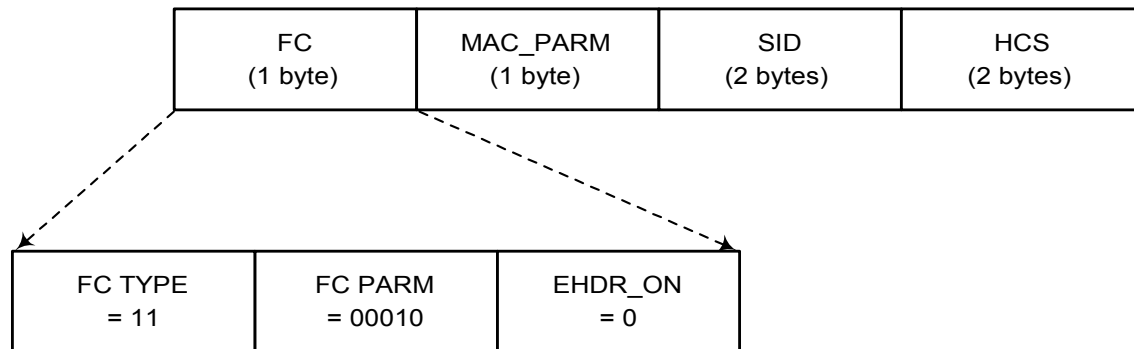
FIGURE 8-8. Request Frame format
