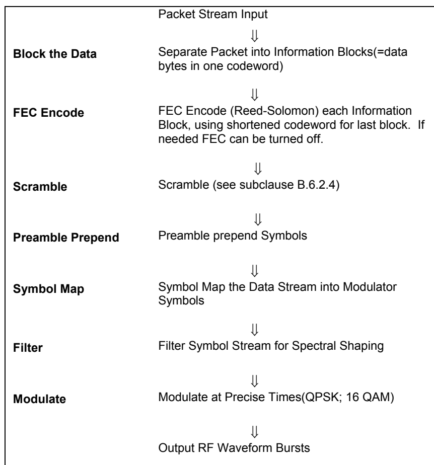
FIGURE 6-10. TDMA upstream transmission processing
