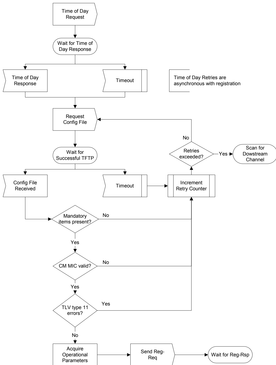
FIGURE 11-12. Registration - CM
