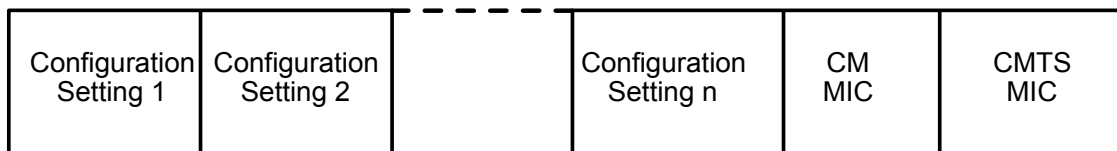
FIGURE D-1. Binary Configuration File Format
