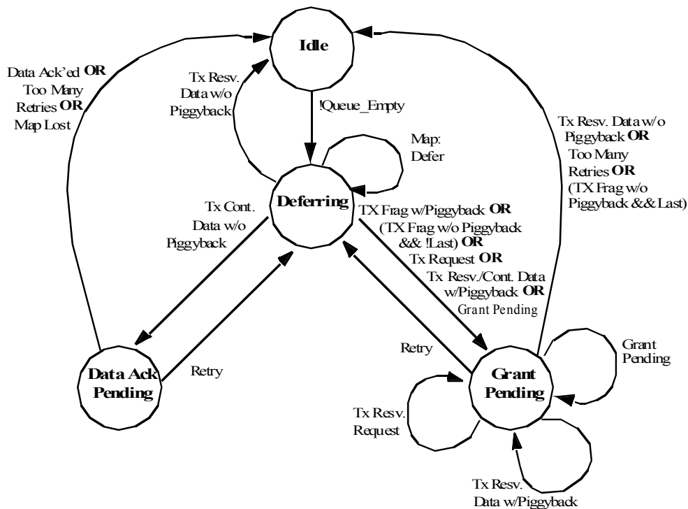
FIGURE K-1. Transmission & Deference State Transition Diagram
