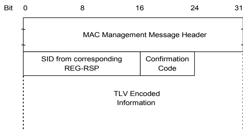
FIGURE 8-28. Registration Acknowledgment
