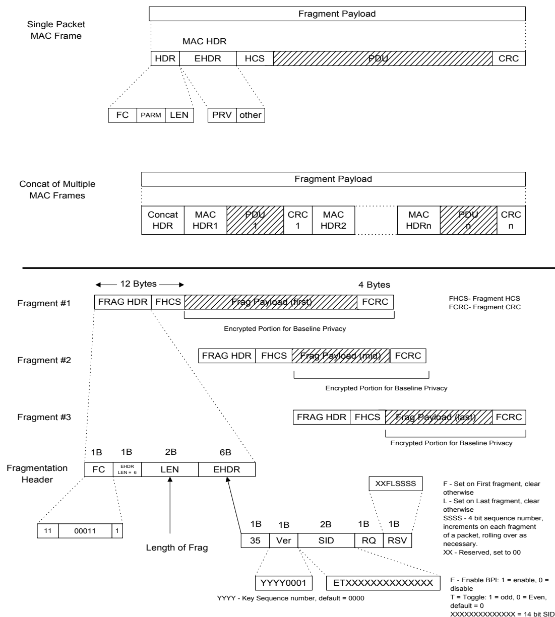
FIGURE 8-13. Fragmentation Details
