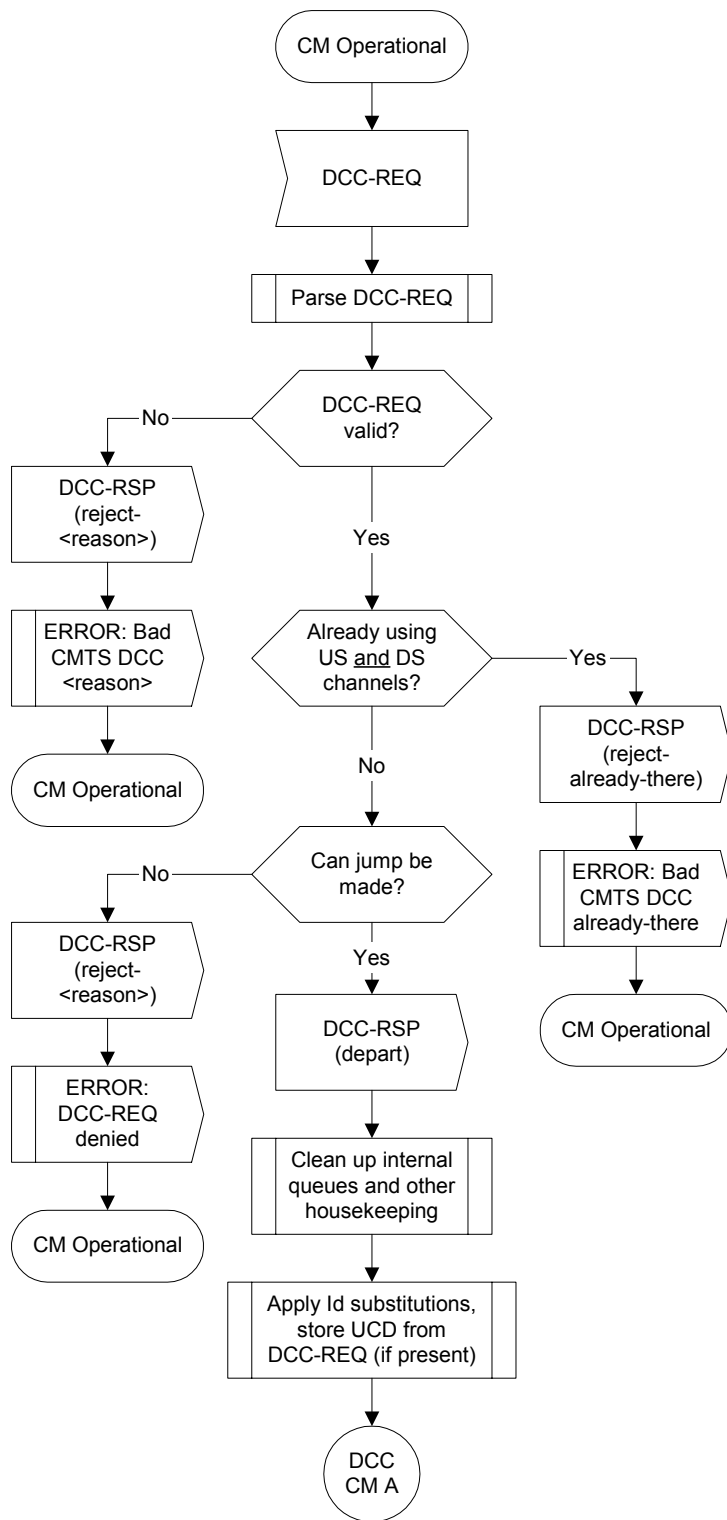
FIGURE 11-62. Dynamically Changing Channels: CM View Part 1 5
