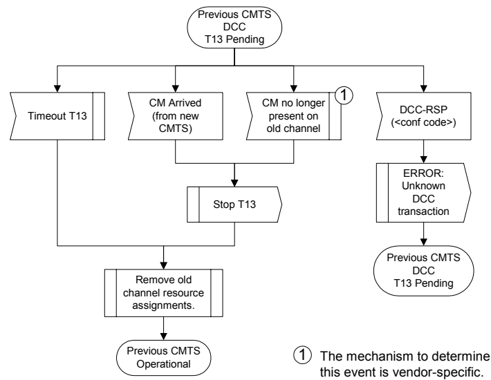
FIGURE 11-60. Dynamically Changing Channels: CMTS View Part 3
