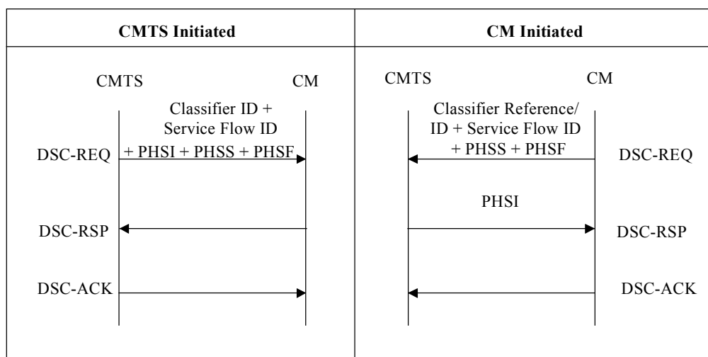
FIGURE 10-13. Payload Header Suppression Signalling Example
