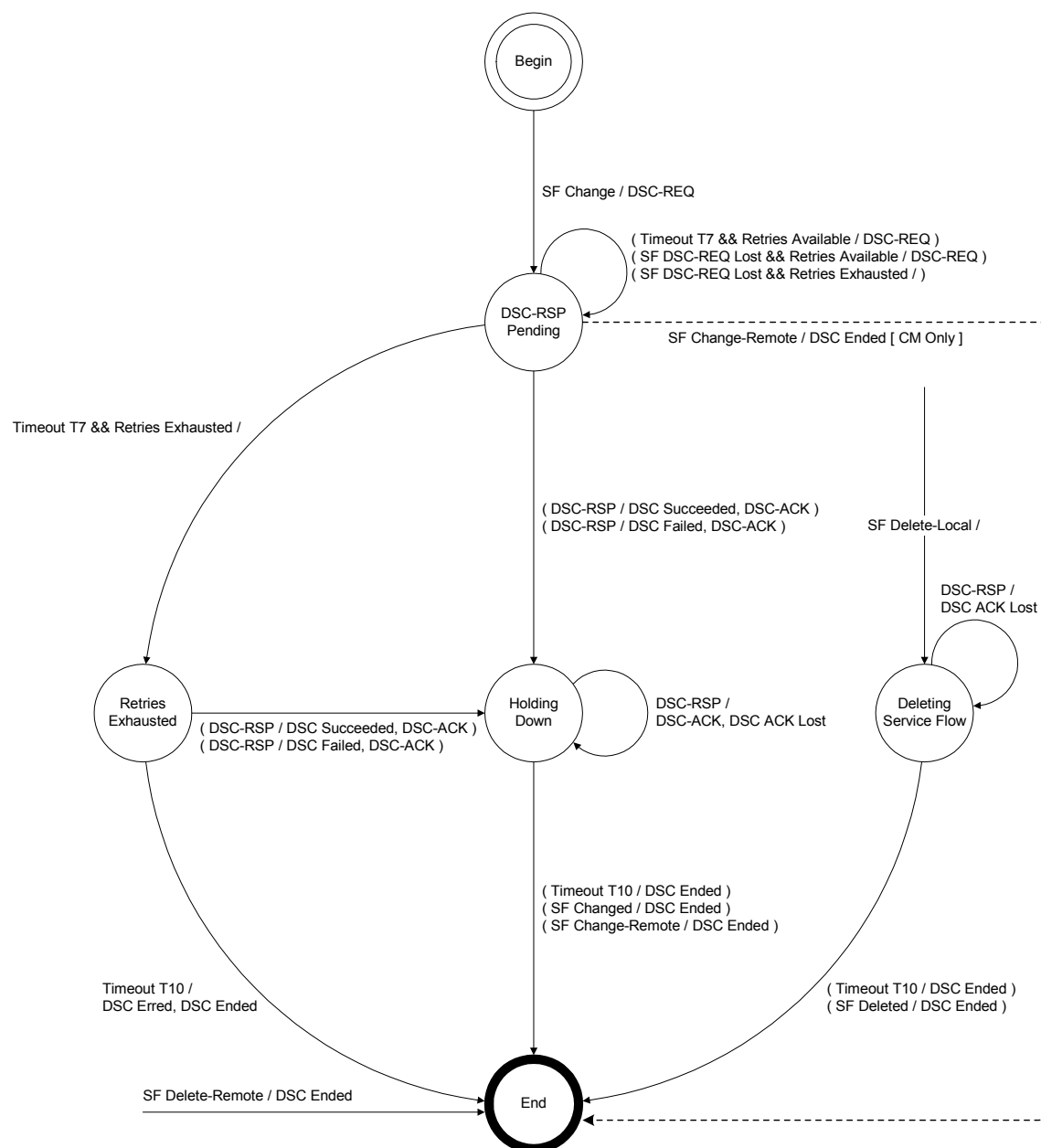
FIGURE 11-24. DSC—Locally Initiated Transaction State Transition Diagram
