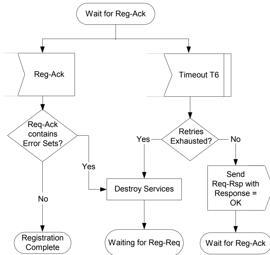
FIGURE 11-15. Registration Acknowledgment- CMTS
