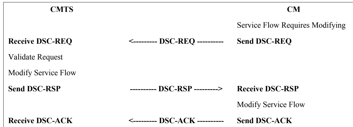
FIGURE 11-39. CM-Initiated DSC
