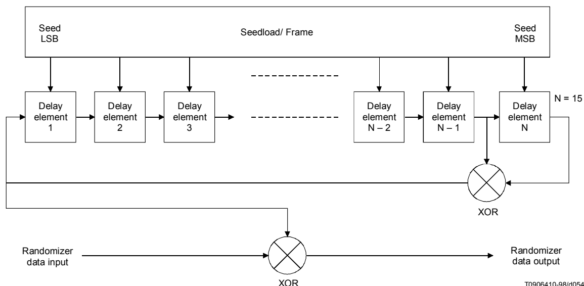
FIGURE N-4. Scrambler structure
