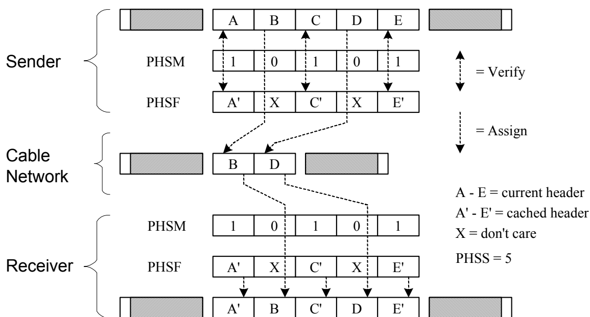
FIGURE 10-12. Payload Header Suppression with Masking
