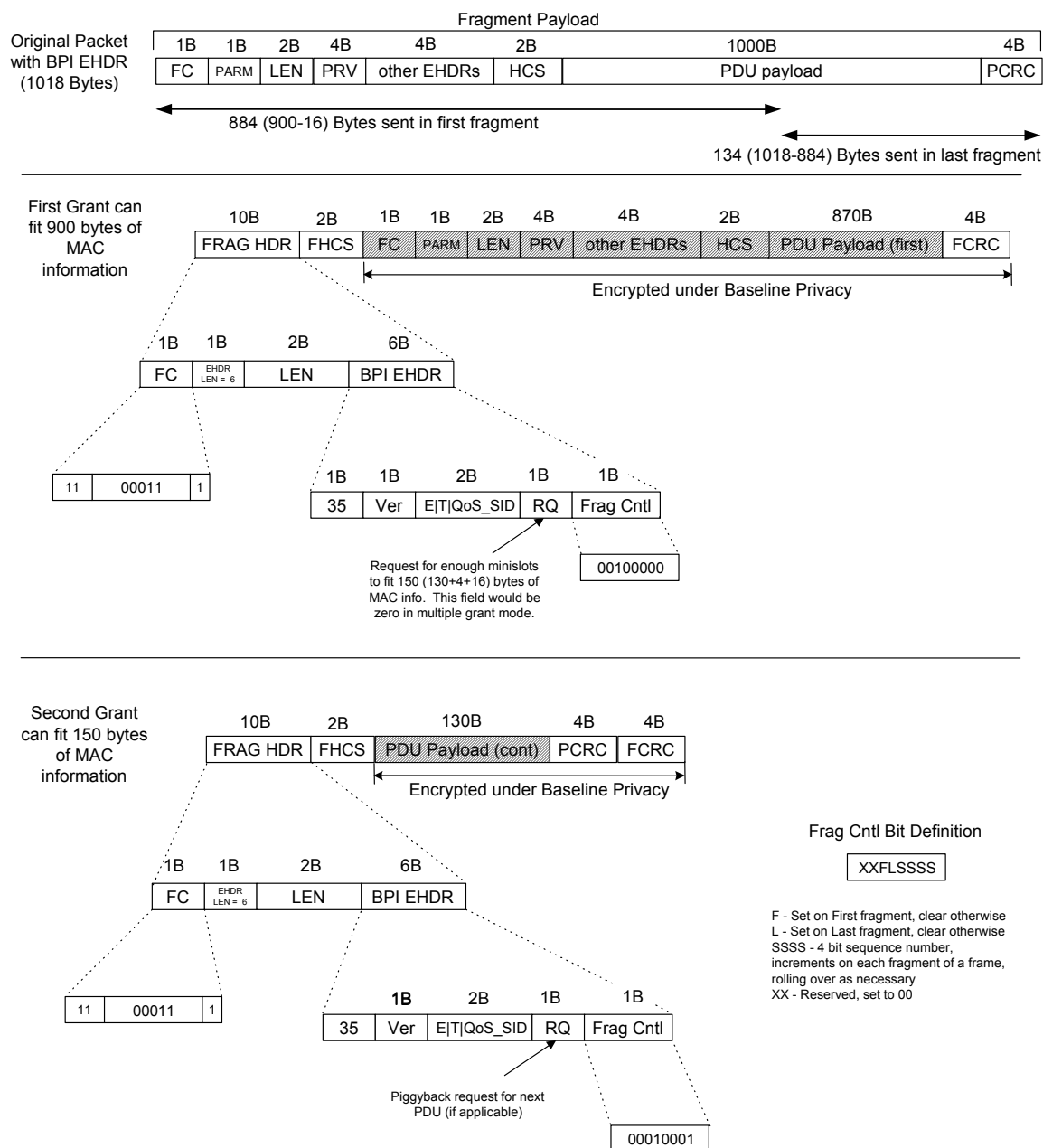
FIGURE 10-9. Example of Fragmenting a Single Packet
