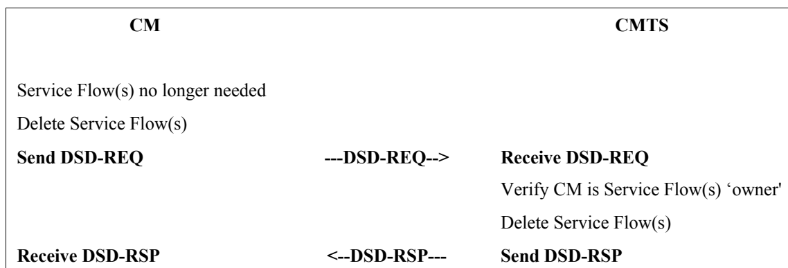
FIGURE 11-50. Dynamic Service Deletion Initiated from CM
