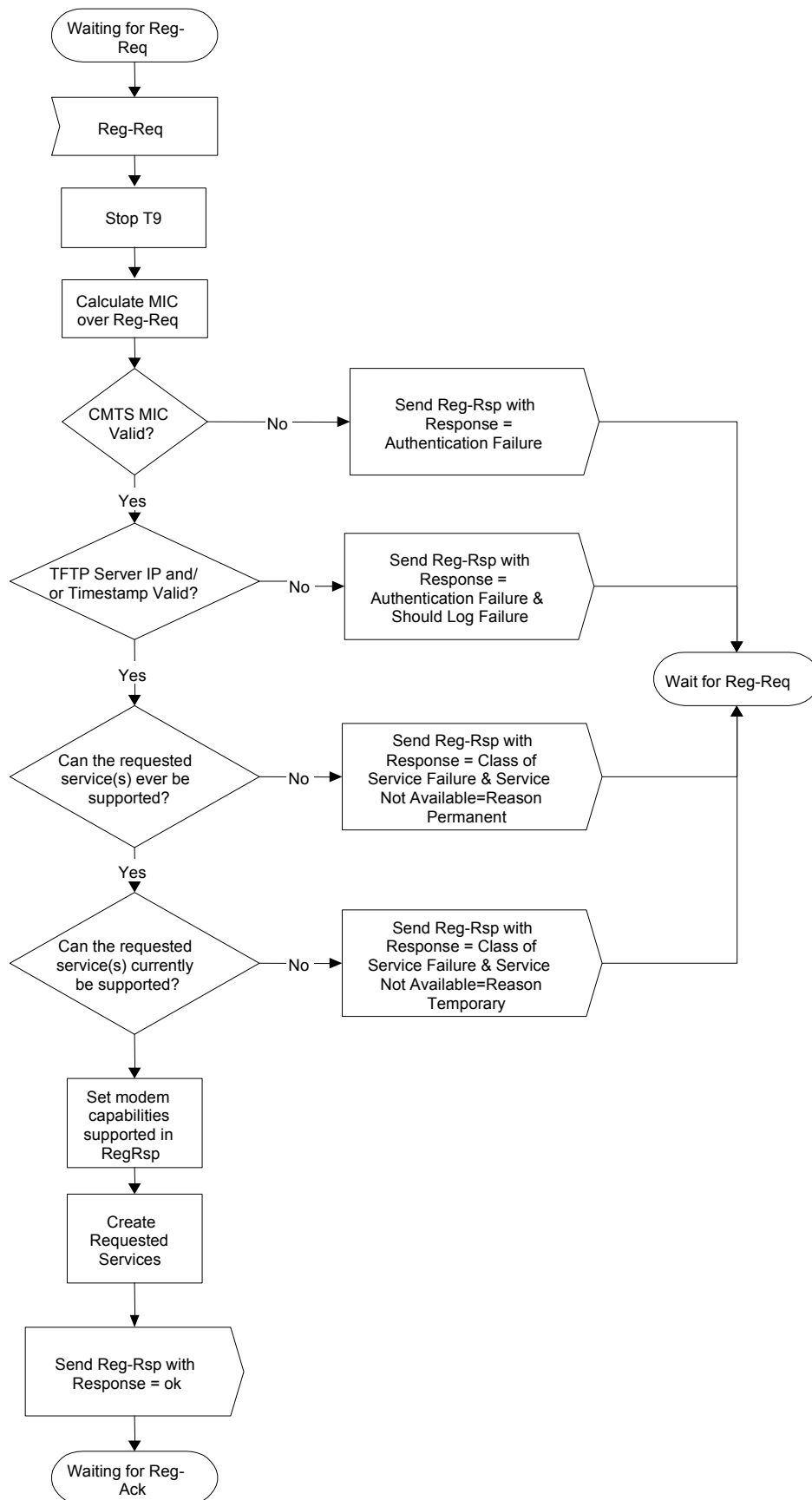
FIGURE 11-14. Registration - CMTS
