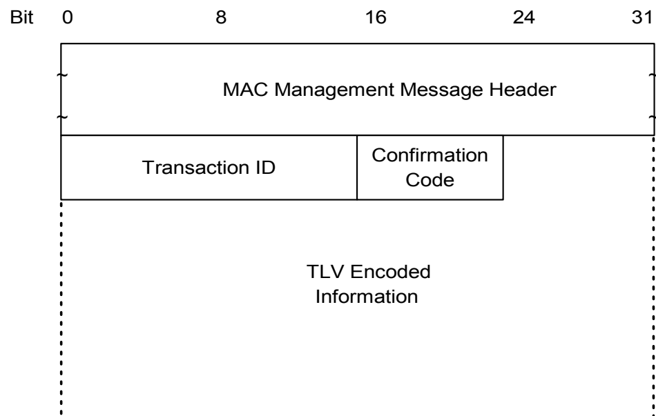
FIGURE 8-33. Dynamic Service Addition - Acknowledge
