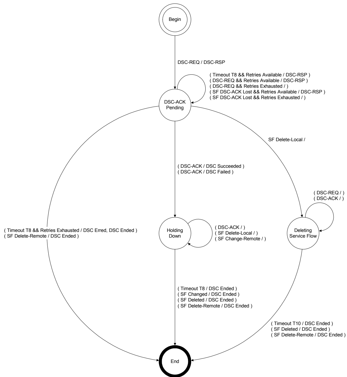
FIGURE 11-25. DSC—Remotely Initiated Transaction State Transition Diagram
