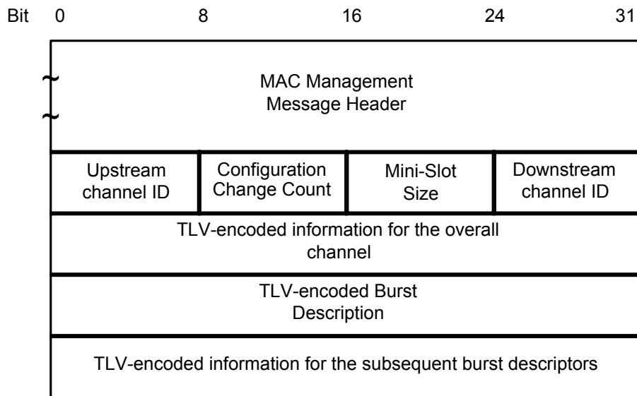
FIGURE 8-16. Upstream Channel Descriptor
