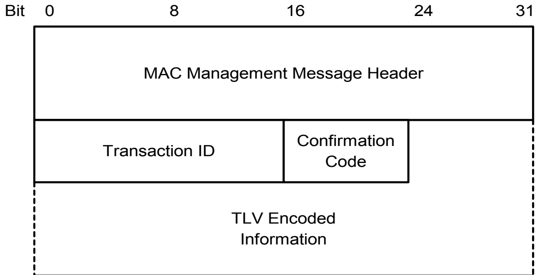
FIGURE 8-40. Dynamic Channel Change Response
