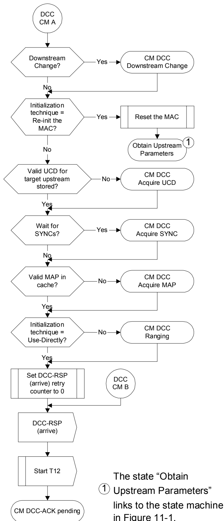
FIGURE 11-63. Dynamically Changing Channels: CM View Part 2
