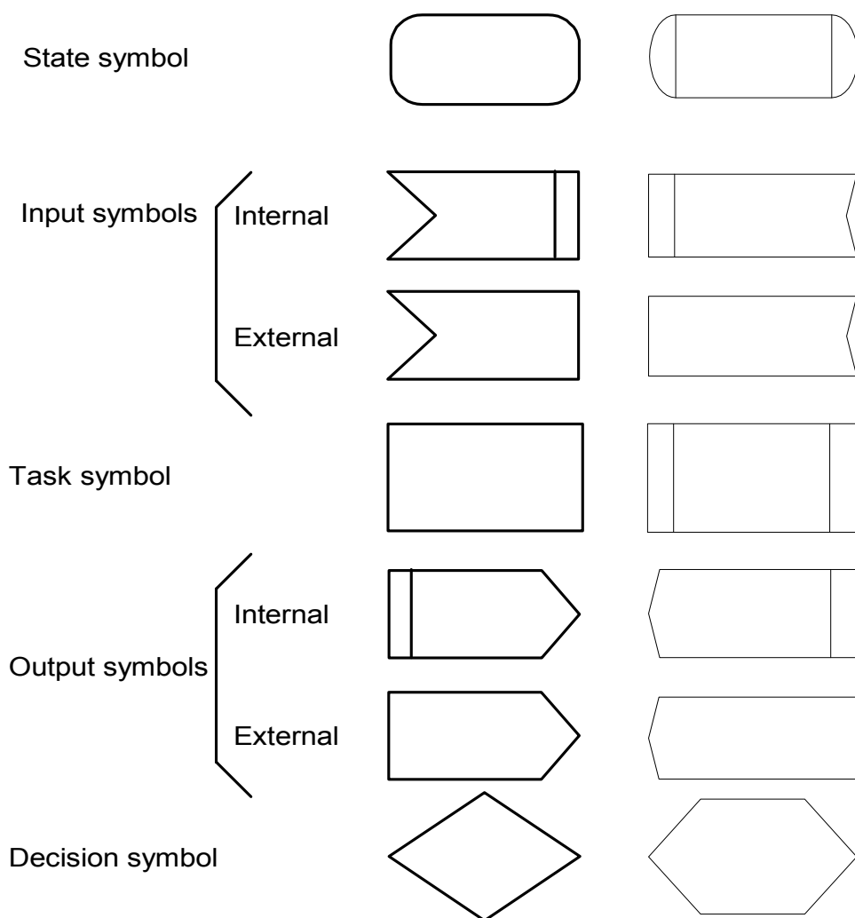
FIGURE 11-2. SDL Notation
