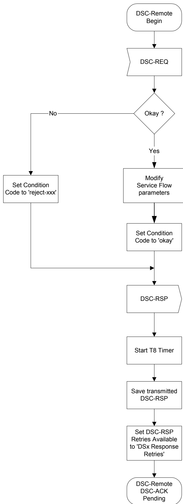
FIGURE 11-46. DSC—Remotely Initiated Transaction Begin State Flow Diagram
