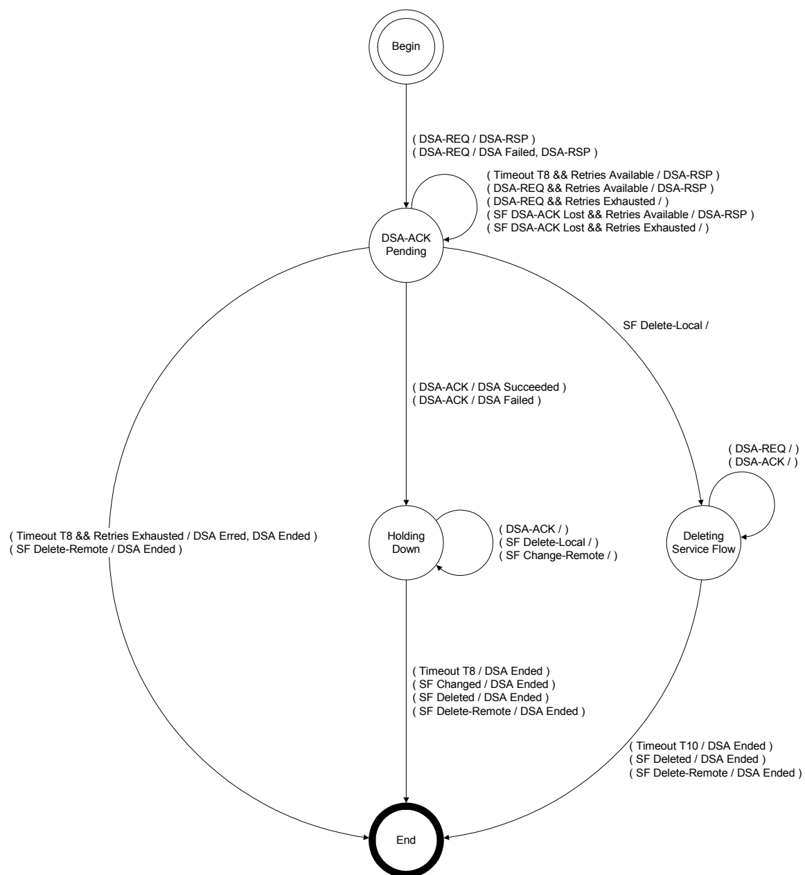
FIGURE 11-23. DSA—Remotely Initiated Transaction State Transition Diagram
