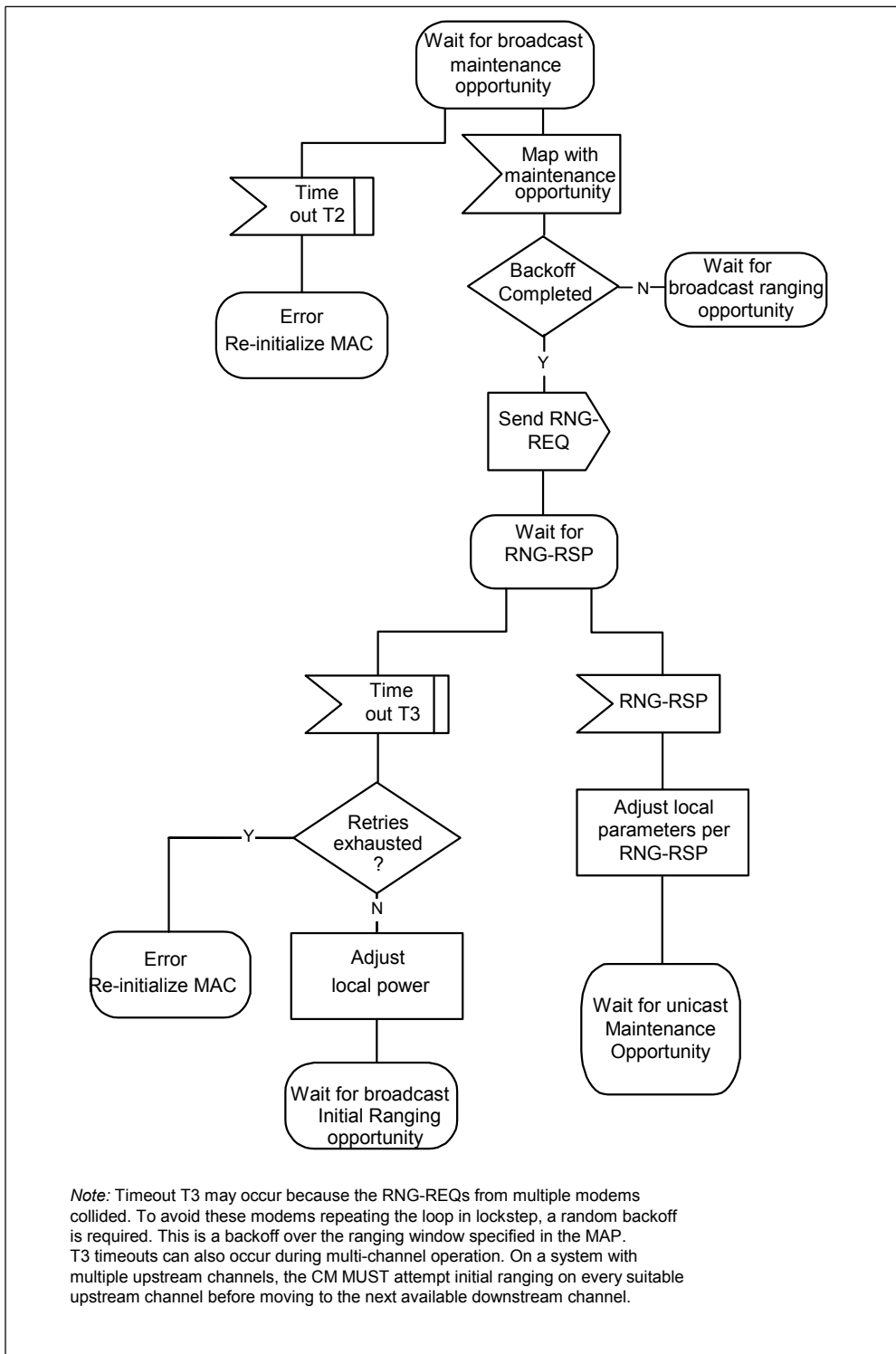
FIGURE 11-6. Initial Ranging - CM
