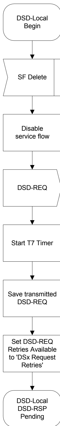
FIGURE 11-52. DSD—Locally Initiated Transaction Begin State Flow Diagram
