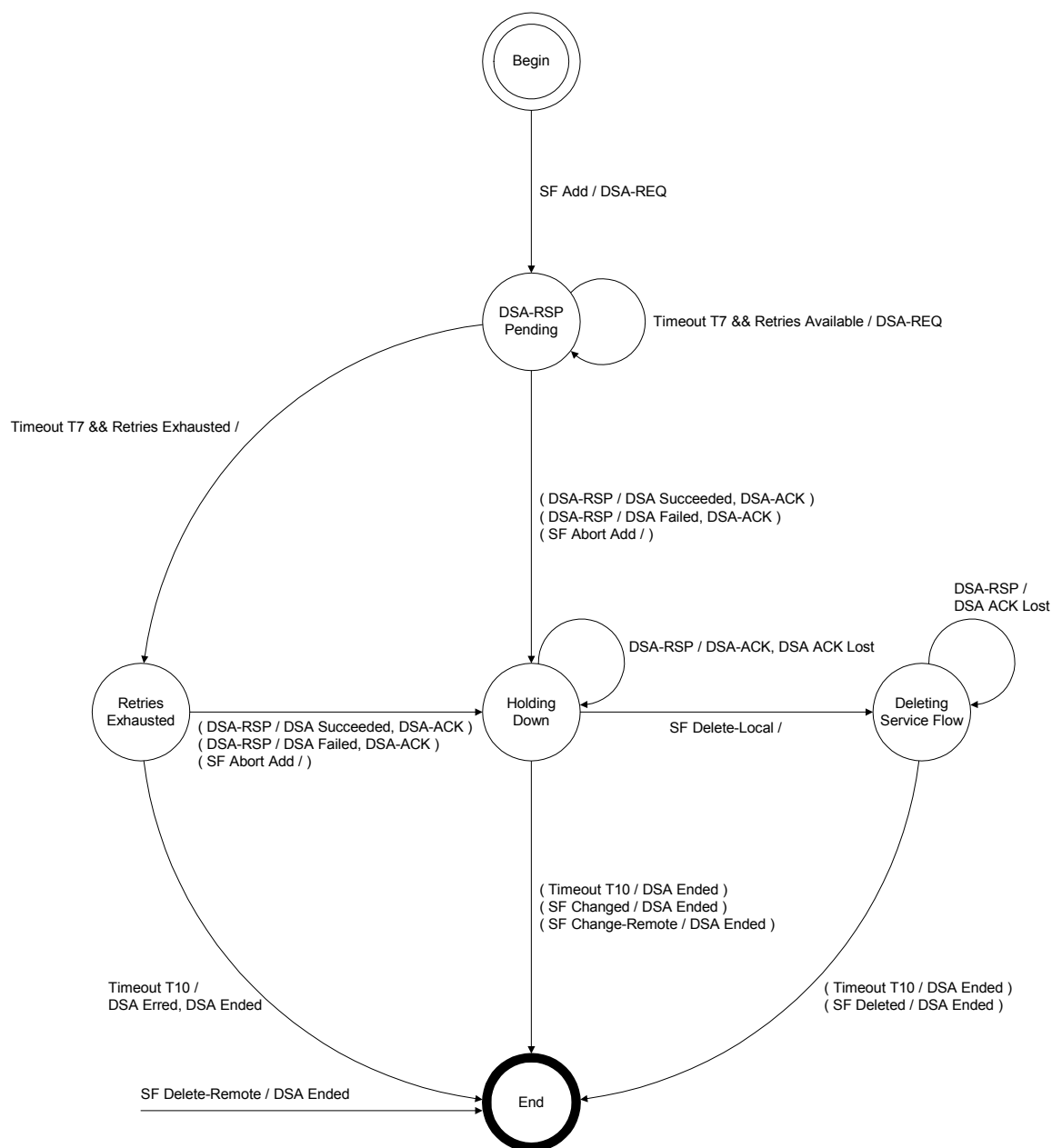
FIGURE 11-22. DSA—Locally Initiated Transaction State Transition Diagram
