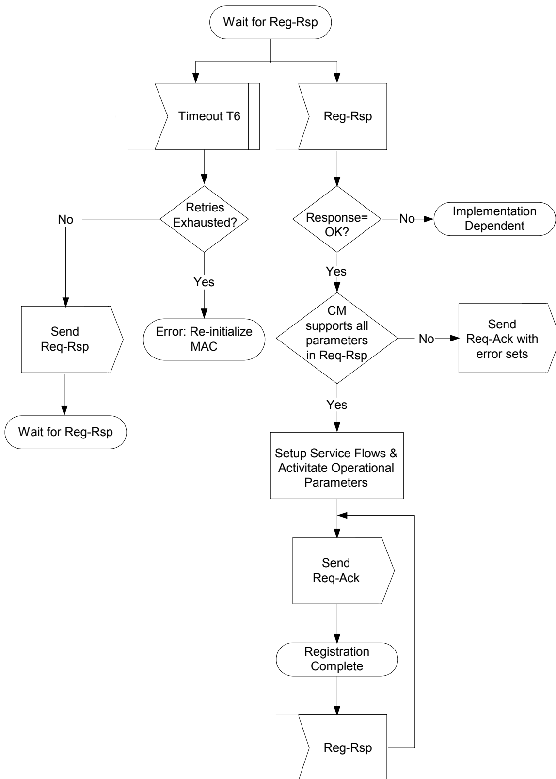
FIGURE 11-13. Wait for Registration Response - CM
