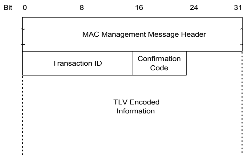
FIGURE 8-32. Dynamic Service Addition - Response
