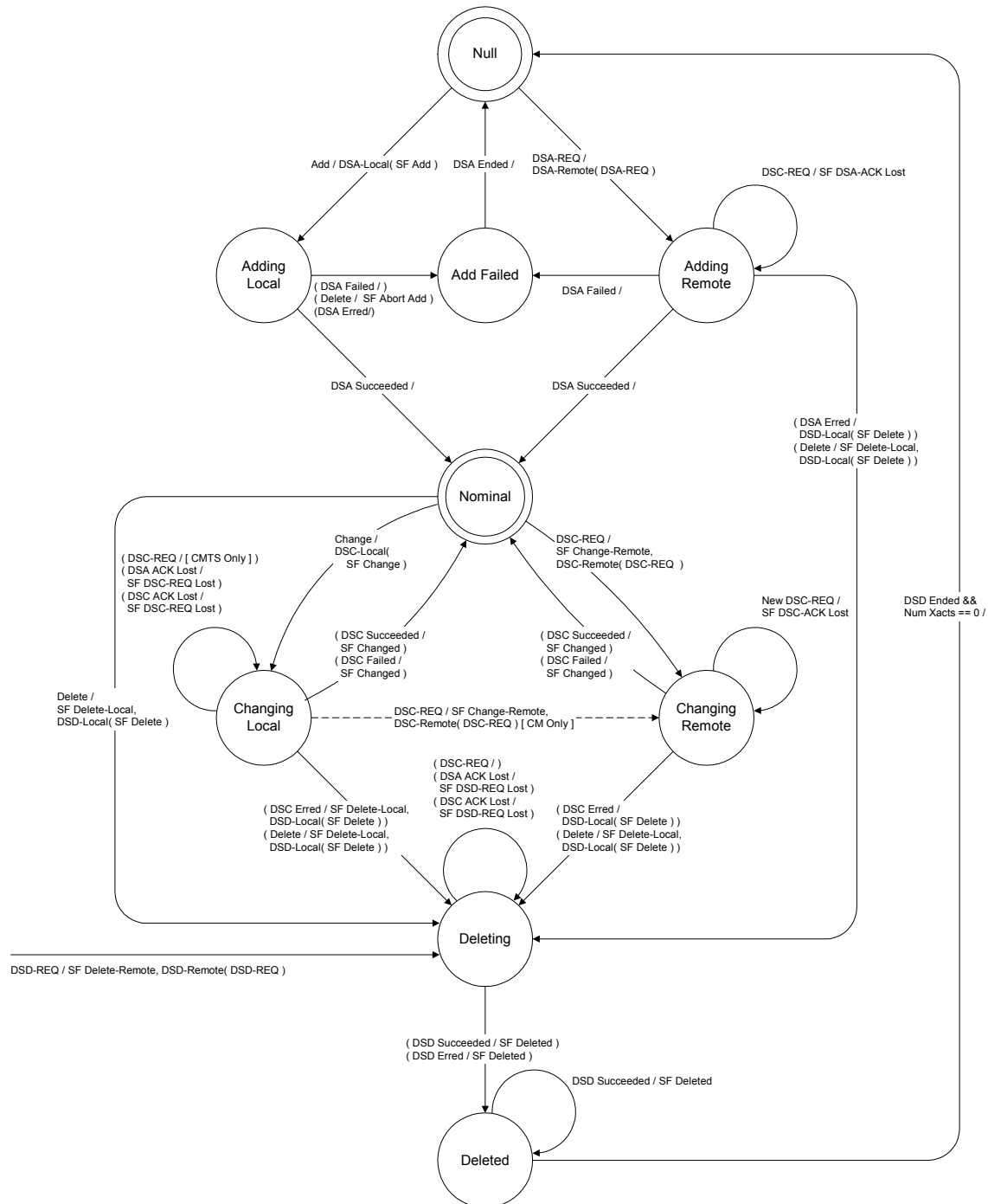
FIGURE 11-21. Dynamic Service Flow State Transition Diagram
