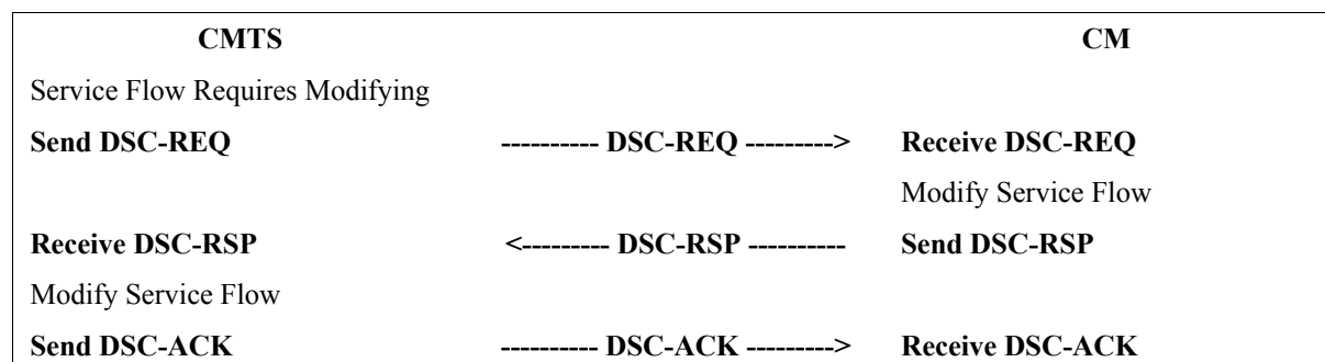
FIGURE 11-40. CMTS-Initiated DSC
