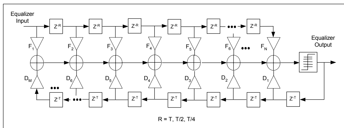
FIGURE 8-24. Generalized Equalizer Tap Location Definition
