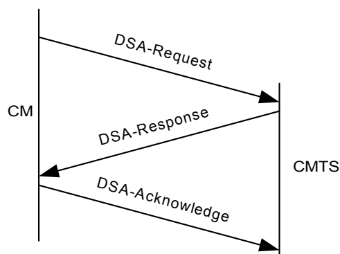
FIGURE 10-6. Dynamic Service Addition Message Flow - CM Initiated
