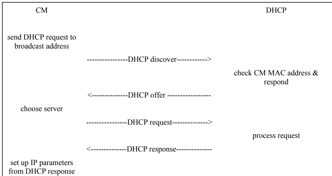
FIGURE 11-10. Establishing IP Connectivity
