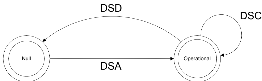
FIGURE 11-20. Dynamic Service Flow Overview
