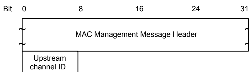
FIGURE 8-29. Upstream Channel Change Request
