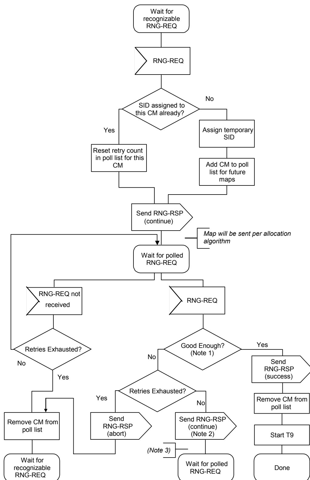
FIGURE 11-8. Initial Ranging - CMTS
