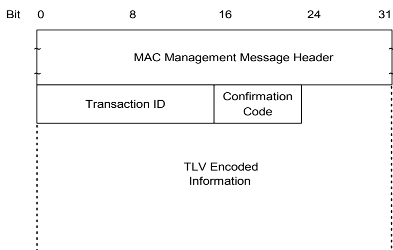
FIGURE 8-35. Dynamic Service Change - Response
