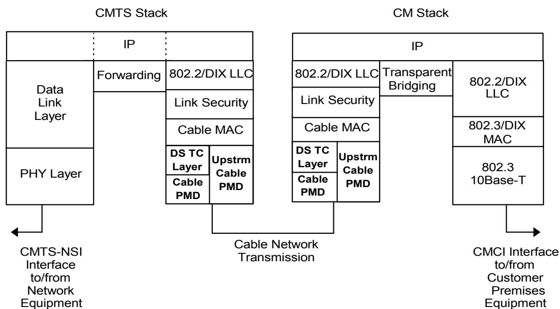
FIGURE 5-2. Data forwarding through the CM and CMTS
