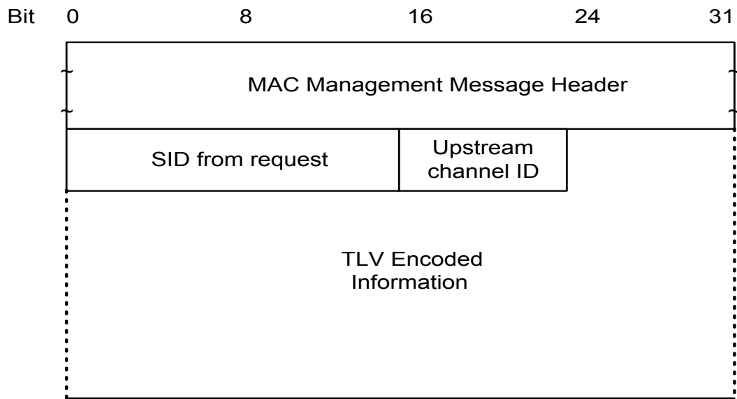
FIGURE 8-22. Ranging Response
