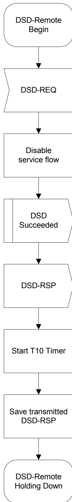
FIGURE 11-55. DSD—Remotely Initiated Transaction Begin State Flow Diagram
