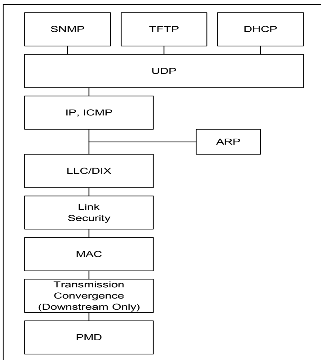
FIGURE 5-1. Protocol stack on the RF interface
