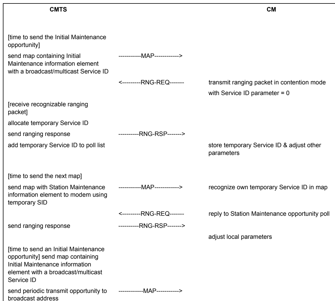
FIGURE 11-5. Ranging and Automatic Adjustments Procedure
