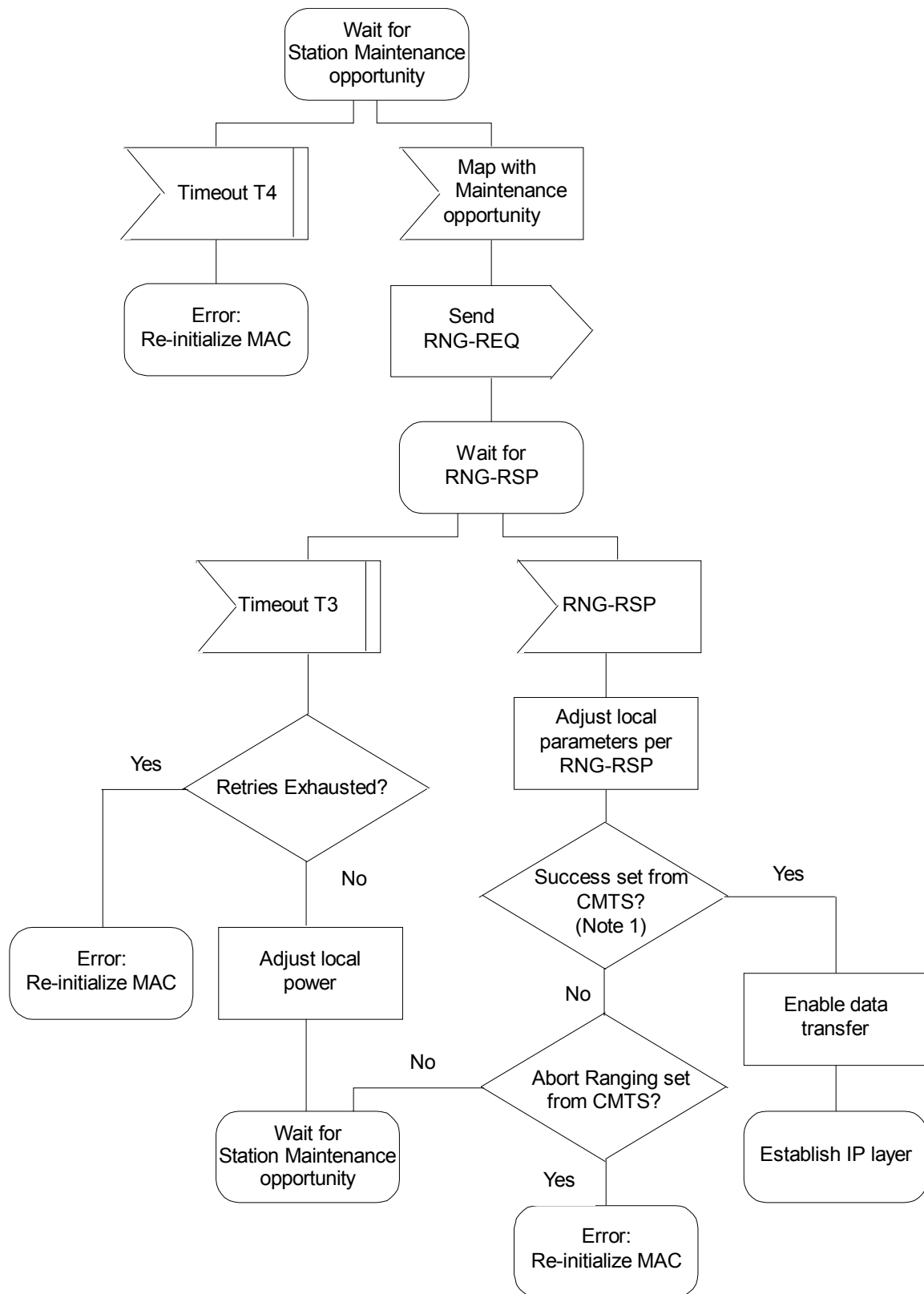
FIGURE 11-7. Initial Ranging - CM (continued)
