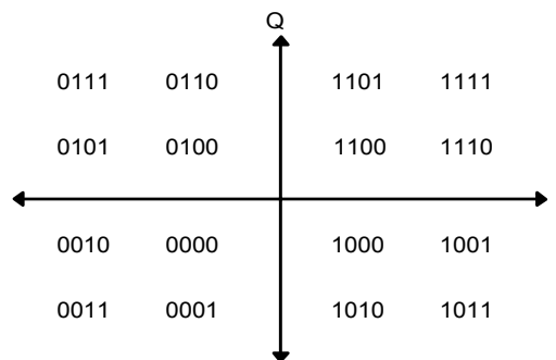
FIGURE 6-3. 16QAM differential-coded symbol mapping
