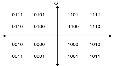
FIGURE 6-2. 16QAM Gray-coded symbol mapping
