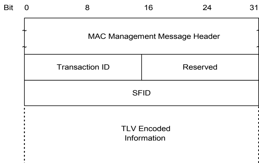
FIGURE 8-37. Dynamic Service Deletion - Request
