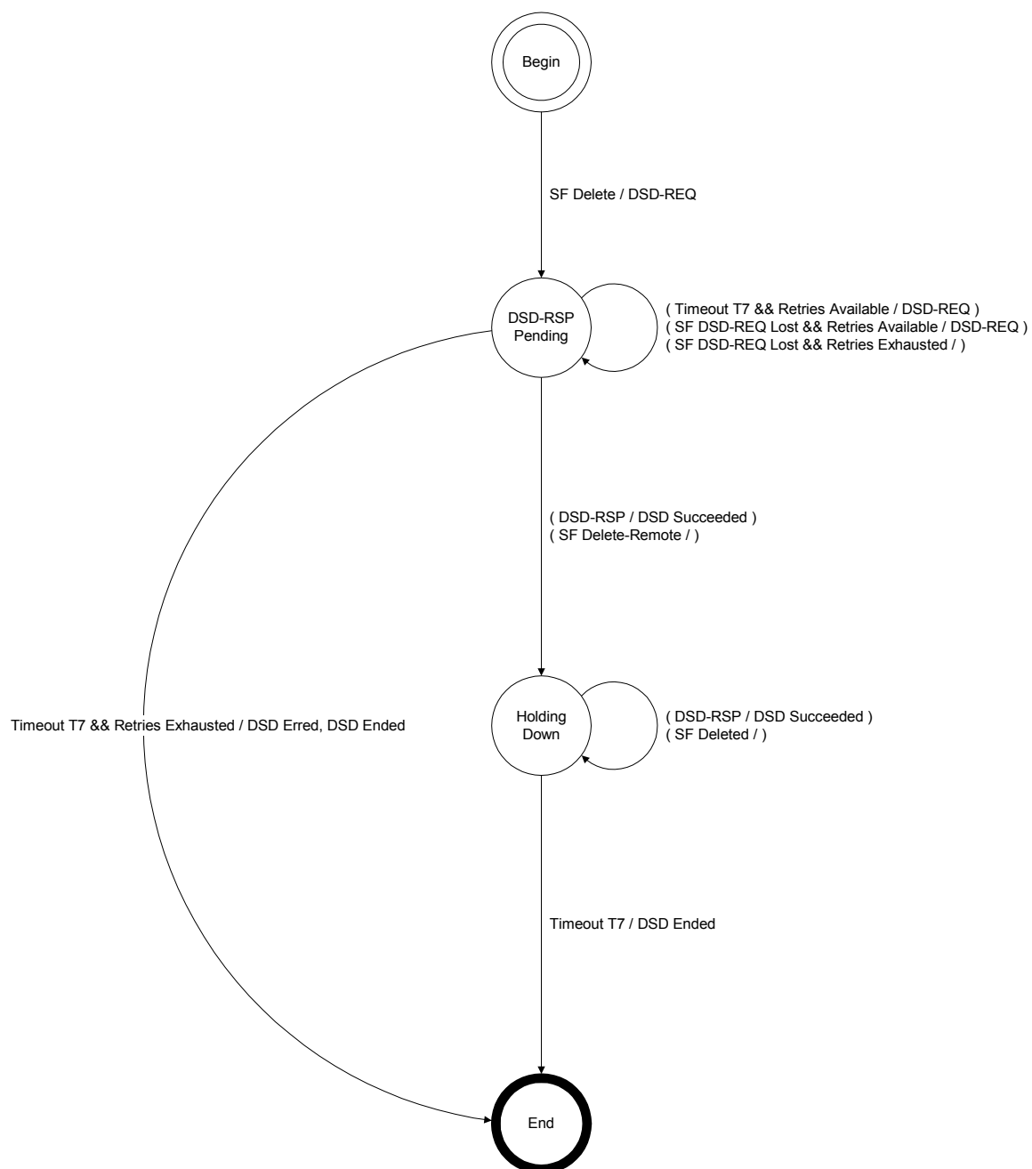
FIGURE 11-26. DSD—Locally Initiated Transaction State Transition Diagram
