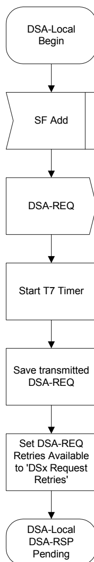
FIGURE 11-30. DSA—Locally Initiated Transaction Begin State Flow Diagram
