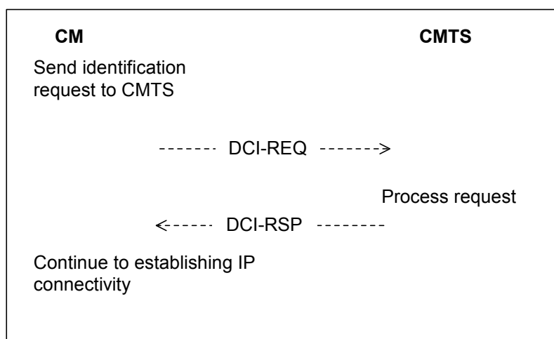
FIGURE 11-9. Device Class Identification
