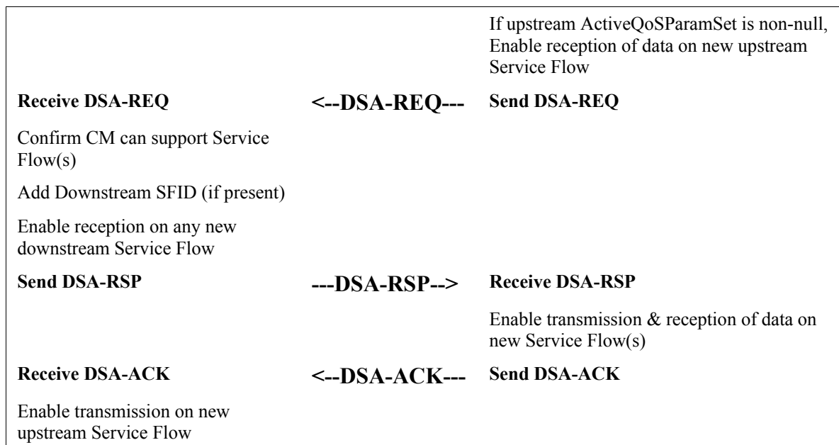
FIGURE 11-29. Dynamic Service Addition Initiated from CMTS
