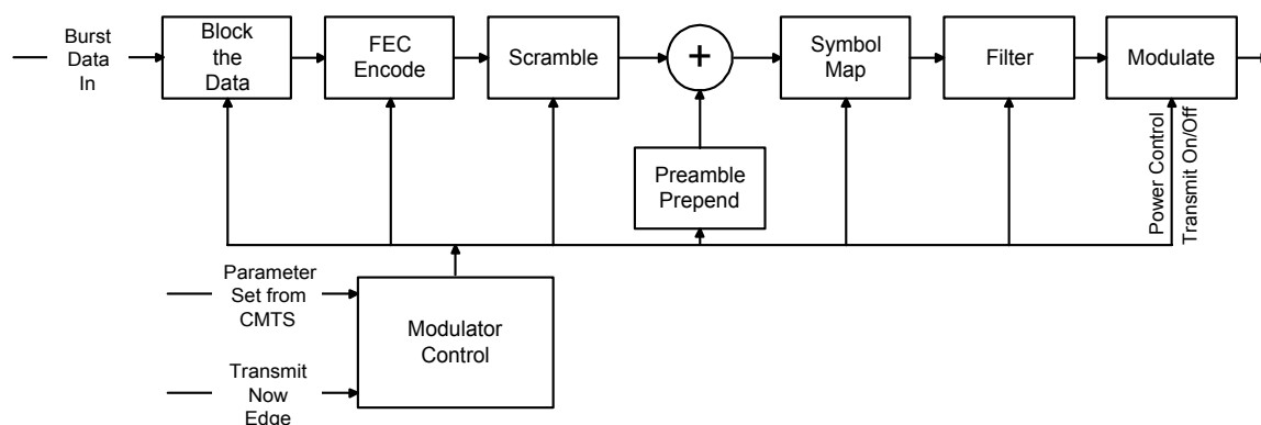
FIGURE 6-9. Signal-processing sequence
