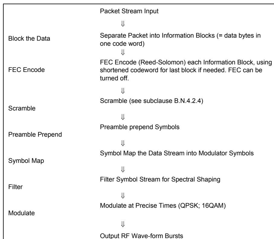
FIGURE N-10. TDMA upstream transmission processing
