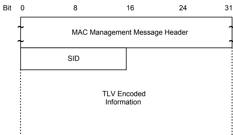
FIGURE 8-26. Registration Request
