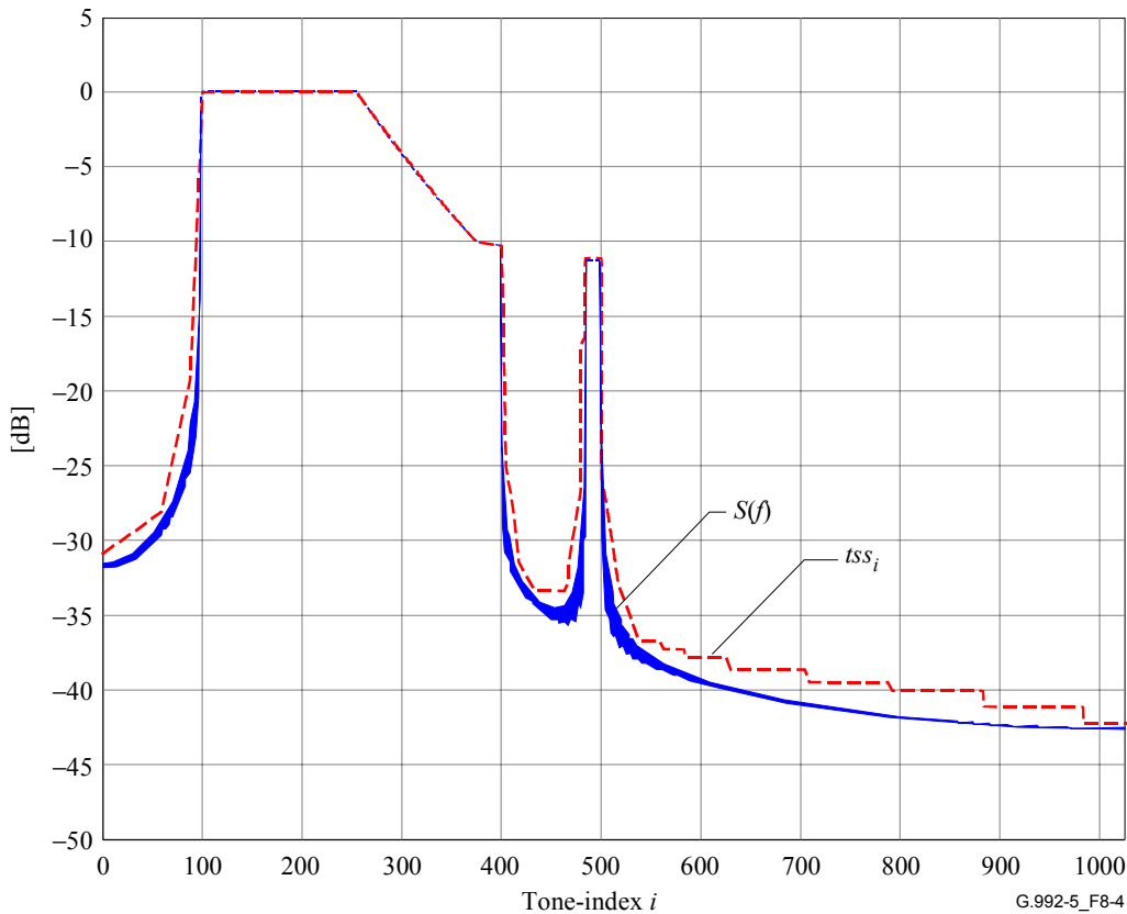
Figure 8-4/G.992.5 – Example of the downstream \log_{tss_i} values (in dB) as function of the subcarrier index
