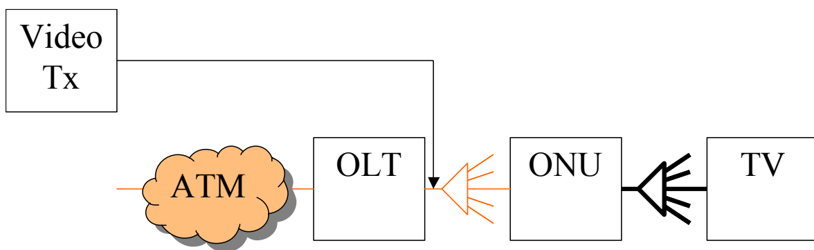
Fig. A.1/G.983.2a2. A B-PON with broadcast video only.
