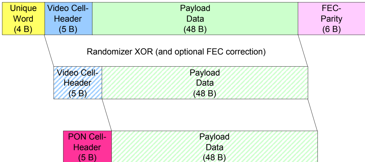
Fig. A.4/G.983.2a2. The transformation of a 55-2 formatted burst into ATM datagrams.
