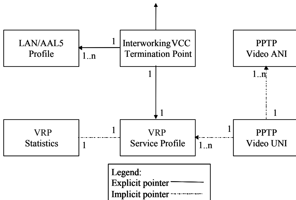
Figure 1/G.983.2a2 – Managed Entity relation diagram for Video Return Path service support
