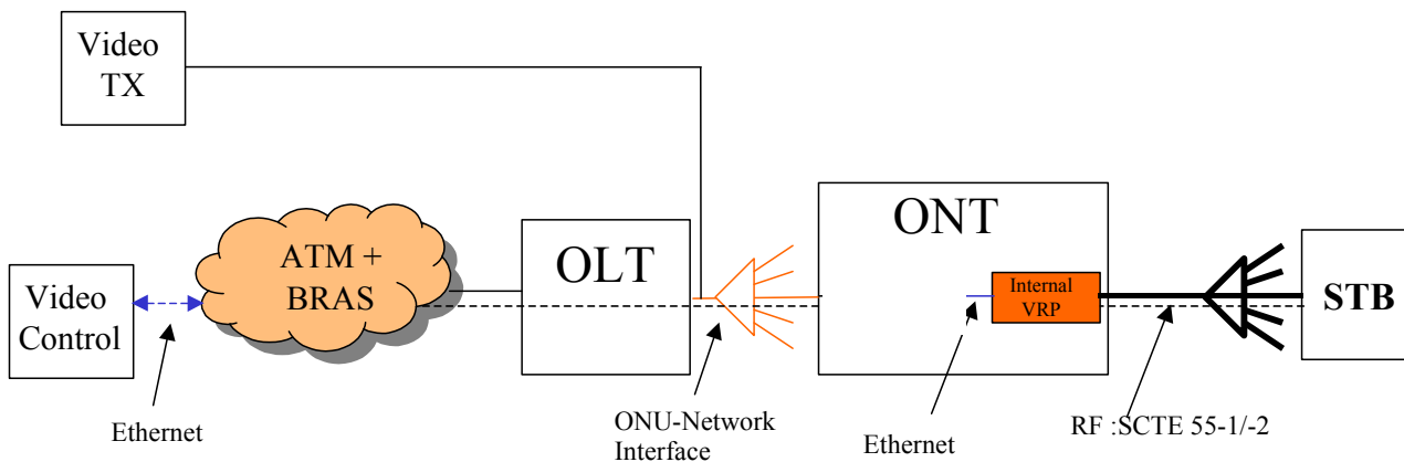
Fig. I.3/G.983.2a2. A B-PON interactive video services with internal VRP adaptation.
