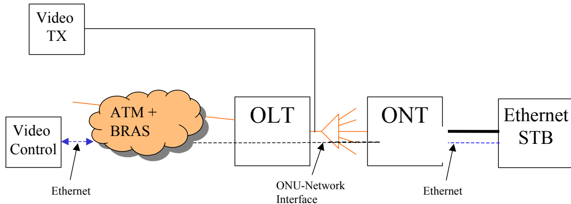
Fig. I.1/G.983.2a2. A B-PON with ONT transparent support of interactive video services.
