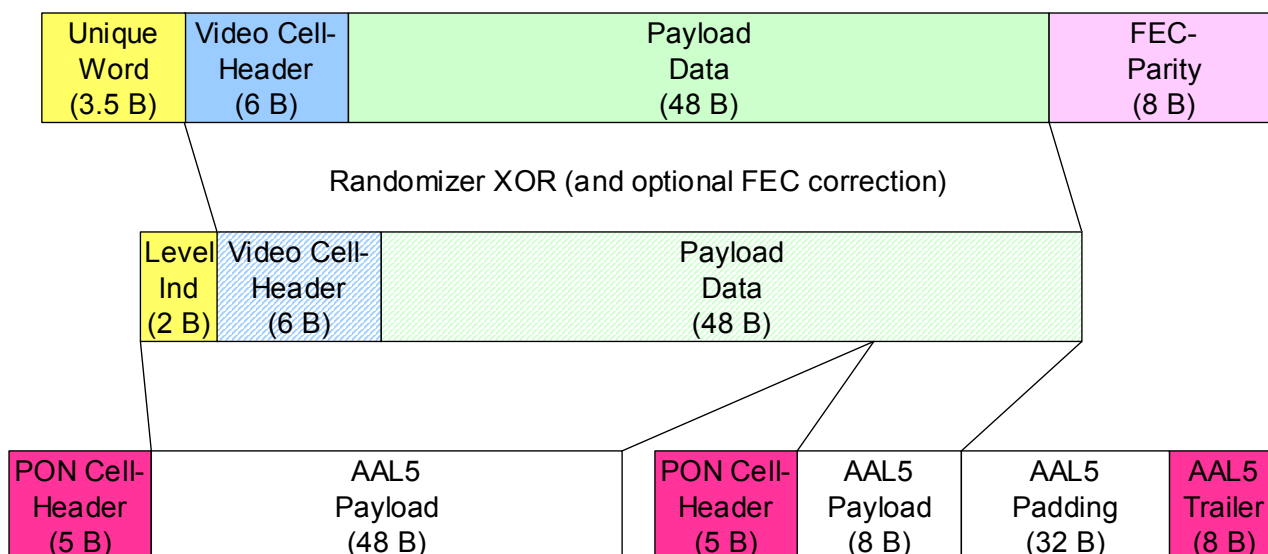
Fig. A.3/G.983.2a2. The transformation of a 55-1 formatted burst into ATM datagrams.
