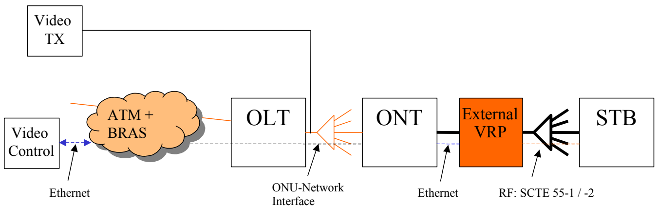
Fig. I.2/G.983.2a2. A B-PON interactive video services with external VRP adaptation.
