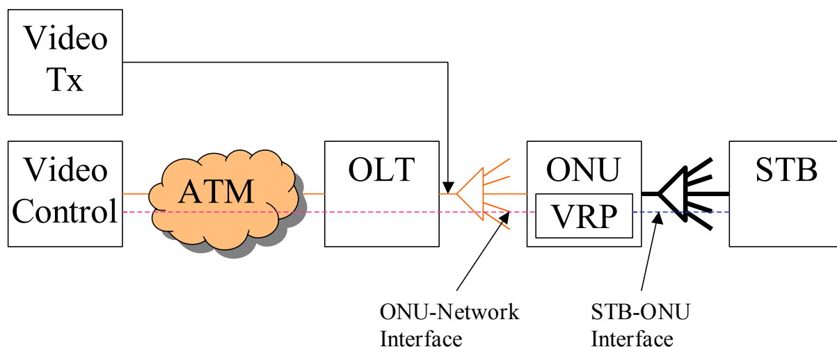
Fig. A.2/G.983.2a2. A B-PON with interactive video services.
