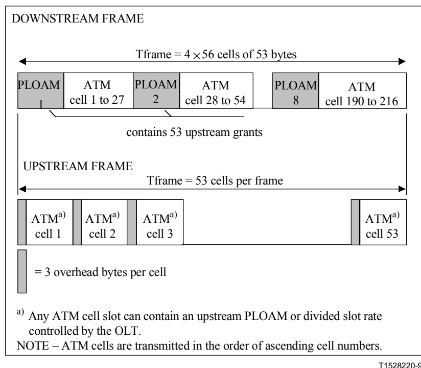
Figure 12/G.983.1 – Frame format for 622.08/155.52 Mbit/s PON
