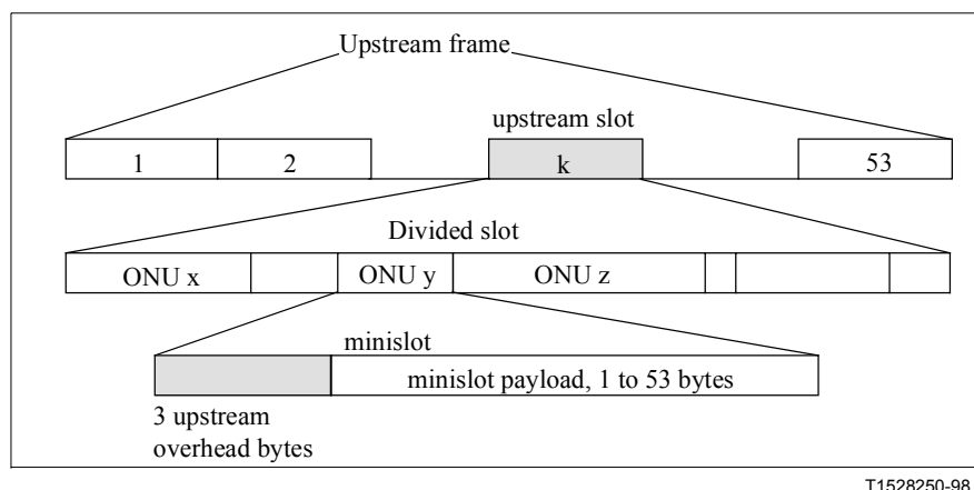
Figure 18/G.983.1 – Format of divided_slot
