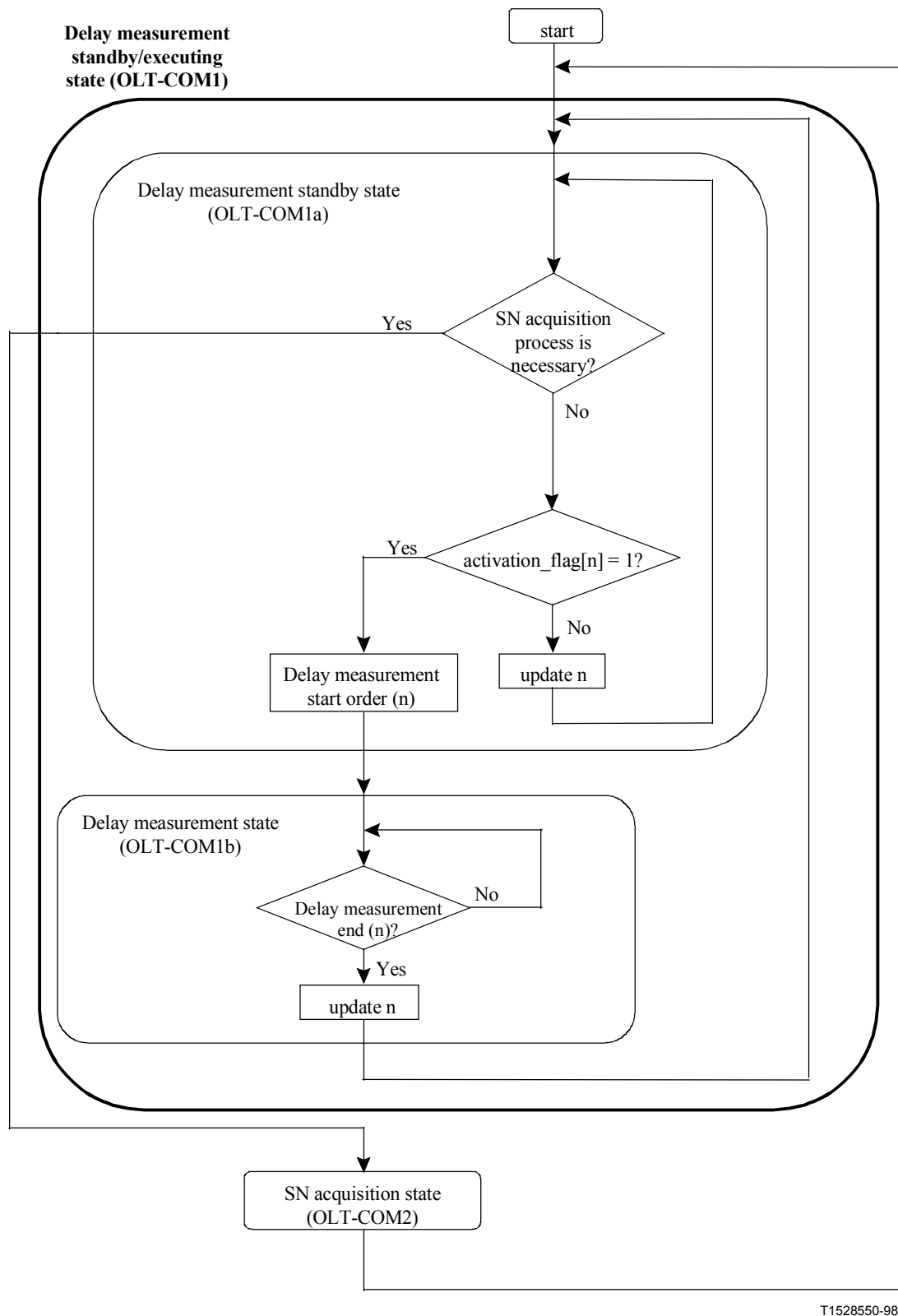
Figure III.2/G.983.1 – Ranging flow [OLT] (example) (sheet 2 of 7)
