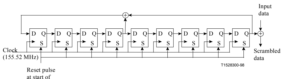
Figure 23/G.983.1 – Upstream scrambler
