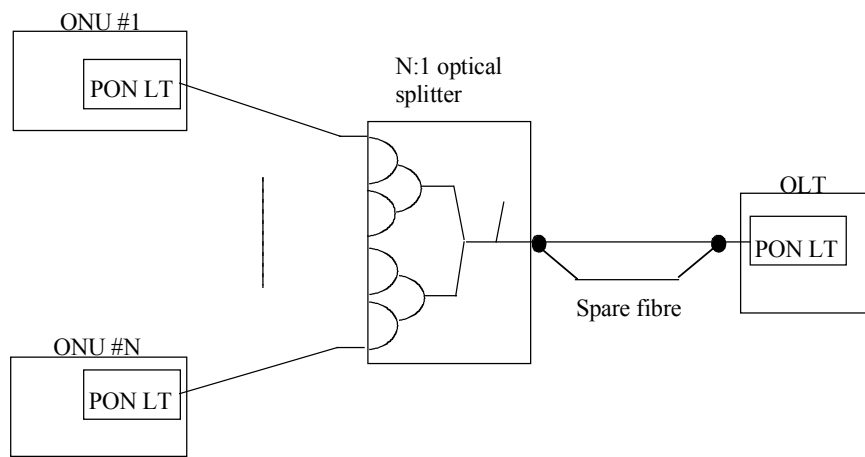
a) Fibre duplex system
