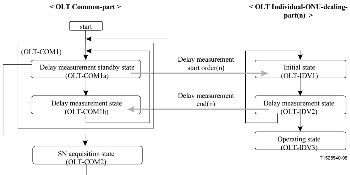
Figure III.2/G.983.1 – Ranging flow [OLT] (example) (sheet 1 of 7)
