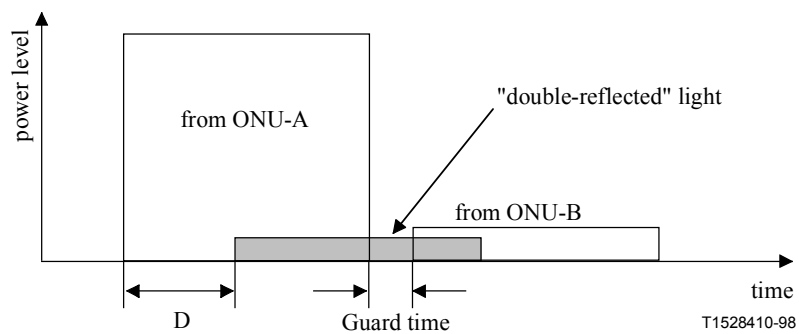
Figure I.3/G.983.1 – Effect of disconnecting a connector near ONU
