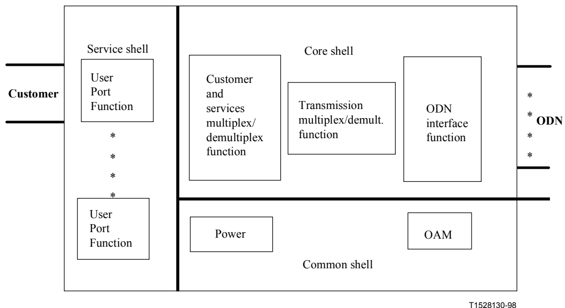
Figure 3/G.983.1 – Example of ONT functional blocks
