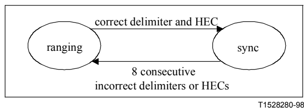
Figure 21/G.983.1 – Cell delineation state diagram
