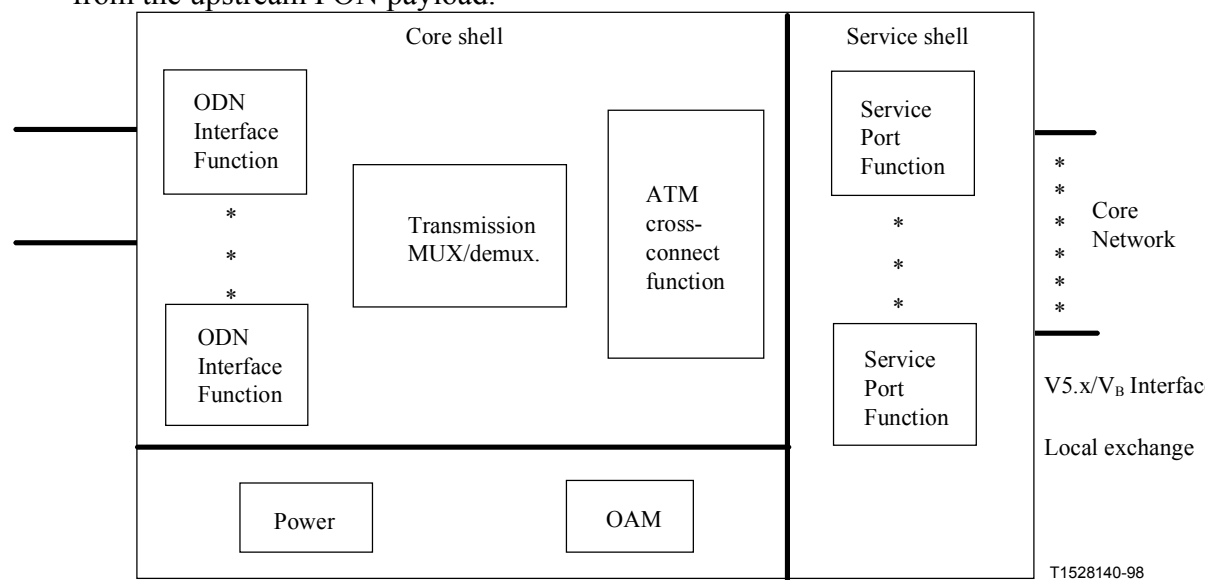
Figure 4/G.983.1 – Example of OLT functional blocks
