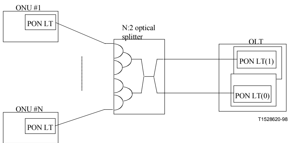
b) OLT-only duplex system
