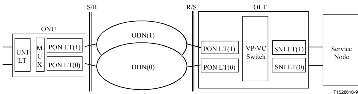
Figure IV.1/G.983.1 – Duplex system model
