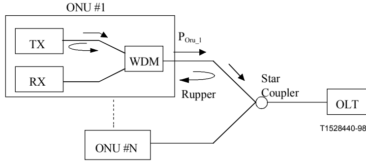
Figure II.3/G.983.1 – Model 1 for incidence into OLT receiver
