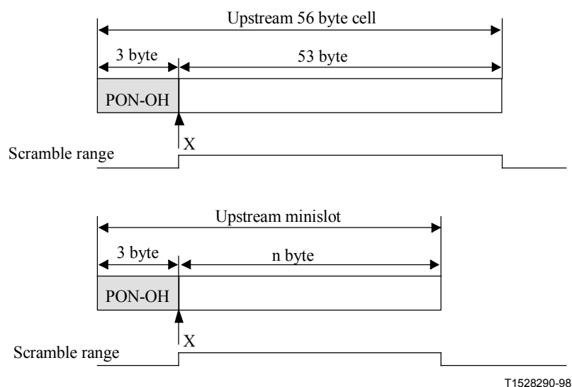
Figure 22/G.983.1 – Upstream scrambler
