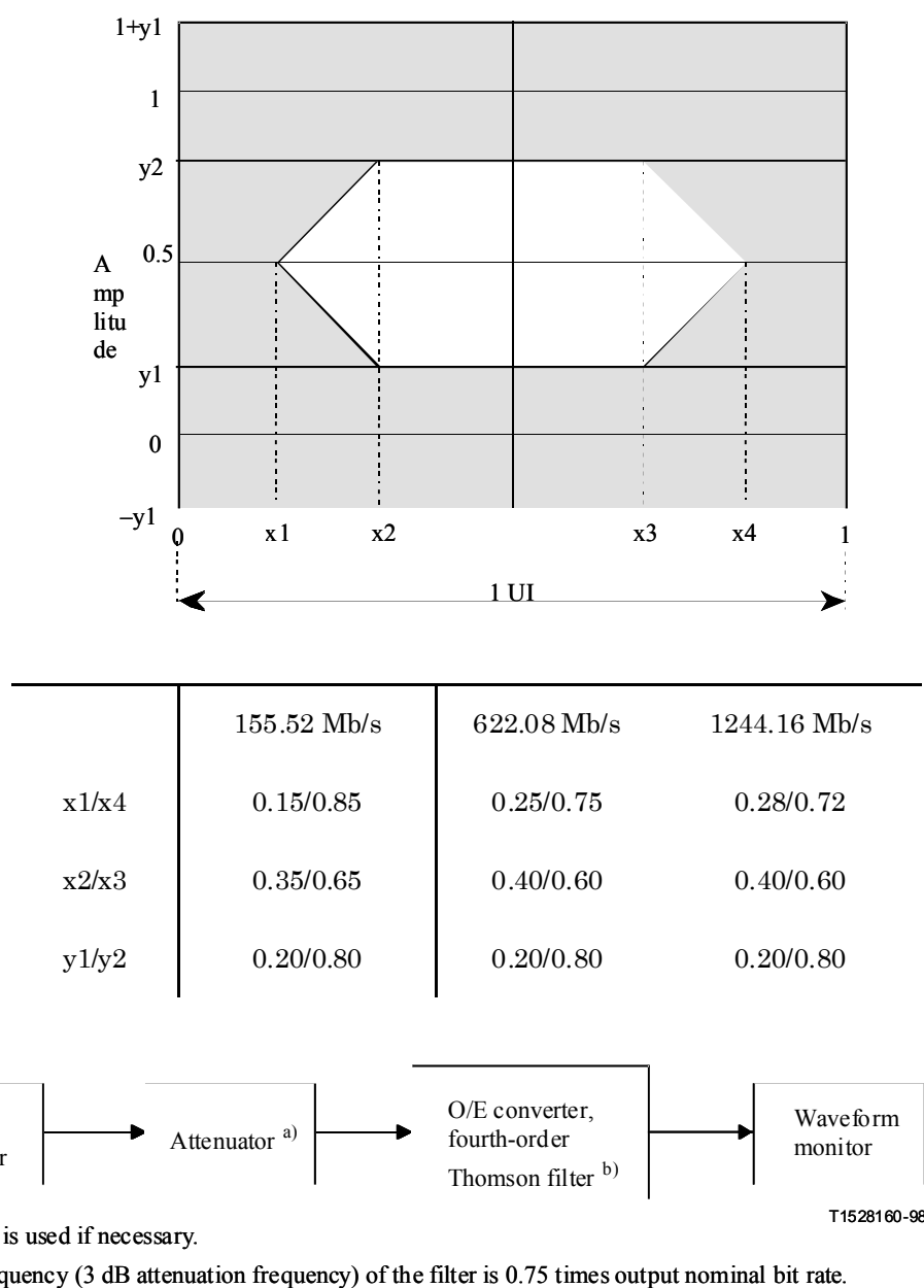
Figure 6/G.983.1 – Mask of the eye diagram for the downstream transmission signal
