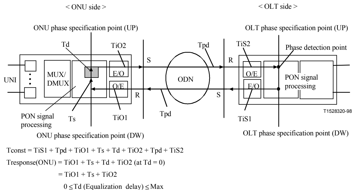
Figure 25/G.983.1 – Configuration of the specification points
