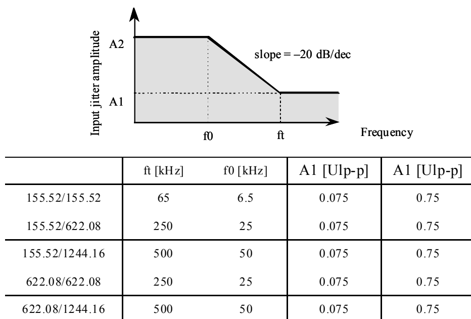
Figure 9/G.983.1 – Jitter tolerance mask for ONU
