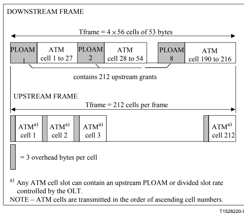
Figure 13/G.983.1 – Frame format for 622.08/622.08 Mbit/s PON
