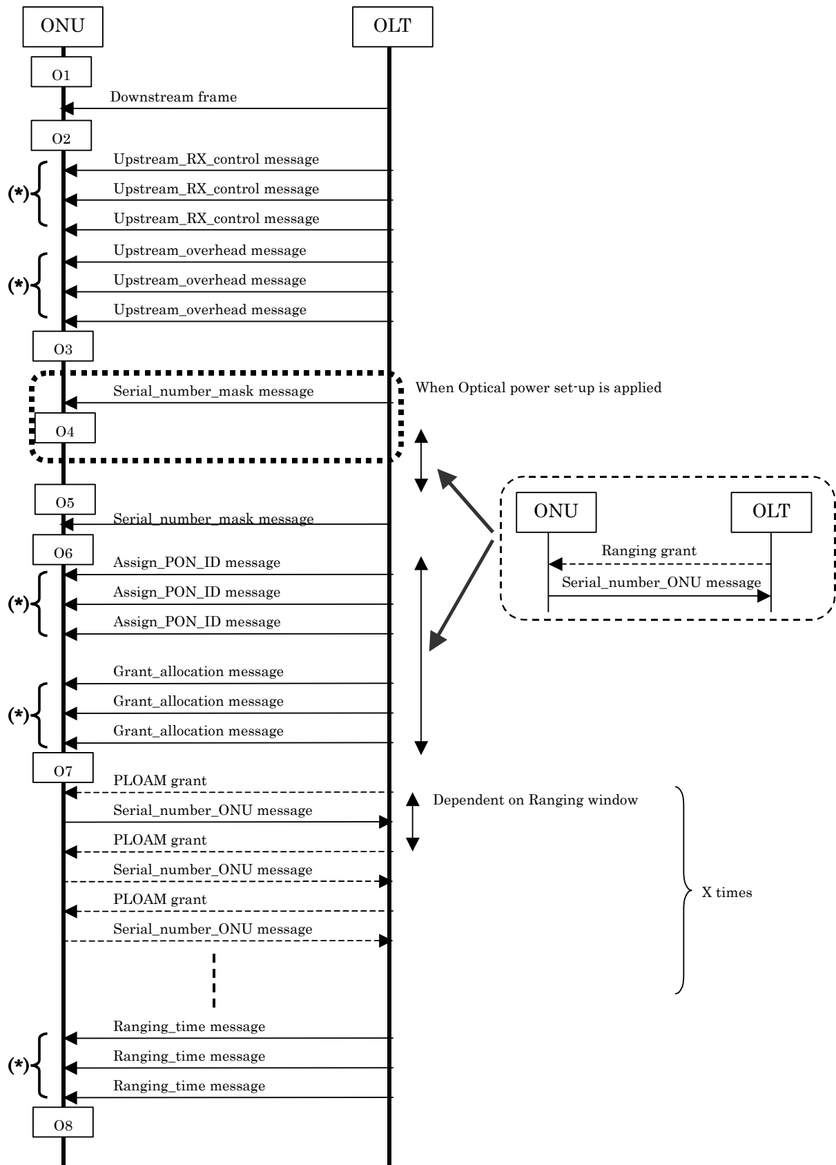
Figure 31/G.983.1 - Message Sequence for Ranging
