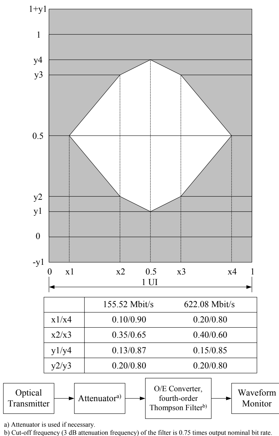
Figure 7/G.983.1 – Mask of the eye diagram for the upstream transmission signal
