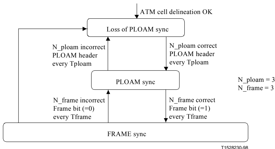
Figure 16/G.983.1 – Frame synchronization flow
