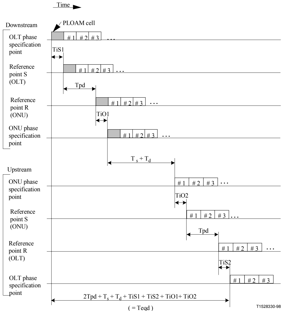
Figure 26/G.983.1 – Phase relationship between downstream and upstream
