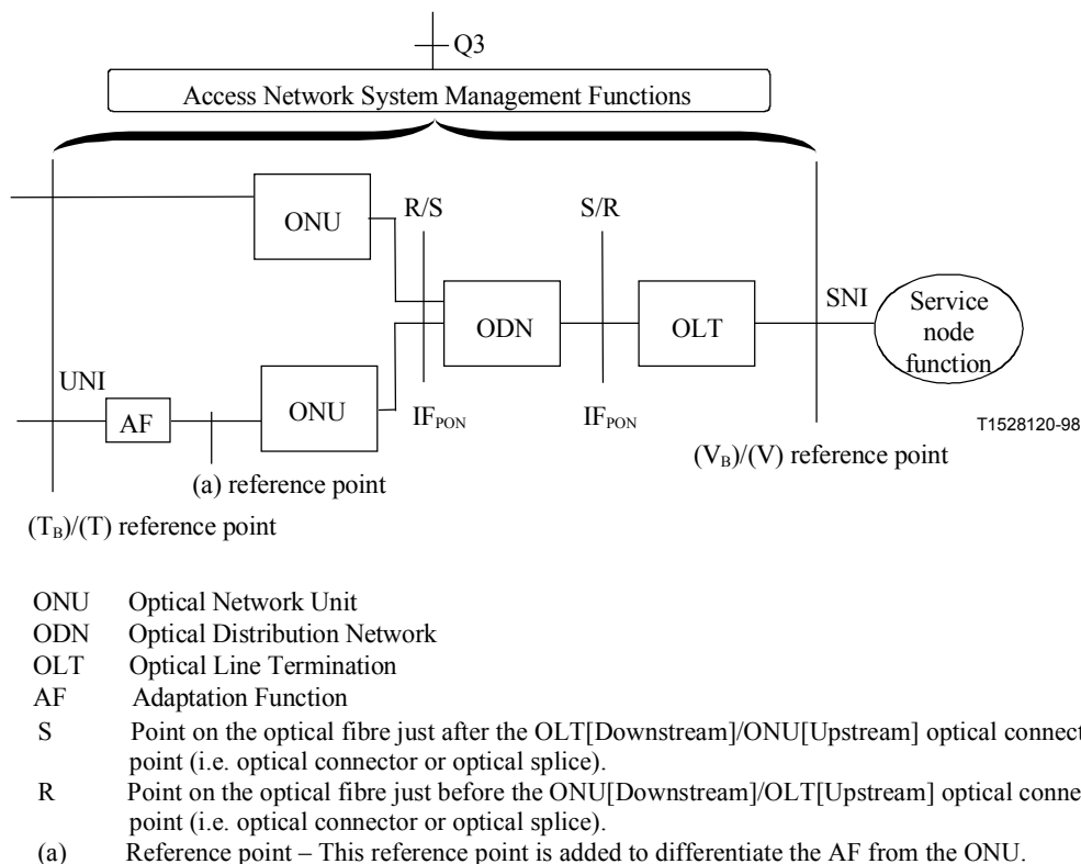
Figure 2/G.983.1 – Reference configuration for an ATM based PON
