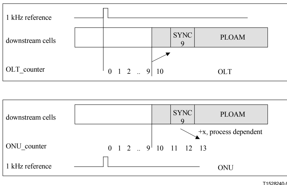
Figure 17/G.983.1 – 1 kHz reference extraction in ONU
