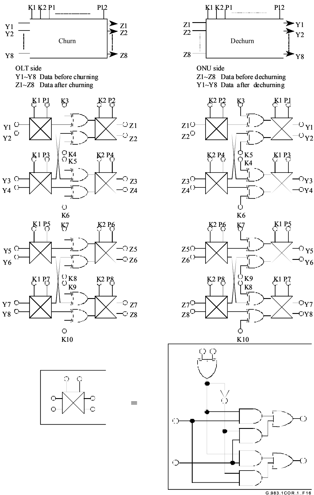
19/G.983.1 – Churning
