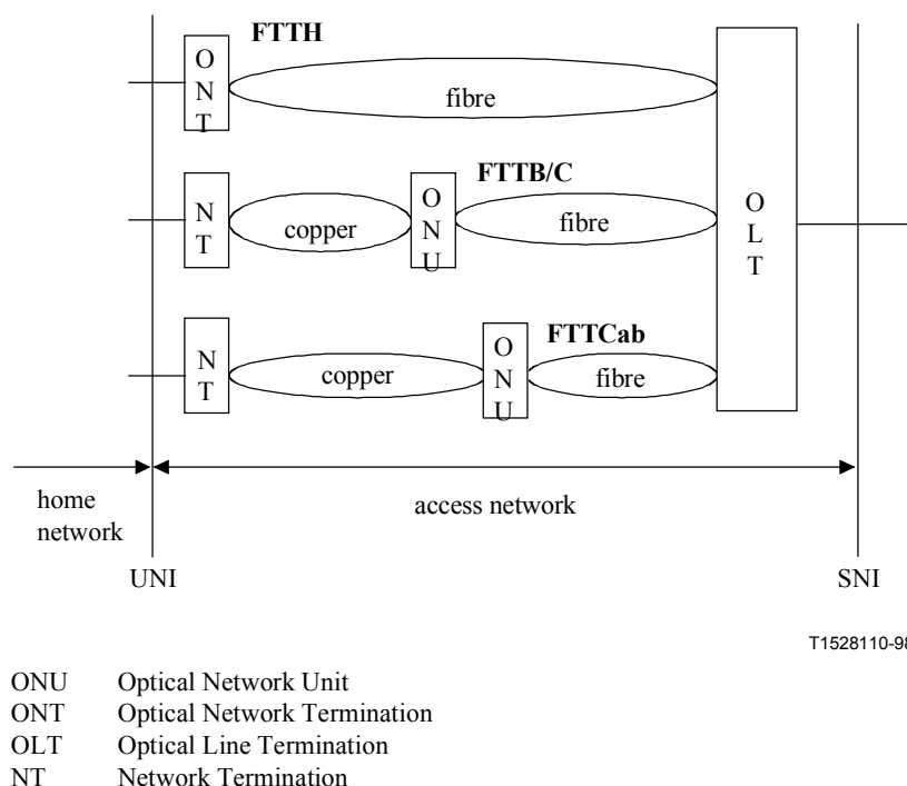
Figure 1/G.983.1 – Network architecture
