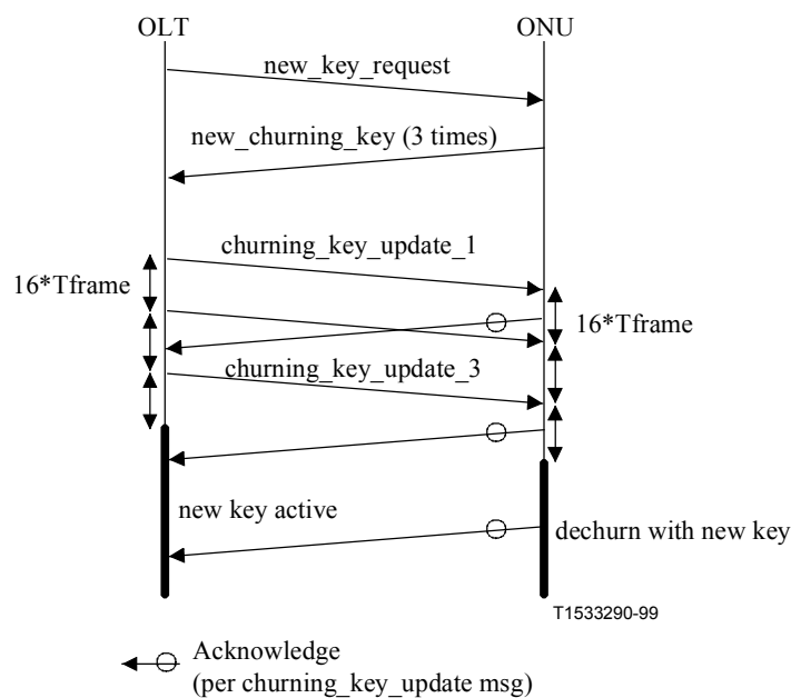
Figure 20/G.983.1 – Churning message flow
