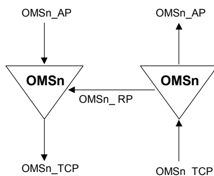
Figure 0-4/G.798 – OMSn_TT
