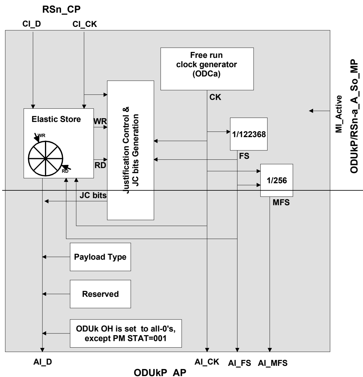
Figure 0-45/G.798 - ODUkP/RSn-a_A_So processes
