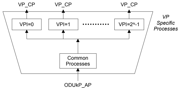
Figure 0-33/G.798 ODUkP/VP_A_Sk atomic function decomposed into Specific and Common Processes parts
