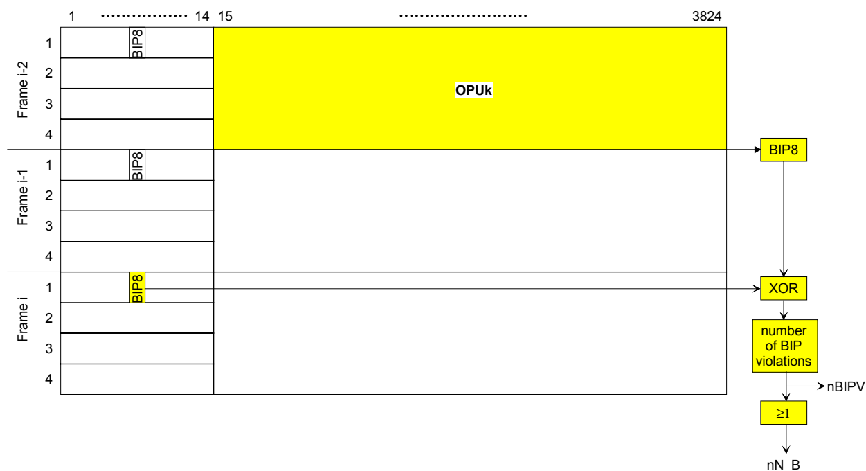
Figure 0-2/G.798 – BIP-8 sink processing (SM OH used as example)
