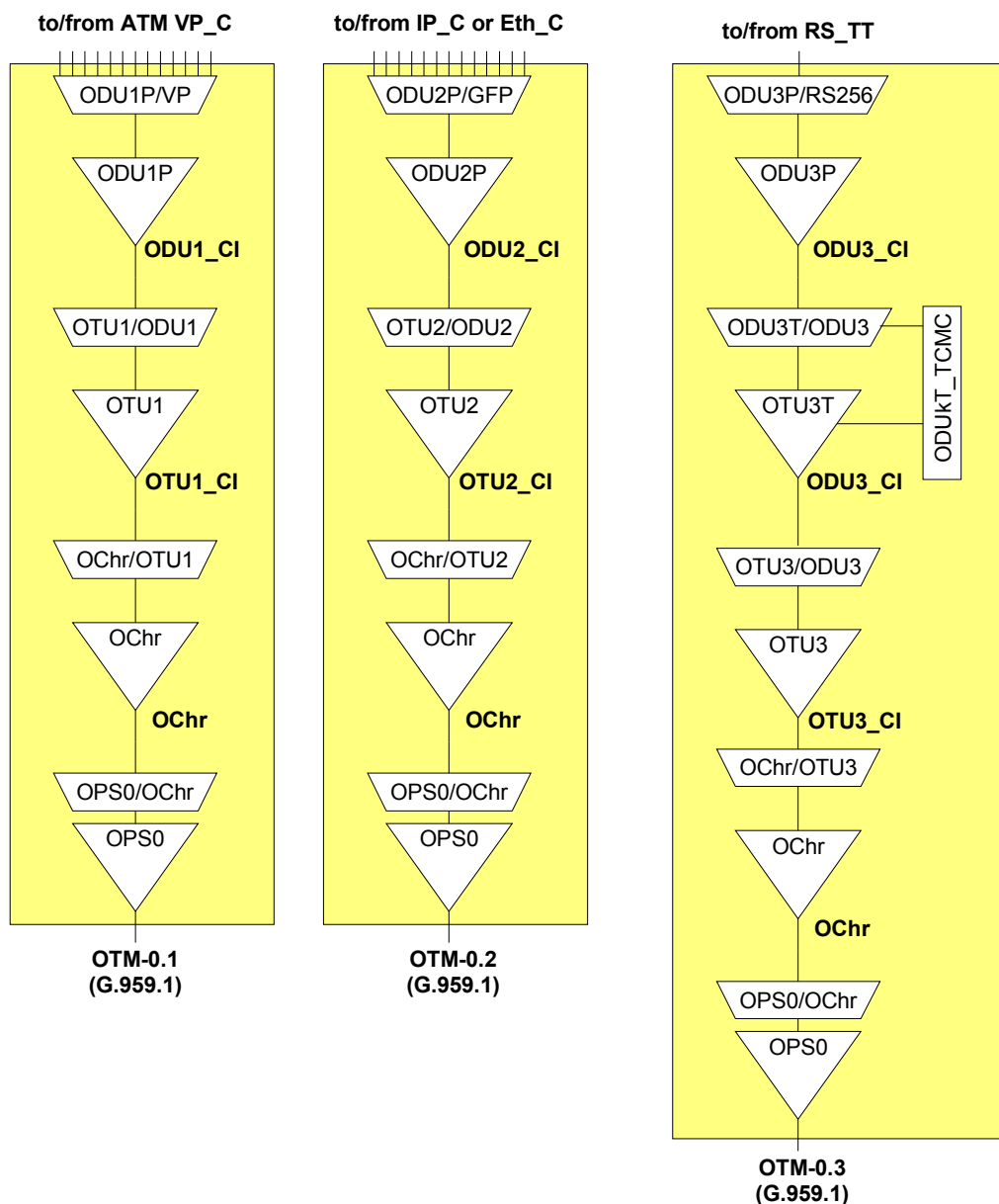
Figure I-4/G.798 – OTM-0.m interface ports on non-OTN equipment
