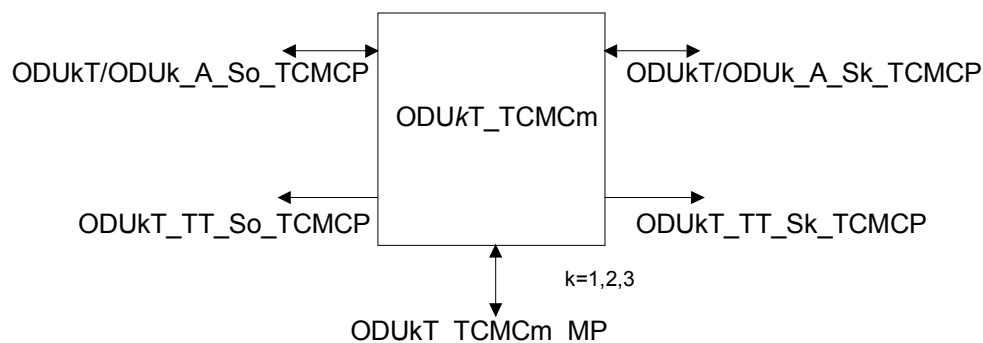
Figure 0-79/G.798 – ODUkT_TCMCm function
