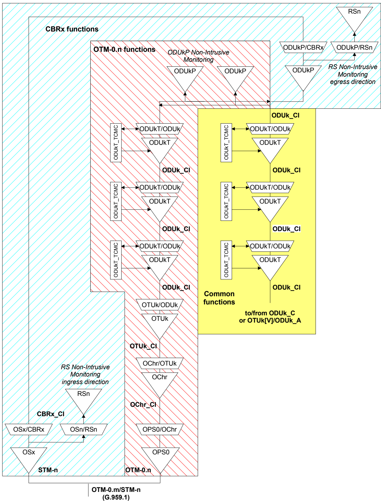
Figure I-3/G.798 - Selectable CBRx/OTM-0.m tributary interface port on OTN equipment
