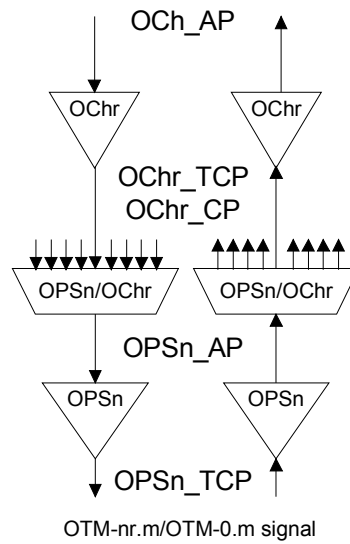
Figure 0-1/G.798 - OTN atomic functions specific for the reduced functionality OTM-nr.m/OTM-0.m interface
