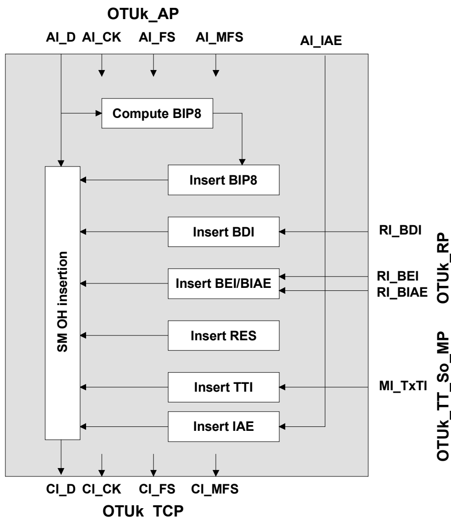
Figure 0-5/G.798 - OTUk_TT_So processes
