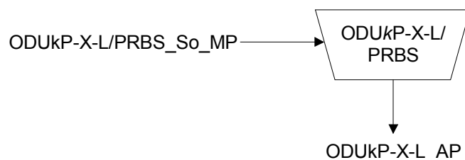
Figure 0-110/G.798 – ODUkP-X-L/PRBS A So function
