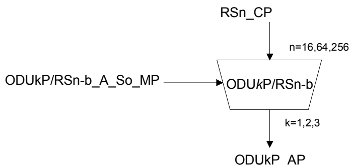
Figure 0-46/G.798 – ODUkP/RSn-b_A_So function
