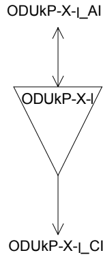
Figure 0-84/G.798 – ODUkP-X-L TT So symbol
