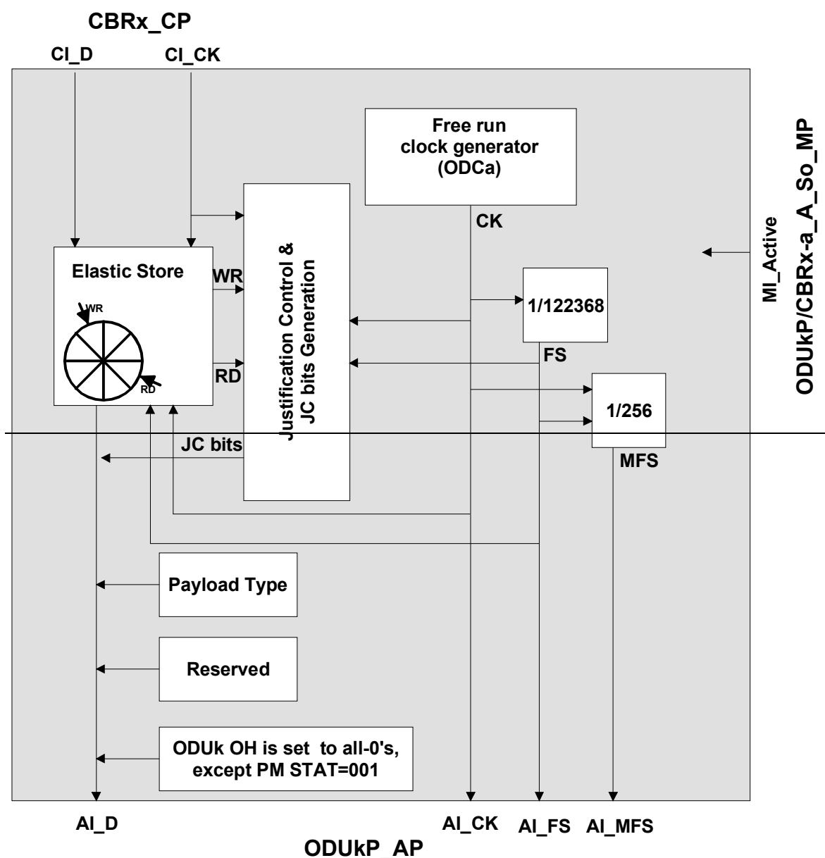
Figure 0-21/G.798 - ODUkP/CBRx-a_A_So processes
