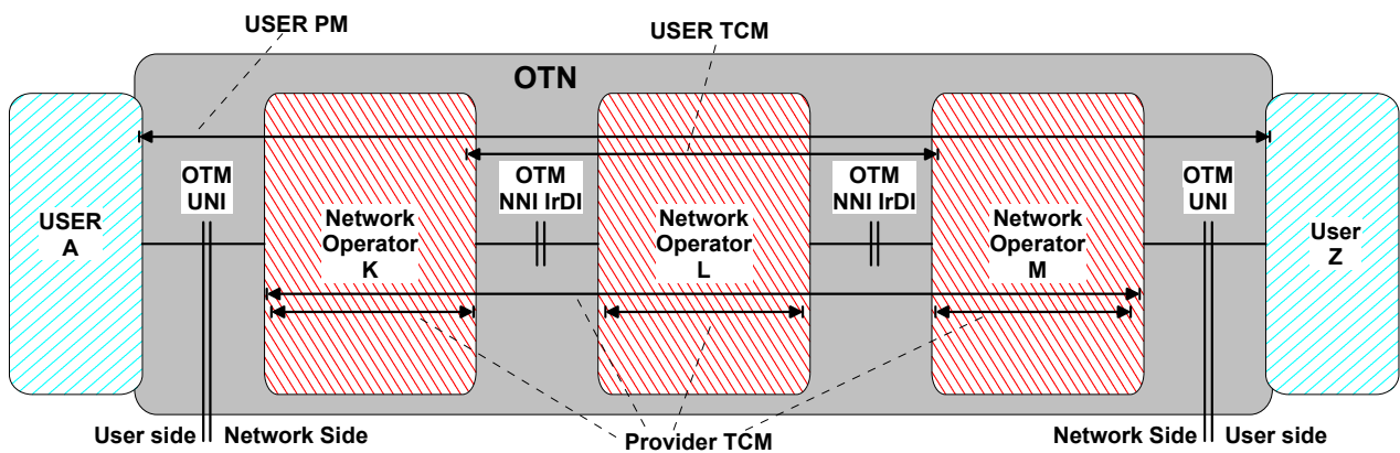
Figure II-3/G.798 - Provider and User Tandem Connections for case of OTM UNI interfaces and termination of the OTN on the user side of the UNI
