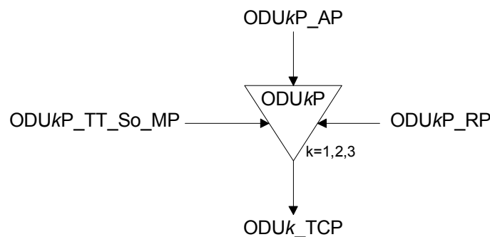
Figure 0-15/G.798 – ODUkP_TT_So function
