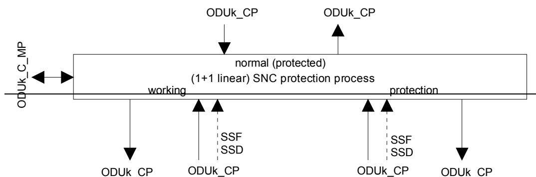
Figure 0-12/G.798 – 1+1 SNC/S and SNC/I protection process with APS protocol
