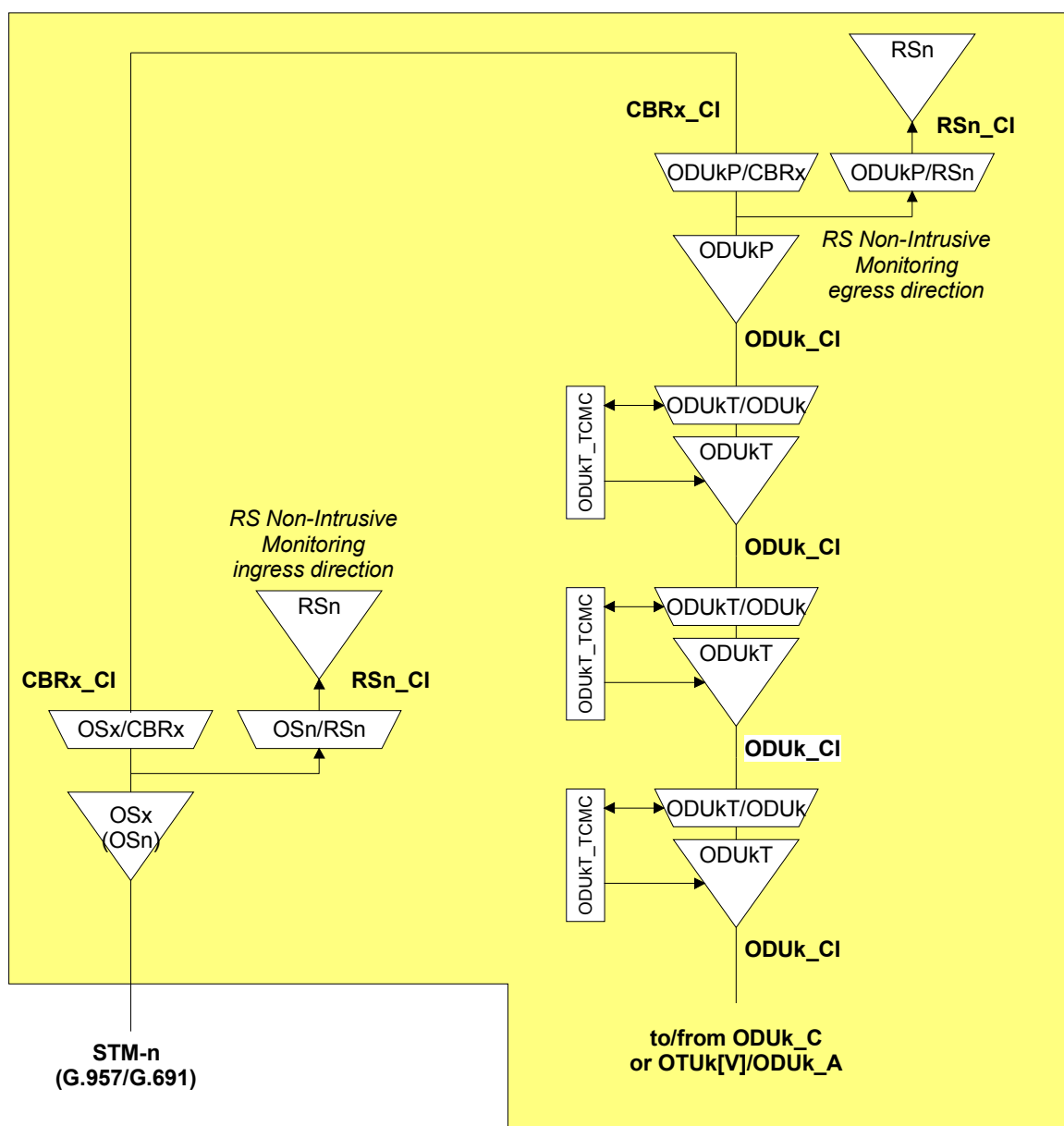
Figure I-1/G.798 - Transparent CBRx tributary interface port with optional SDH RS non-intrusive monitor on OTN equipment
