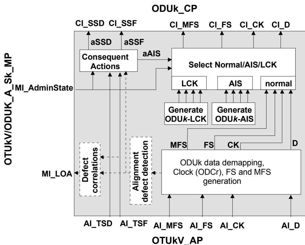
Figure 0-20/G.798 - OTUkV/ODUk_A_Sk processes
