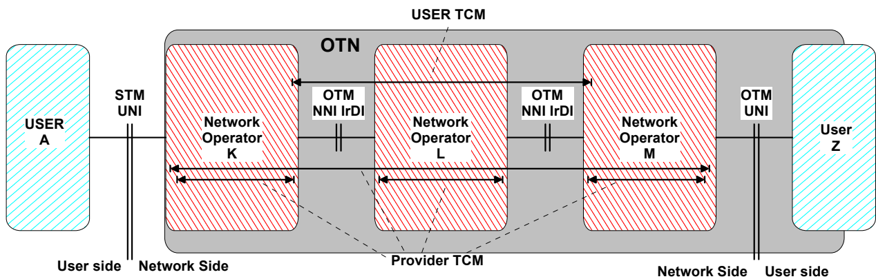
Figure II-2/G.798 - Provider and User Tandem Connections for case of mixed STM and OTM UNI interfaces
