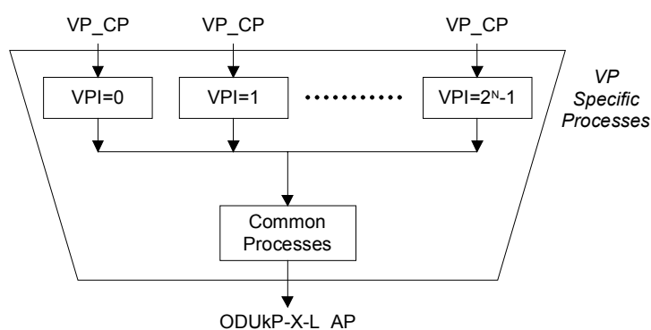
Figure 0-99/G.798 ODUkP-X-L/VP_A So atomic function decomposed into Specific and Common Processes parts
