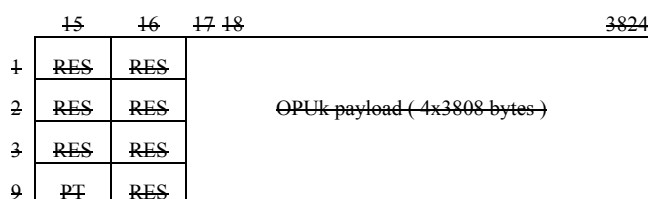
Figure 14-31/G.798 ODUkP_AI_So_D
