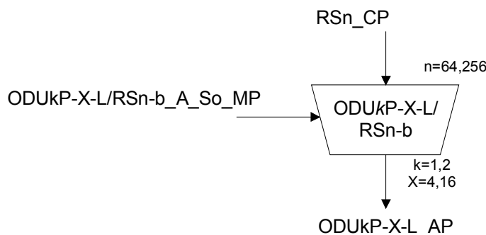
Figure 0-94/G.798 – ODUkP-X-L/RSn-b A So function
