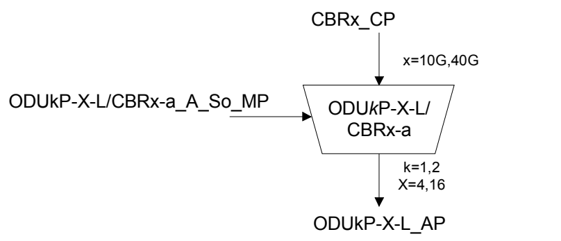
Figure 0-86/G.798 – ODUkP-X-L/CBRx-a A So function
