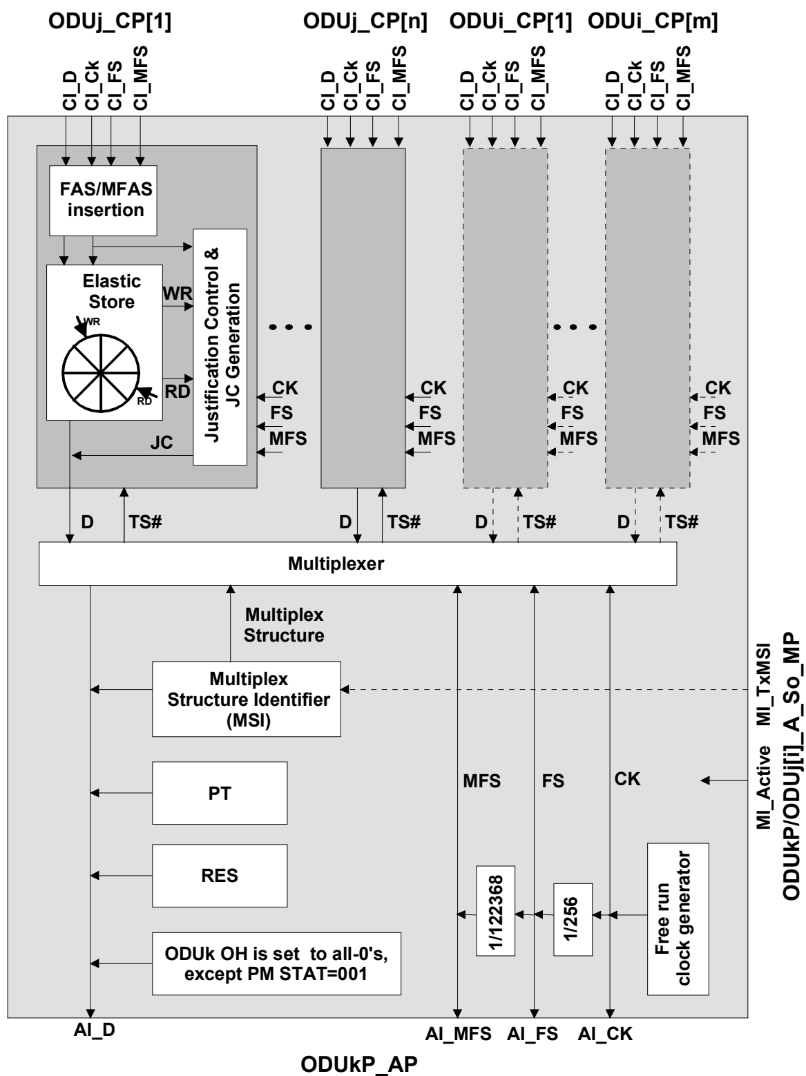
Figure 0-52/G.798 - ODUkP/ODUj[i] A So processes
