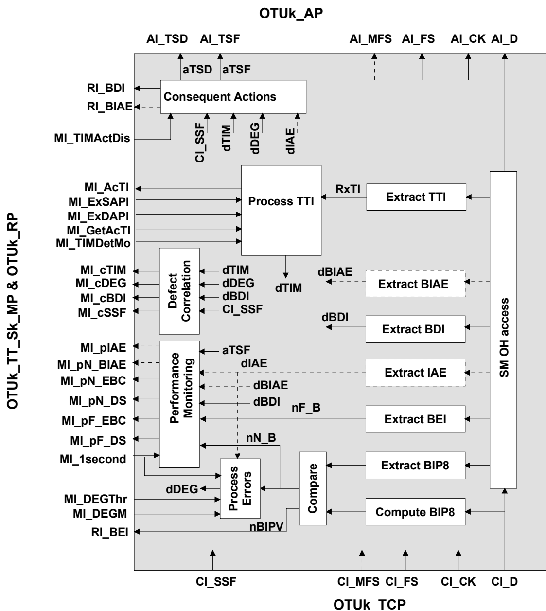
Figure 0-12/G.798 - OTUkV_TT_Sk processes
