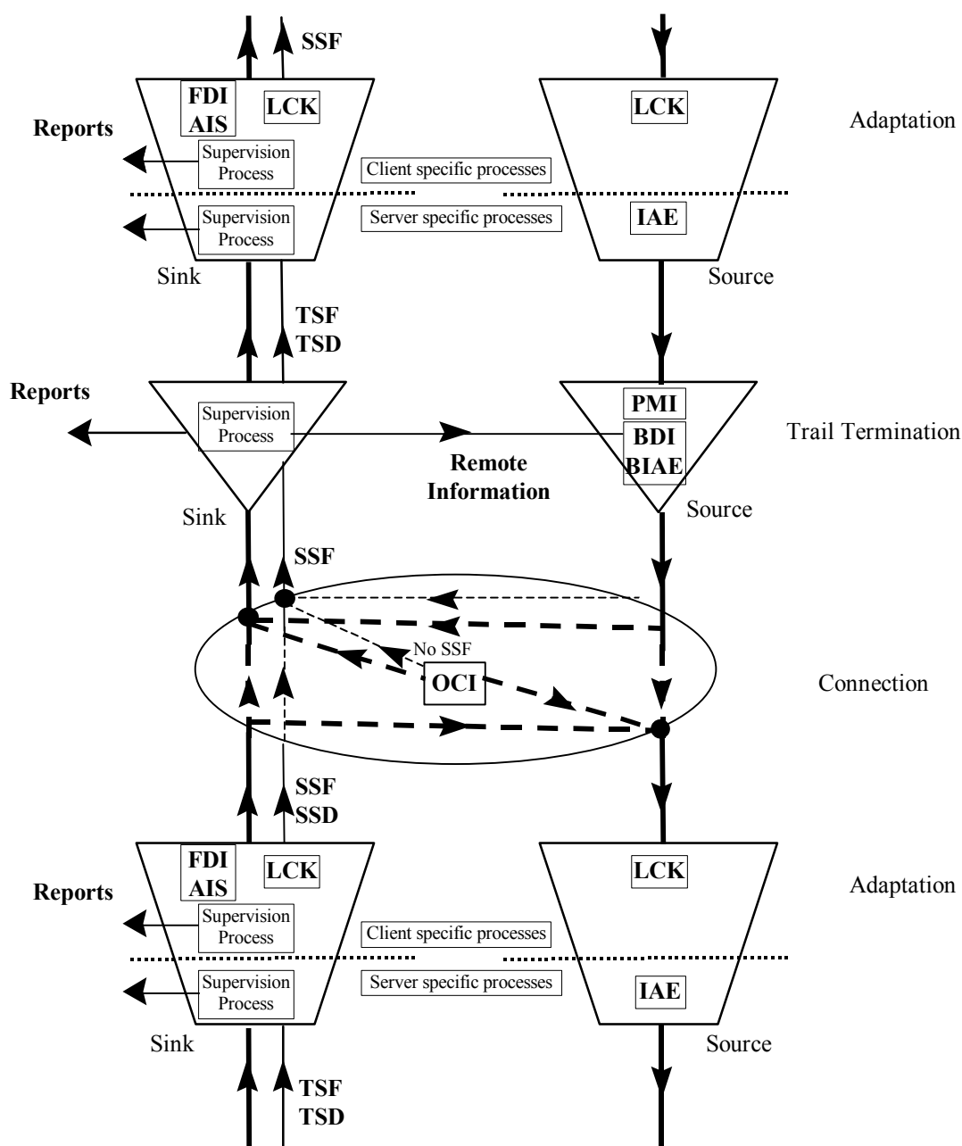
Figure 0-4/G.798 – Generic layer fault processing
