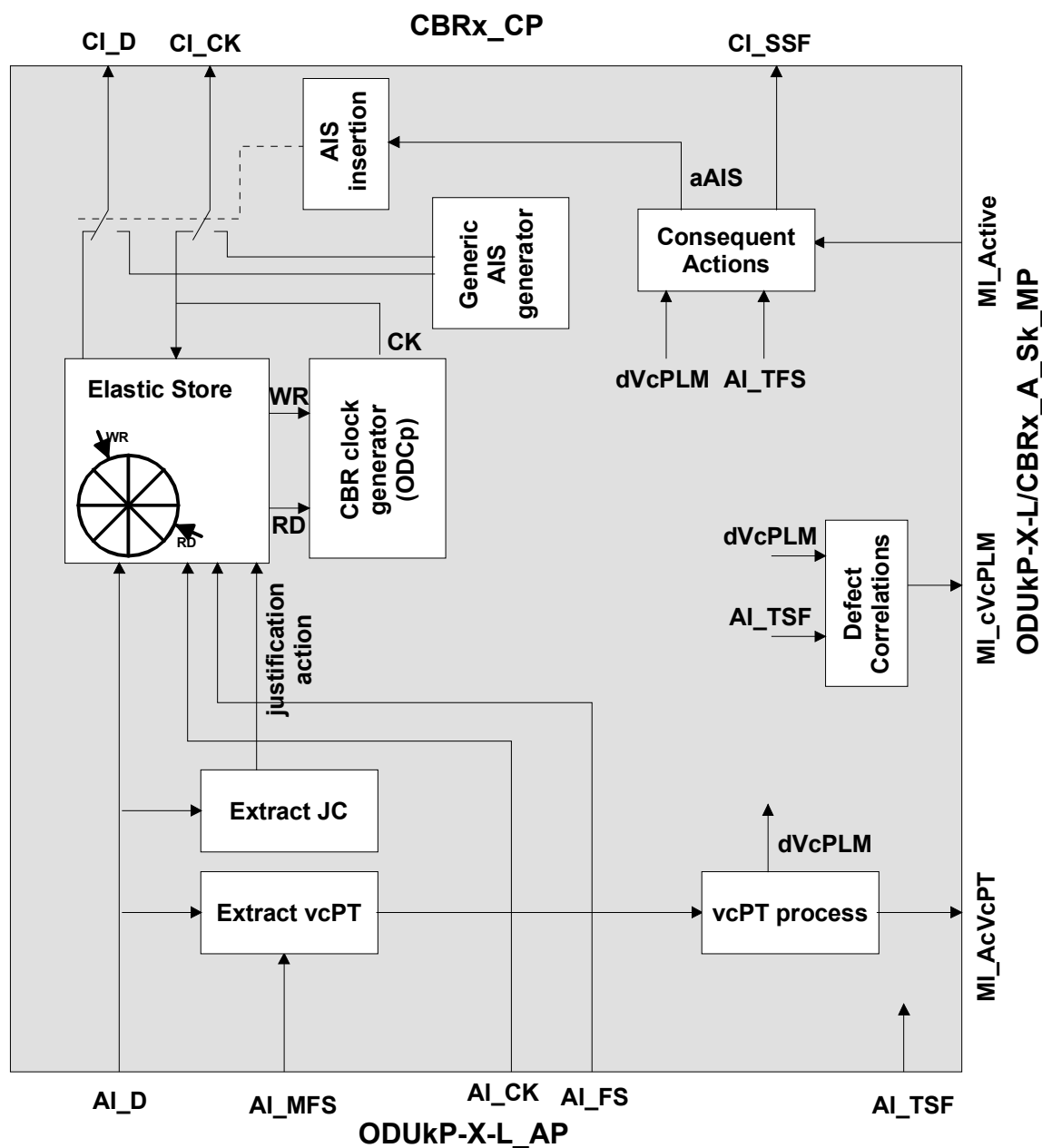
Figure 0-91/G.798 - ODUkP-X-L/CBRx A Sk processes
