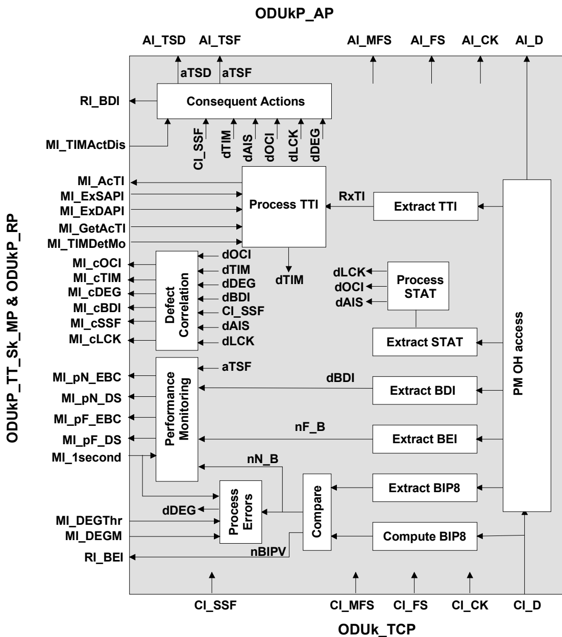
Figure 0-18/G.798 - ODUkP_TT_Sk processes
