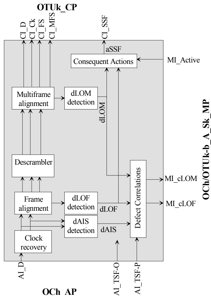
Figure 0-27/G.798 - OCh/OTUk-b_A_Sk processes
