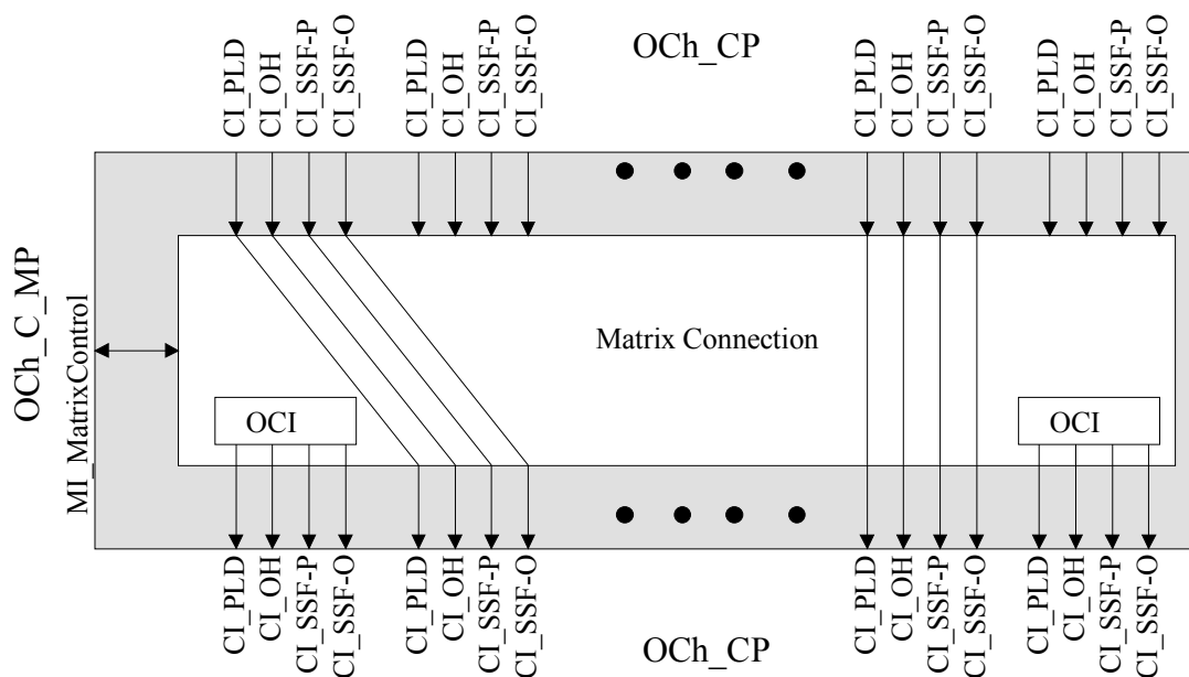
Figure 0-4/G.798 – OCh_C function processes
