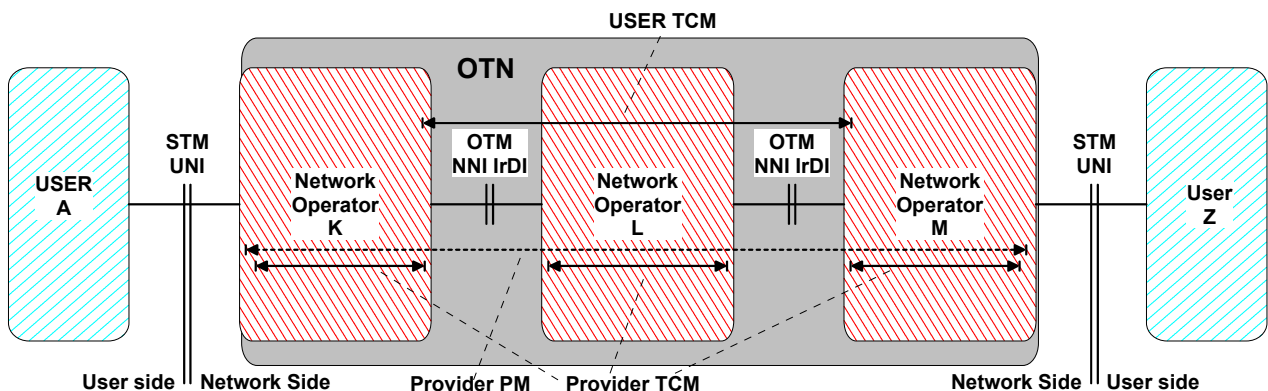
Figure II-1/G.798 - Provider and User Tandem Connections for case of STM-N UNI interface
