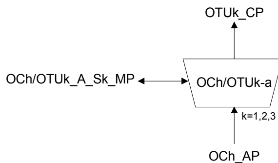
Figure 0-24/G.798 – OCh/OTUK-a_A_Sk function
