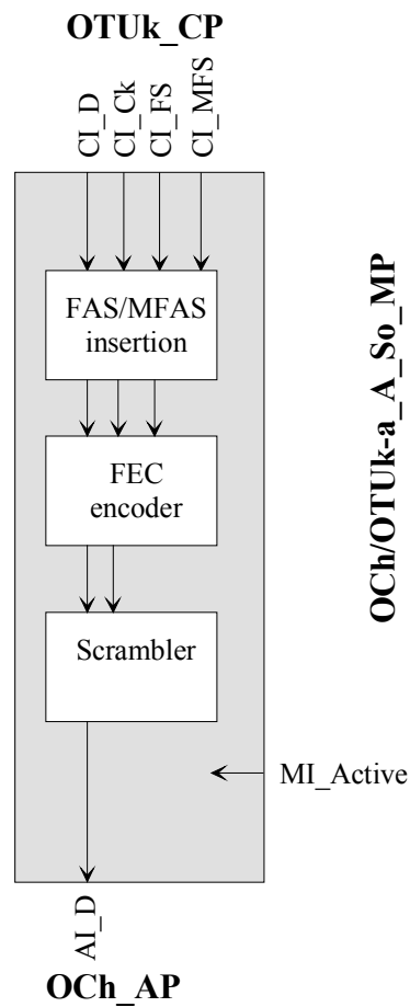
Figure 0-21/G.798 - OCh/OTUk-a_A_So processes
