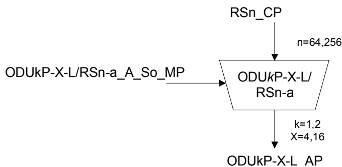
Figure 0_92/G.798 – ODUkP-X-L/RSn-a A So function
