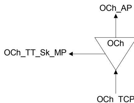
Figure 0-10/G.798 – OCh_TT_Sk function
