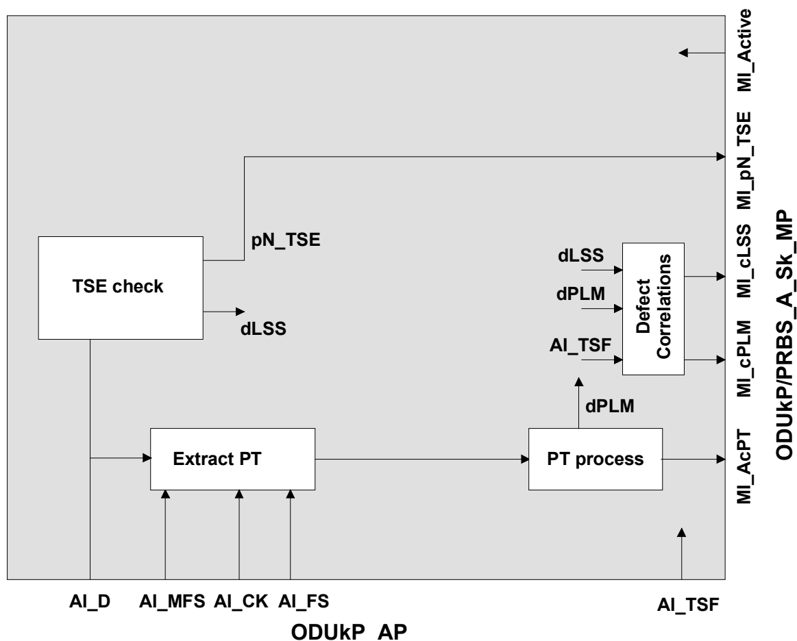
Figure 0-43/G.798 - ODUkP/PRBS_A_Sk processes
