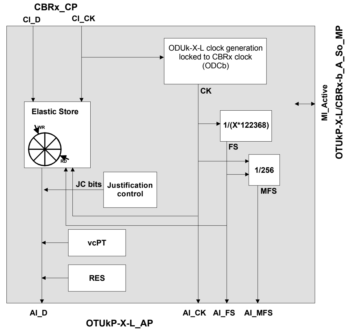
Figure 0-89/G.798 - ODUkP-X-L/CDRx-b A So processes
