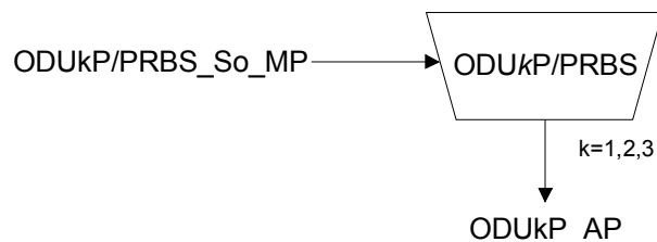
Figure 0-40/G.798 – ODUkP/PRBS_A_So function
