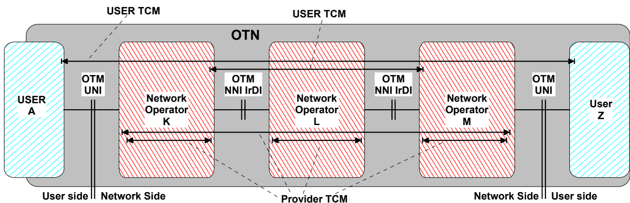
Figure II-4/G.798 - Provider and User Tandem Connections for case of OTM UNI interfaces and no termination of the OTN on the user side of the UNI
