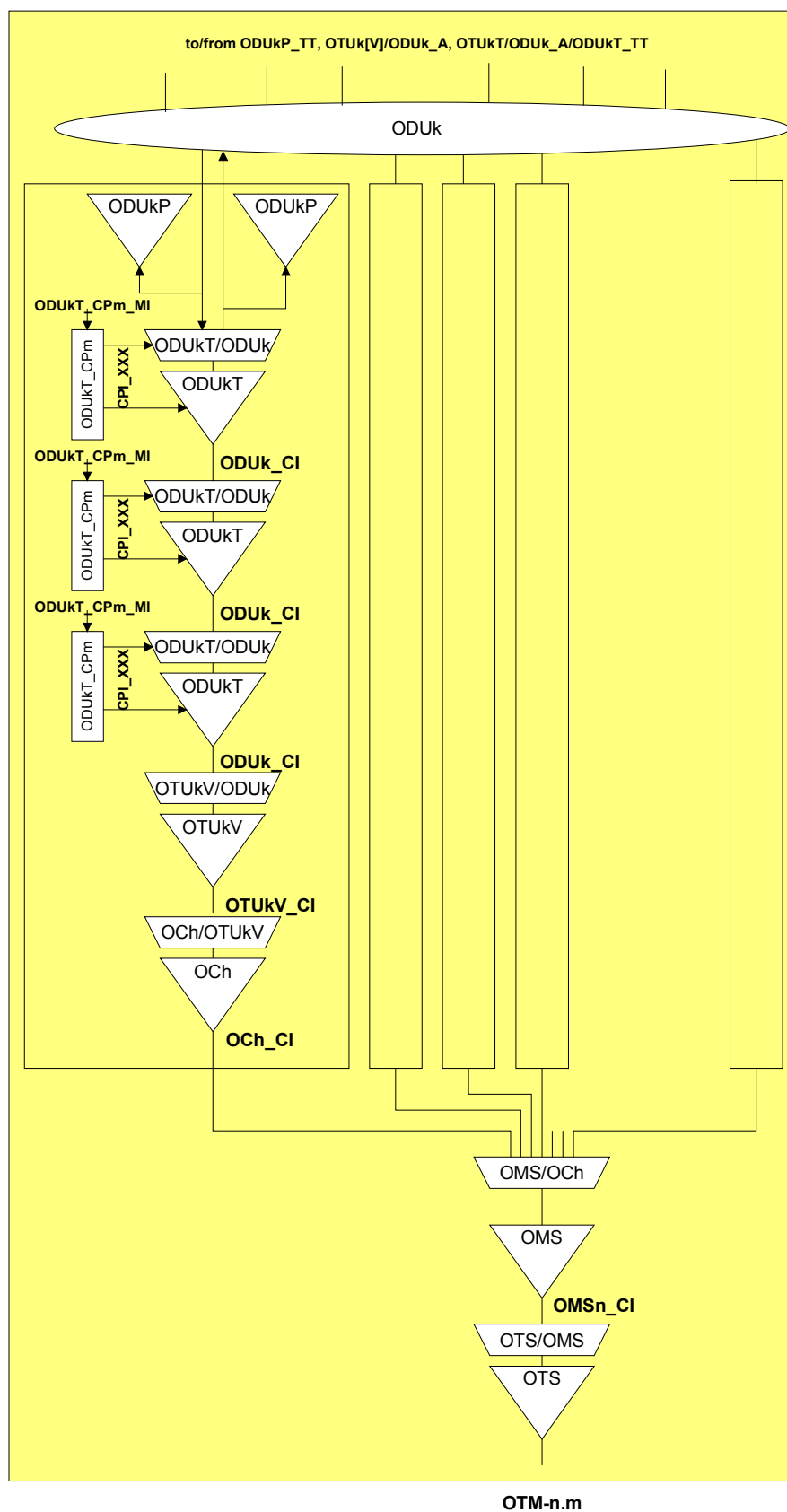
Figure I-6/G.798 - OTM-n.m interface port with 3-R regeneration functionality an ODUk connection function
