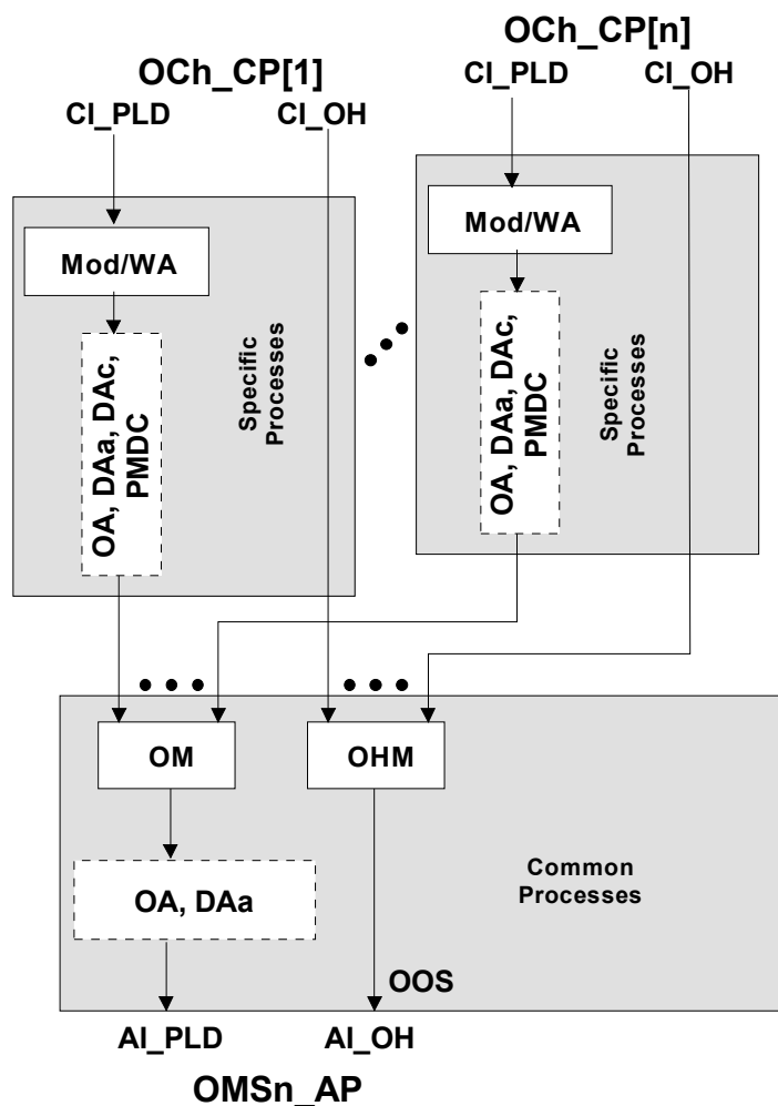
Figure 0-10/G.798 – OMSn/OCh_A_So processes
