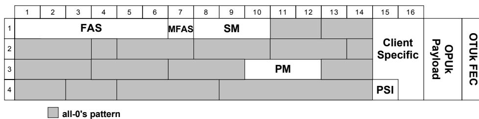
Figure I-5/G.798 – Minimum OTUk/ODUk overhead
