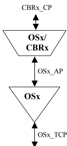
Figure I-1/G.798 – OSx layer network and client layer adaptation functions
