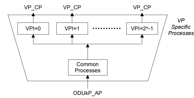
Figure 0-103/G.798 ODUkP-X-L/VP_A_Sk atomic function decomposed into Specific and Common Processes parts
