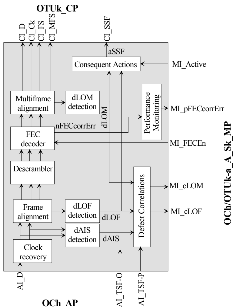
Figure 0-25/G.798 - OCh/OTUk-a_A_Sk processes
