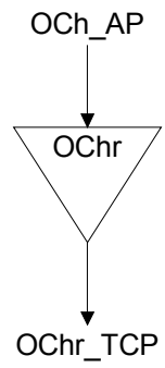
Figure 0-13/G.798 – OChr_TT_So function
