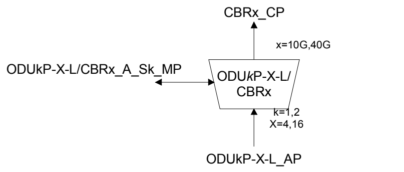
Figure 0-90/G.798 – ODUkP-X-L/CBRx A Sk function
