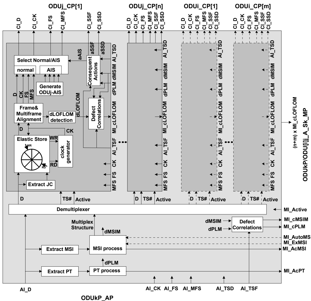
Figure 0-54/G.798 - ODUkP/ODUj[i]j_A_Sk processes
