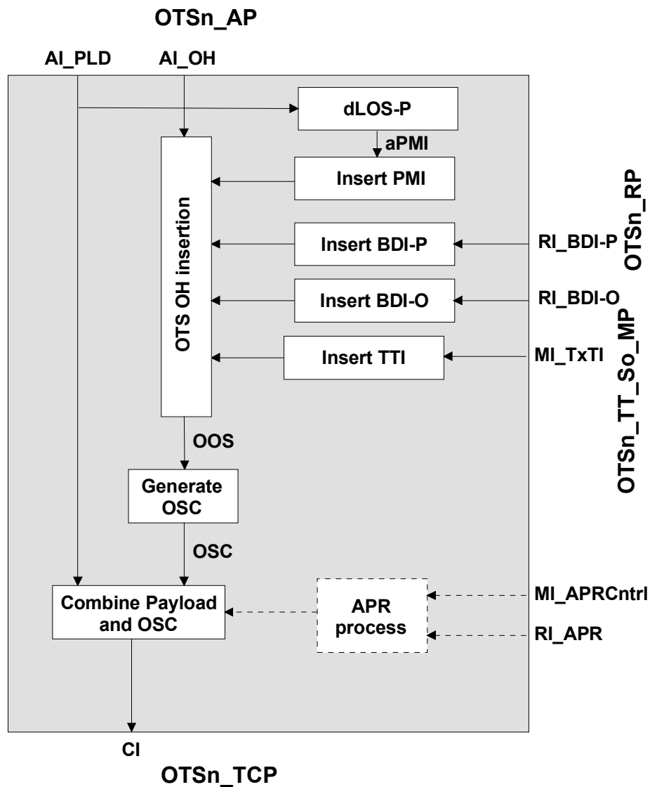
Figure 0-6/G.798 – OTSn_TT_So processes
