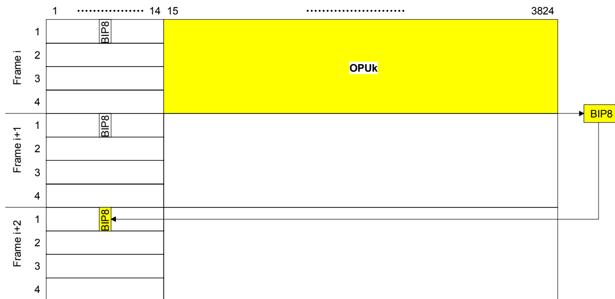
Figure 0-1/G.798 – BIP-8 source processing (SM OH used as example)
