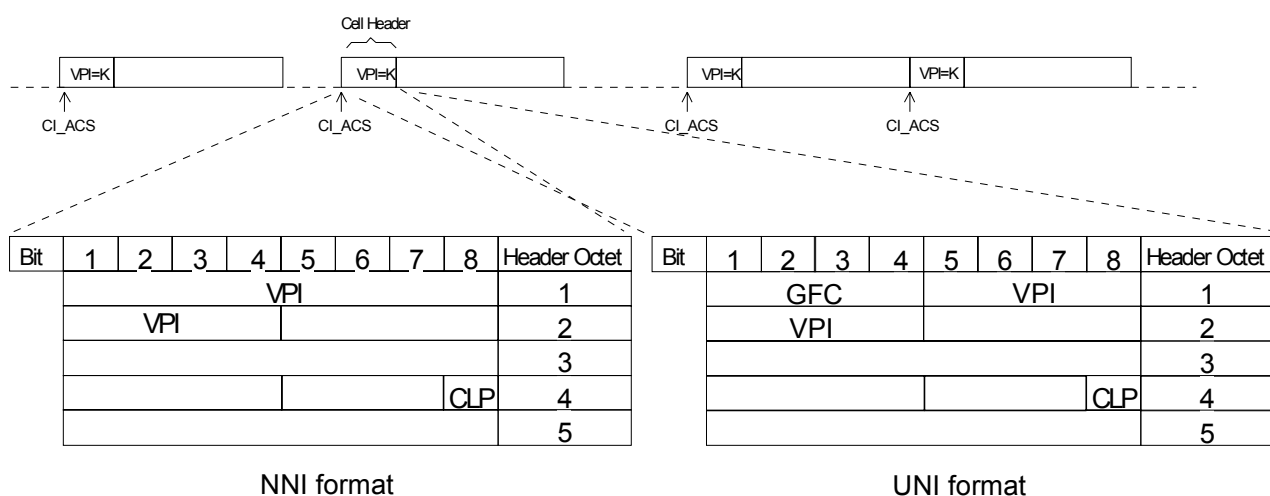
Figure 0_100/G.798 VP CI (NNI format)
