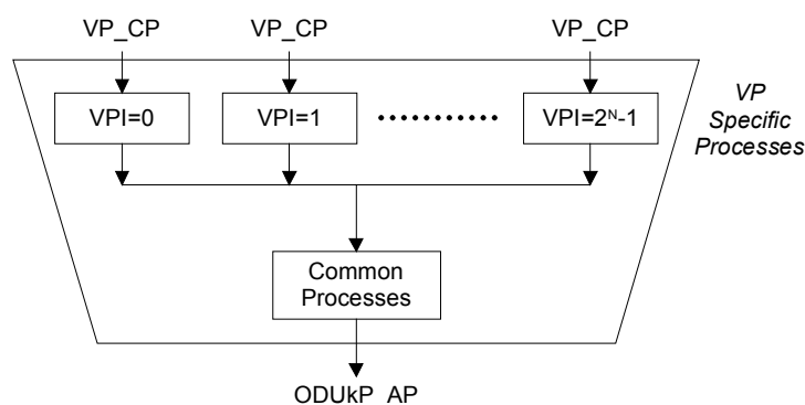
Figure 0-27/G.798 ODUkP/VP_A_So atomic function decomposed into Specific and Common Processes parts
