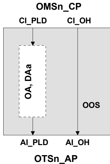
Figure 0-10/G.798 – OTSn/OMSn_A_So processes
