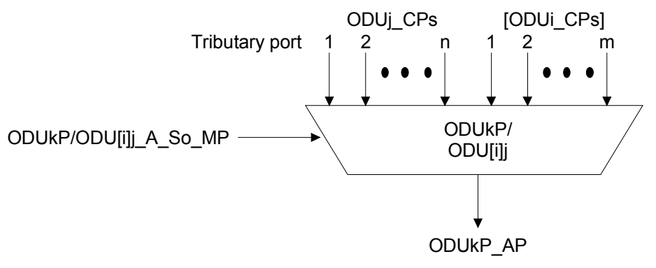
Figure 0-51/G.798 – ODUkP/ODU[i]j_A So function
