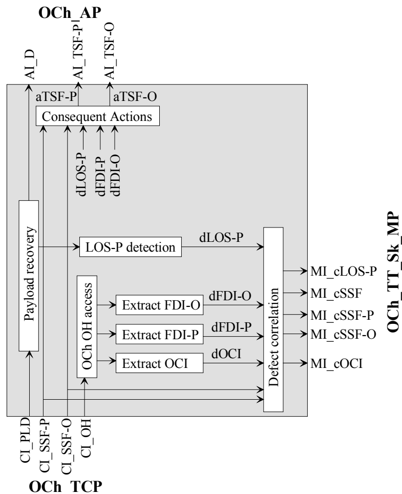
Figure 0-11/G.798 - OCh_TT_Sk processes
