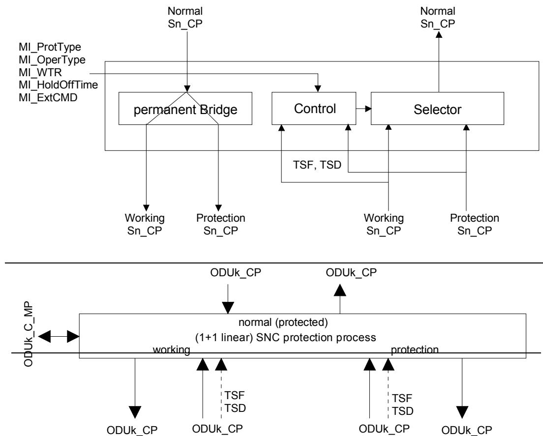
Figure 0-9/G.798 – 1+1 uni-directional SNC/N protection process without APS protocol
