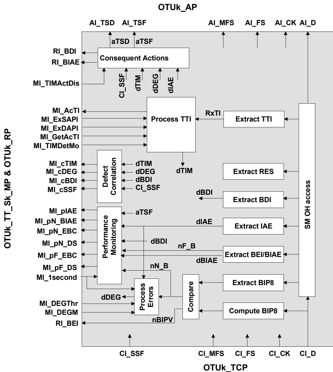
Figure 0-7/G.798 - OTUk_TT_Sk processes
