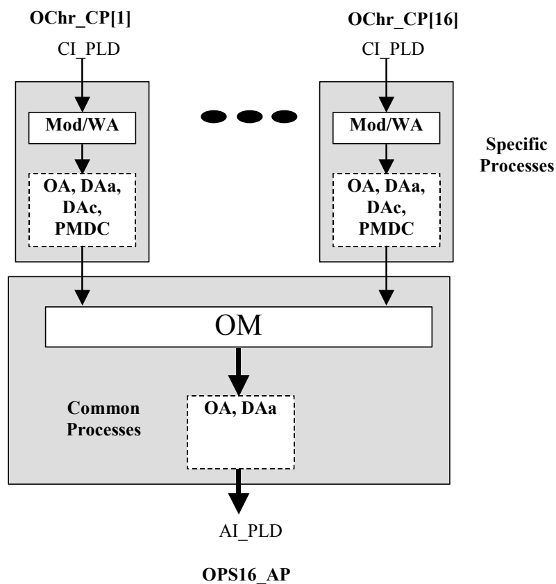
Figure 0-11/G.798 – OPS16/OChr_A_So processes
