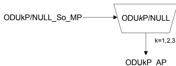
Figure 0-36/G.798 – ODUkP/NULL_A_So function
