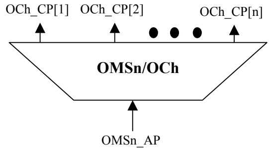
Figure 0-11/G.798 – OMSn/OCh_A_Sk function
