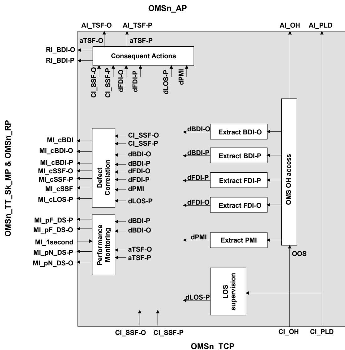
Figure 0-8/G.798 – OMSn_TT_Sk processes
