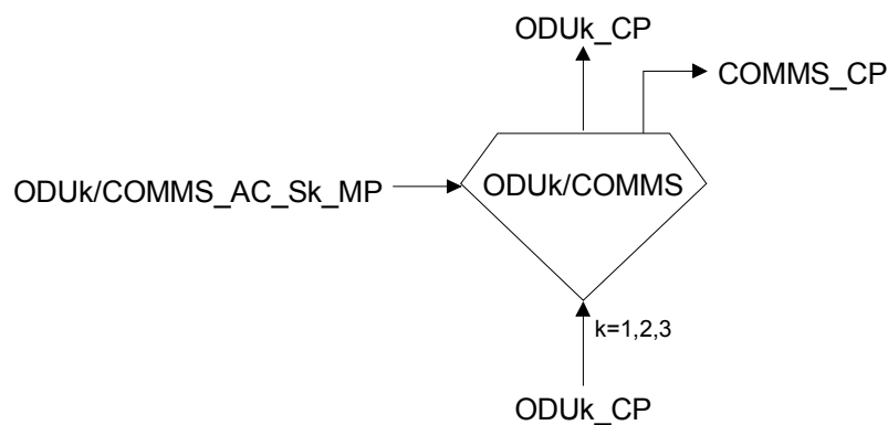
Figure 0-63/G.798 – ODUk/COMMS_AC_Sk function
