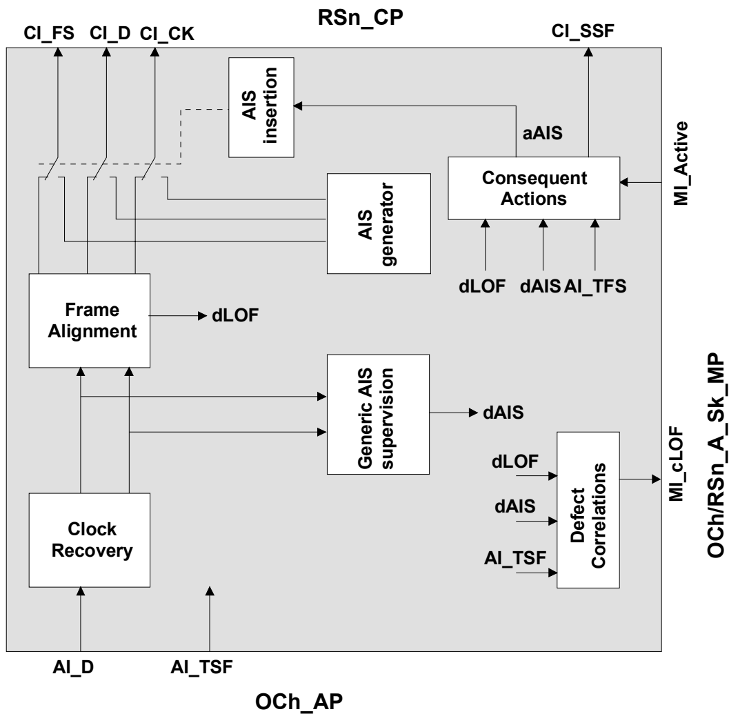
Figure 0-35/G.798 – OCh/RSn_A_Sk processes
