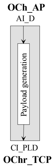
Figure 0-14/G.798 - OChr_TT_So processes
