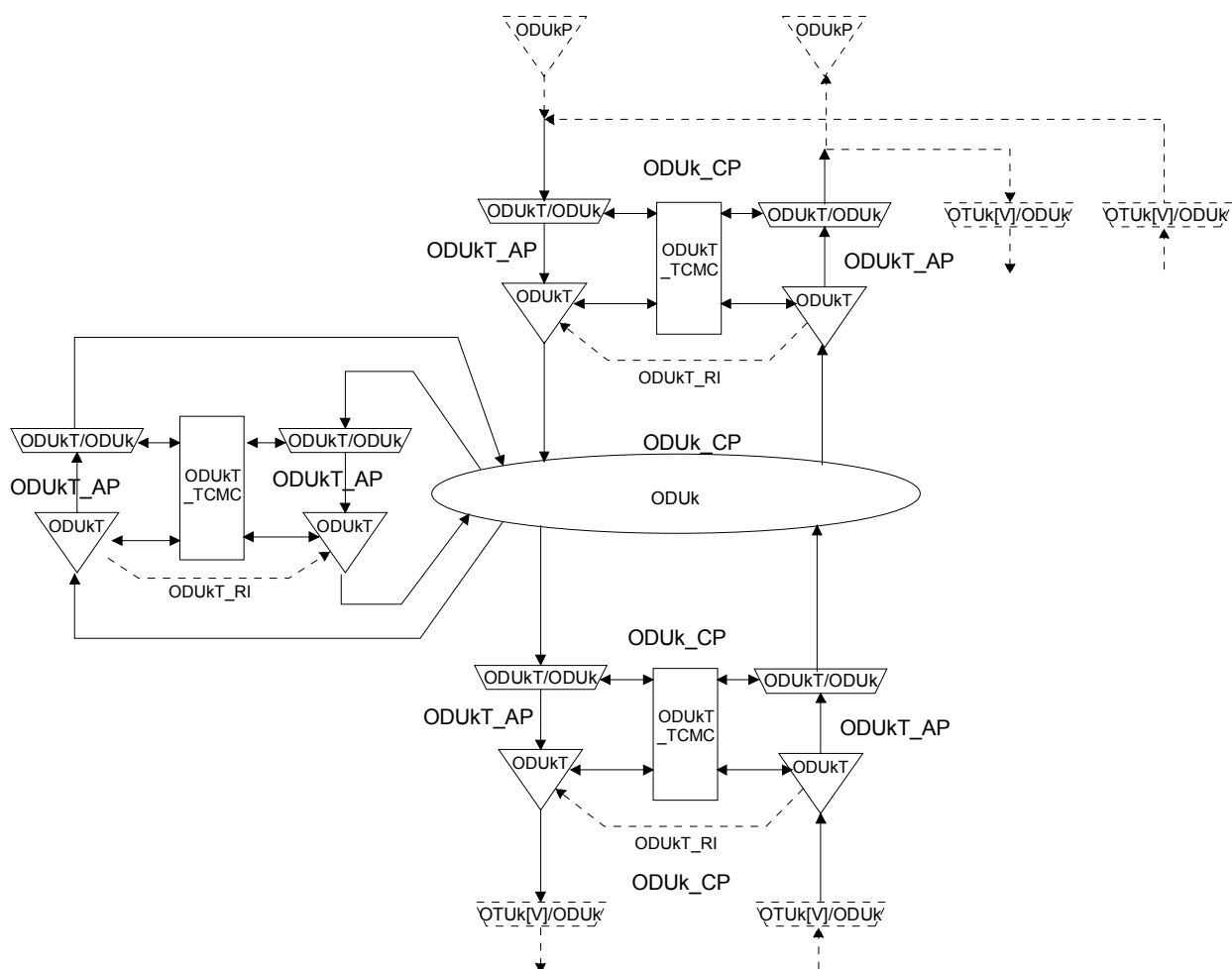
Figure 0-65/G.798 – Location of ODUkT_TT, ODUkT/ODUk_A and ODUkT_TCMC functions
