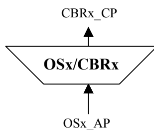
Figure I-9/G.798 – OSx/CBRx_A_Sk function
