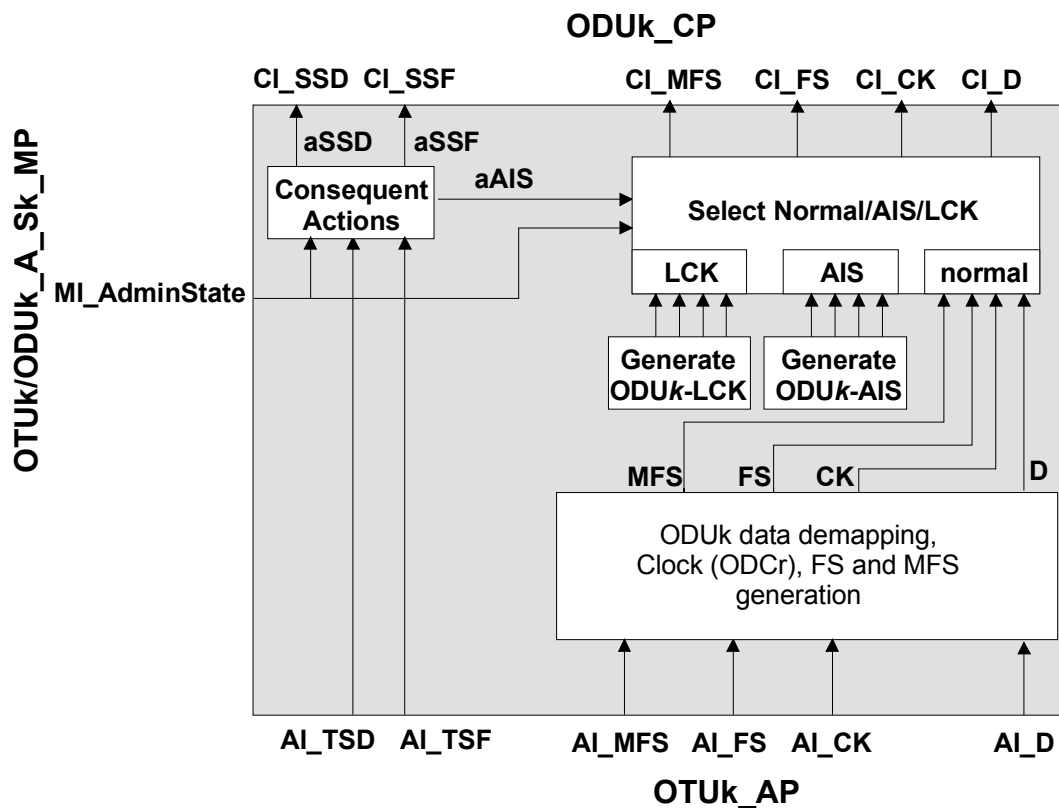
Figure 0-16/G.798 - OTUk/ODUk_A_Sk processes
