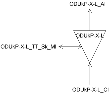
Figure 0_85/G.798 – ODUkP-X-L TT Sk symbol
