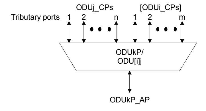
Figure 0-50/G.798 – ODUkP/ODU[i]j_A function
