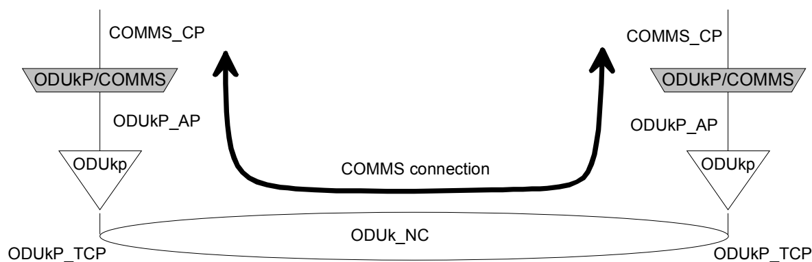
a) COMMS (GCC) access at ODUkP access points
