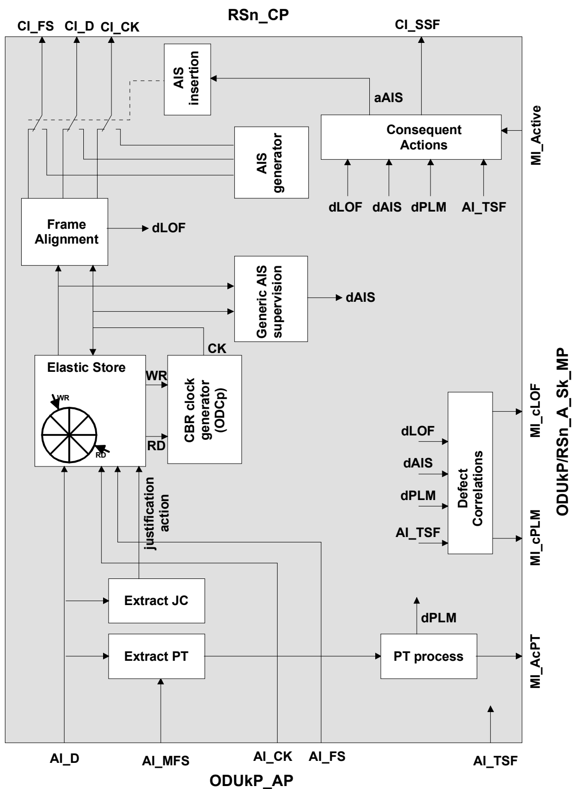
Figure 0-49/G.798 - ODUkP/RSn_A_Sk processes
