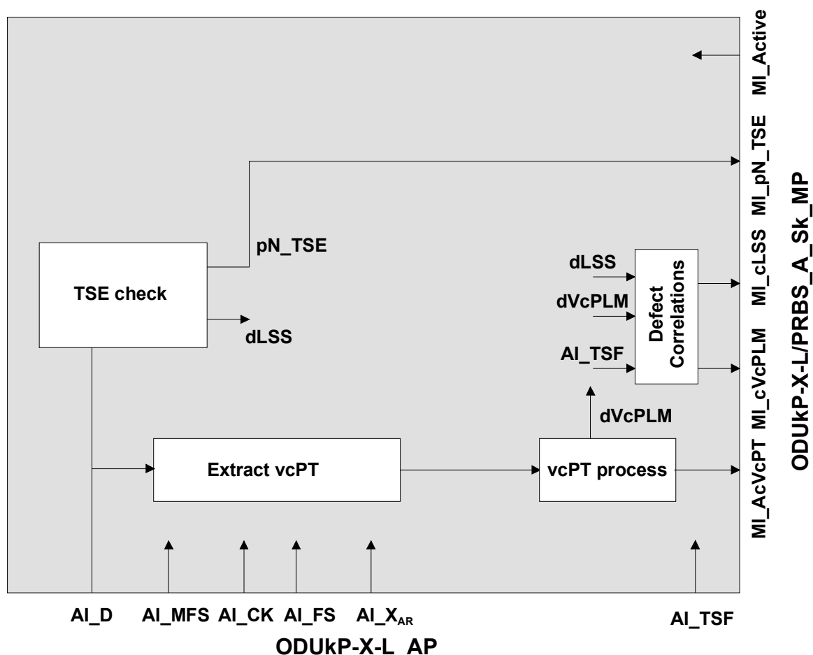
Figure 0-113/G.798 - ODUkP-X-L/PRBS_A_Sk processes
