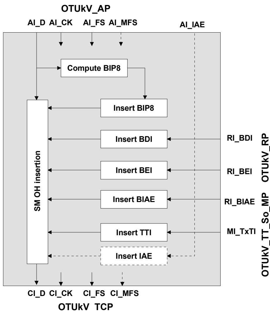
Figure 0-10/G.798 - OTUkV_TT_So processes
