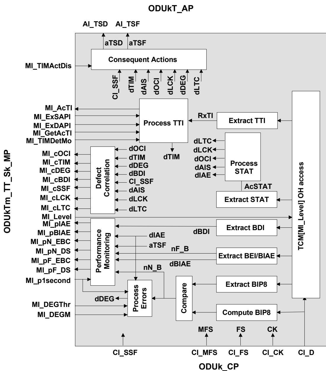
Figure 0-73/G.798 - ODUkTm_TT_Sk processes
