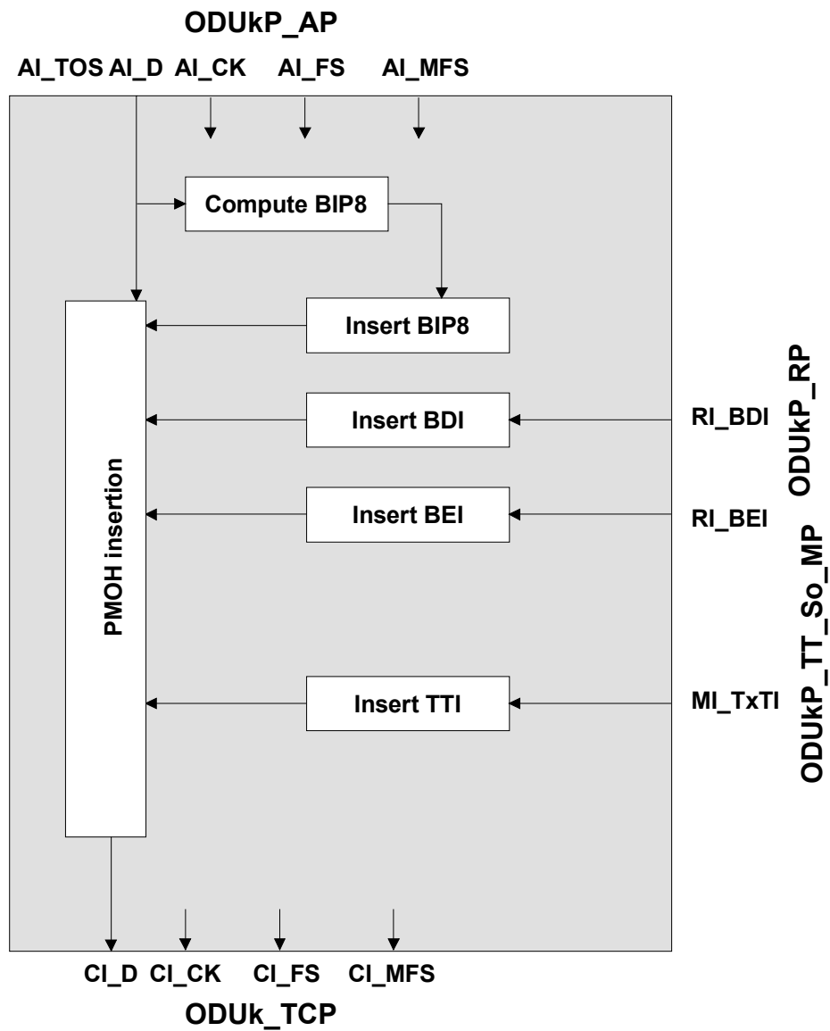
Figure 0-16/G.798 - ODUkP_TT_So processes
