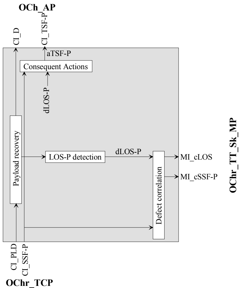
Figure 0-16/G.798 - OChr_TT_Sk processes
