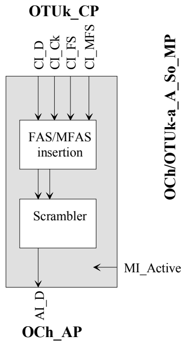
Figure 0-23/G.798 - OCh/OTUK-b_A_So processes
