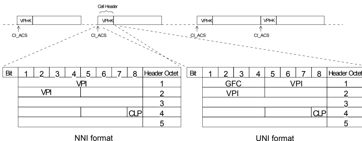
Figure 0-28/G.798 VP_CI (NNI format)
