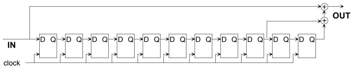
Figure 0-5/G.798 – Inverse PN-11 process for GenericAIS detection
