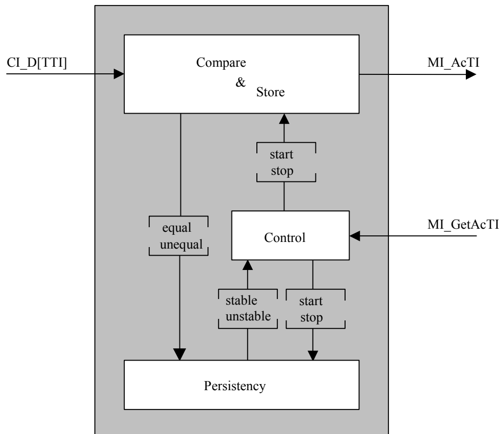
Figure IV-1/G.798 - TTI Reporting Process
