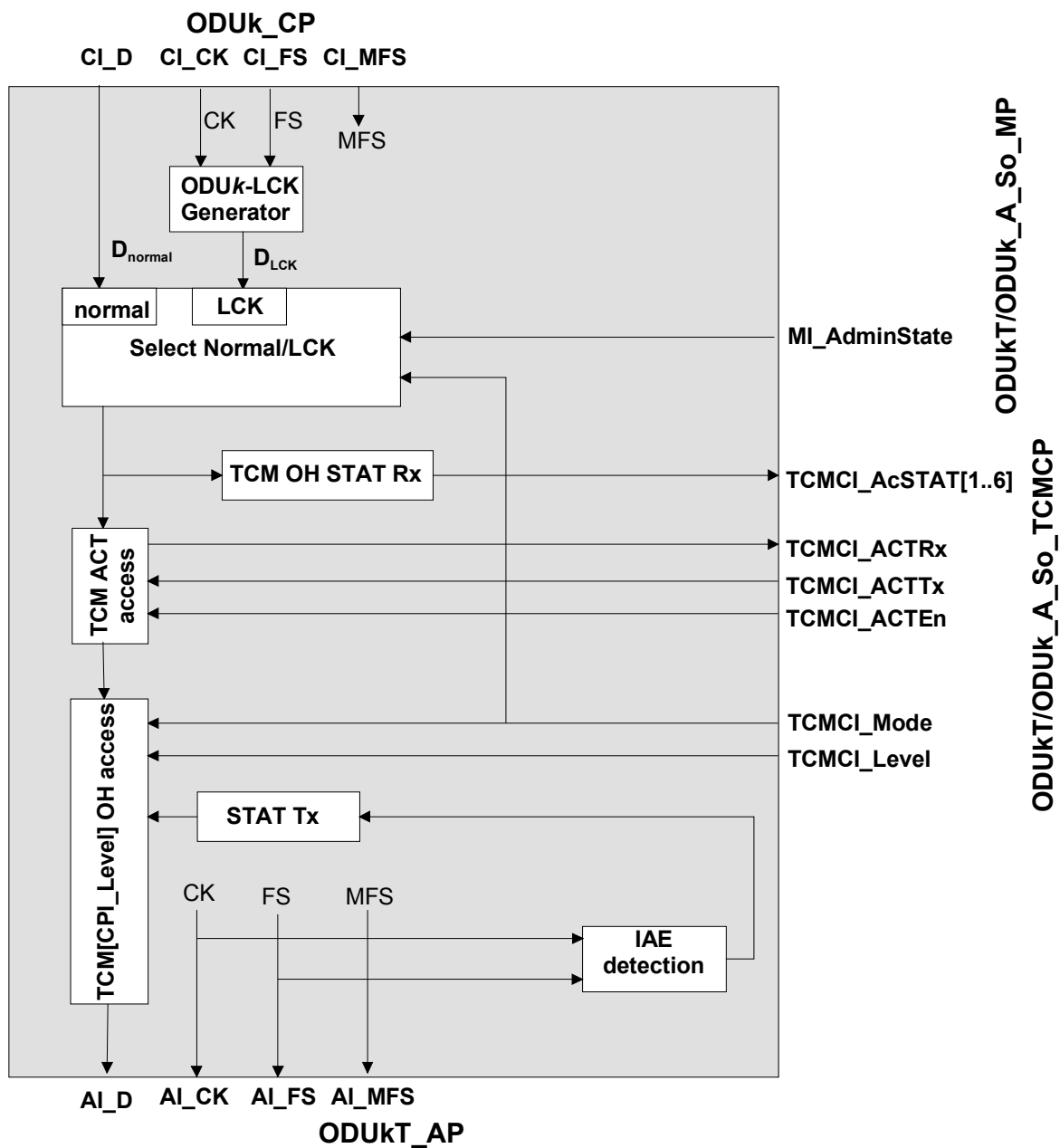
Figure 0-75/G.798 - ODUkT/ODUk_A_So processes
