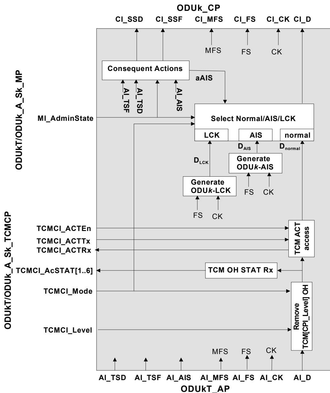
Figure 0-77/G.798 - ODUkT/ODUk_A_Sk processes
