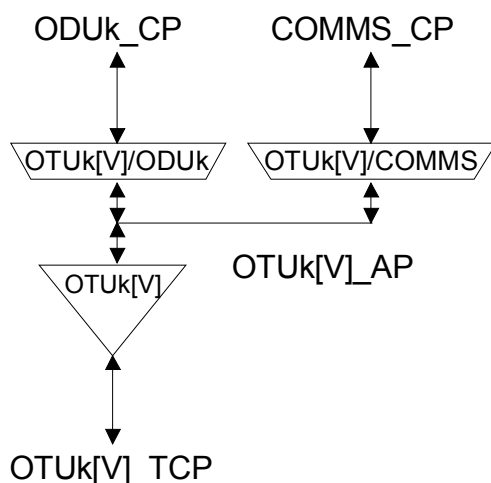
Figure 0-1/G.798 – OTUk[V] layer network and client layer adaptation functions
