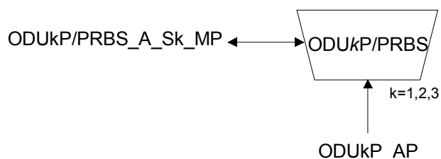
Figure 0-42/G.798 – ODUkP/PRBS_A_Sk function
