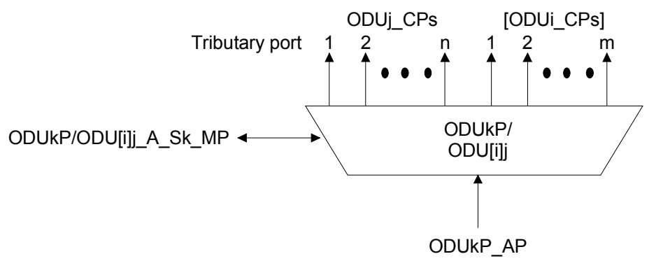
Figure 0-53/G.798 – ODUkP/ODU[i]j_A_Sk function
