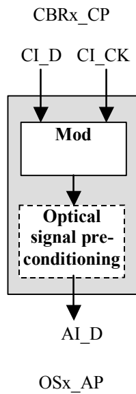
Figure I-8/G.798 – OSx/CBRx_A_So processes
