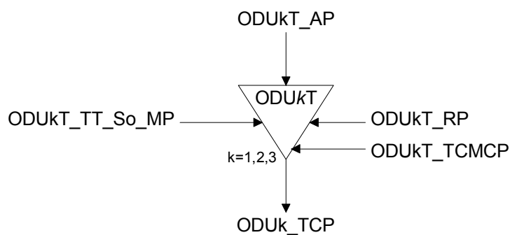
Figure 0-67/G.798 – ODUkT_TT_So function
