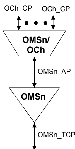
Figure 0-1/G.798 – OMS layer network and client layer adaptation functions
