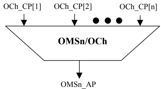
Figure 0-9/G.798 – OMSn/OCh_A_So function
