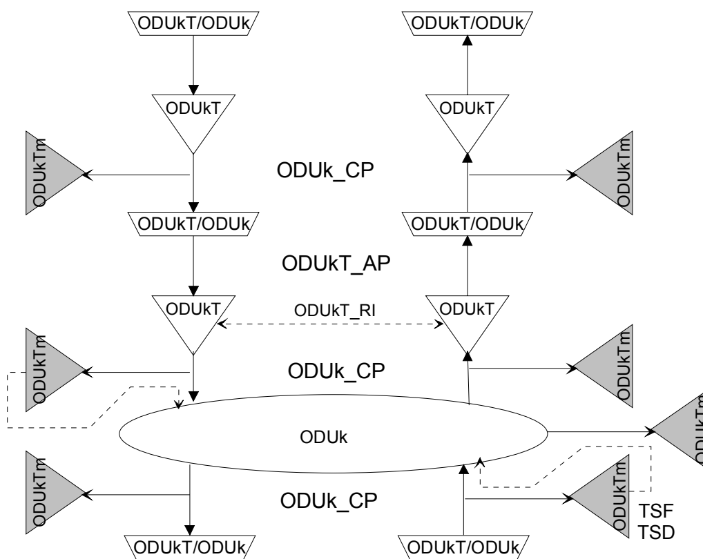
Figure 0-71/G.798 – Connection of ODUkTm_TT_Sk function (non-intrusive monitor)
