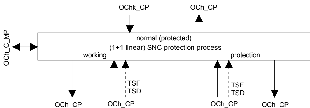
Figure 0-6/G.798 – SNC/N protection process
