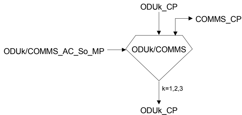
Figure 0-61/G.798 – ODUk/COMMS_AC_So function
