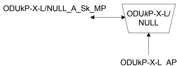
Figure 0-108/G.798 – ODUkP-X-L/NULL A Sk function
