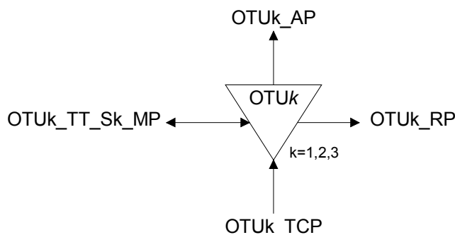
Figure 0-11/G.798 – OTUkV_TT_Sk function
