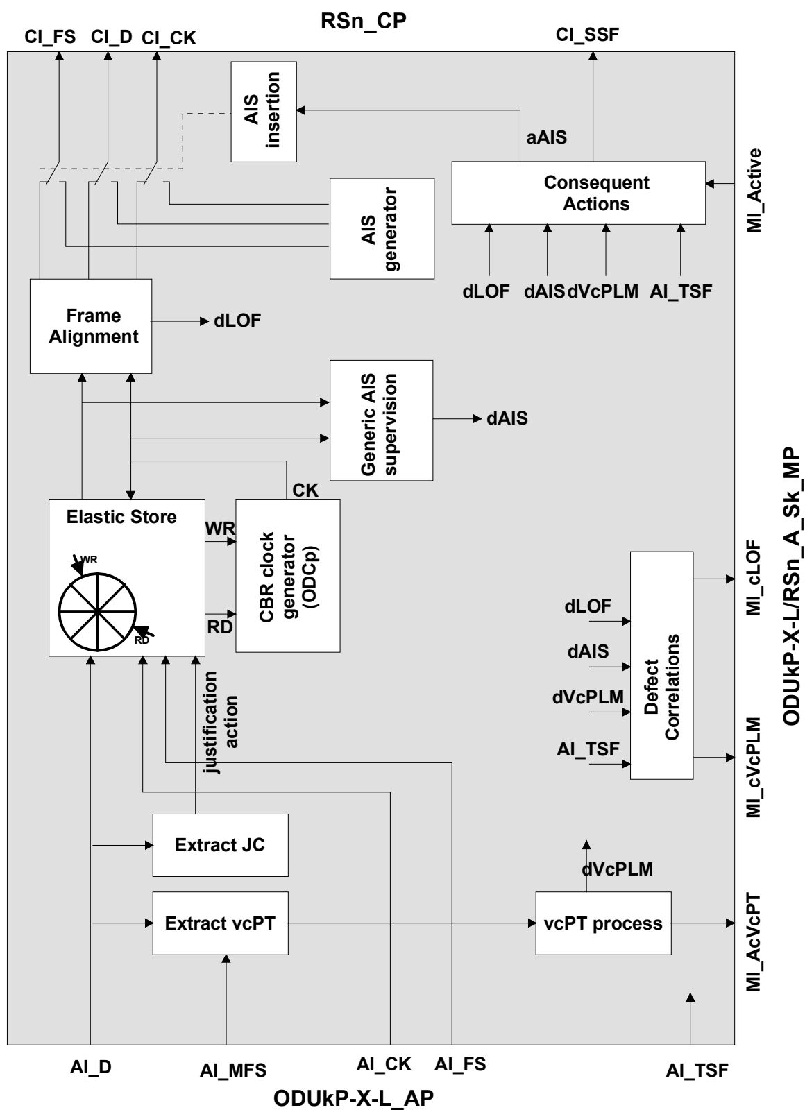
Figure 0-97/G.798 - ODUkP-X-L/RSn A Sk processes
