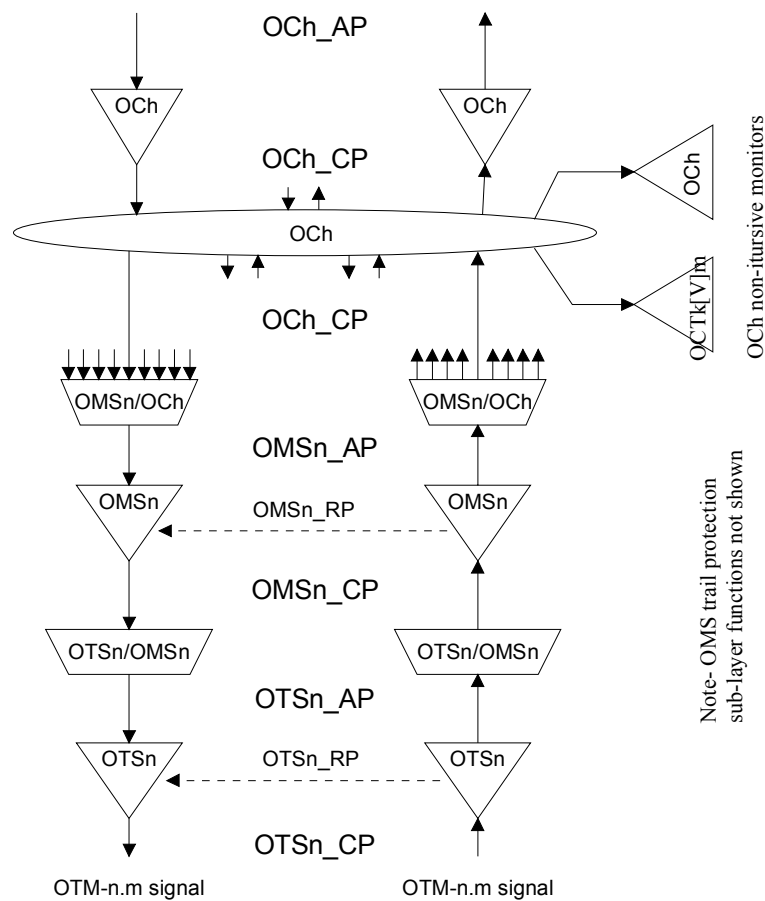
Figure 0-2/G.798 - OTN atomic functions specific for the full functionality OTM-n.m interface
