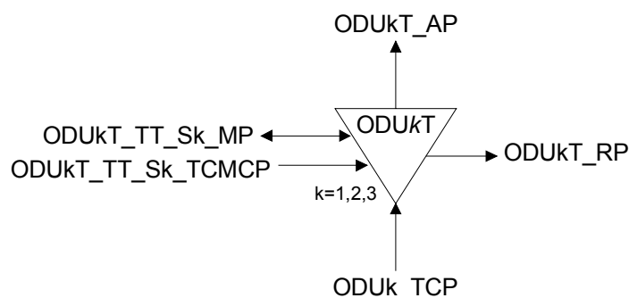
Figure 0-69/G.798 – ODUkT_TT_Sk function
