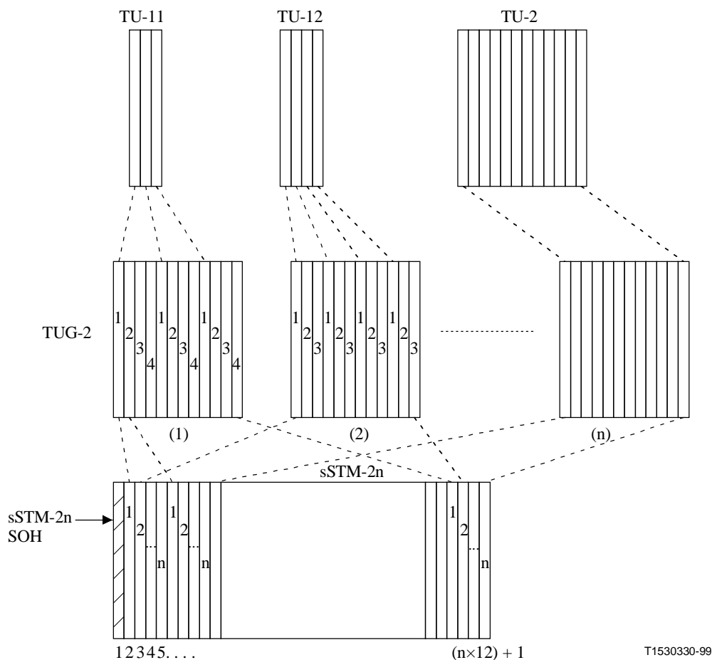
Figure 7/G.708 – Arrangement of n \times TUG-2s multiplexed into a sSTM-2n ( n = 1, 2, 4 )
