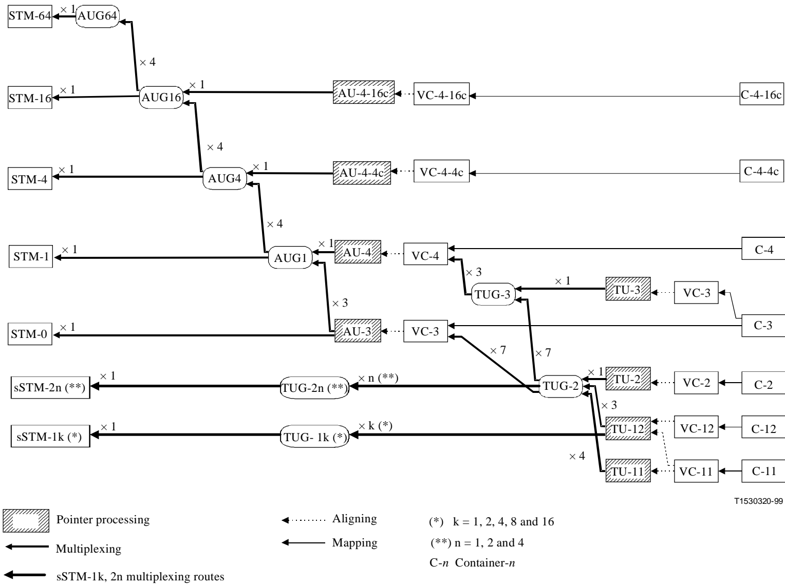
Figure 6/G.708 – Integration of sSTM formats into the G.707 multiplexing structure
