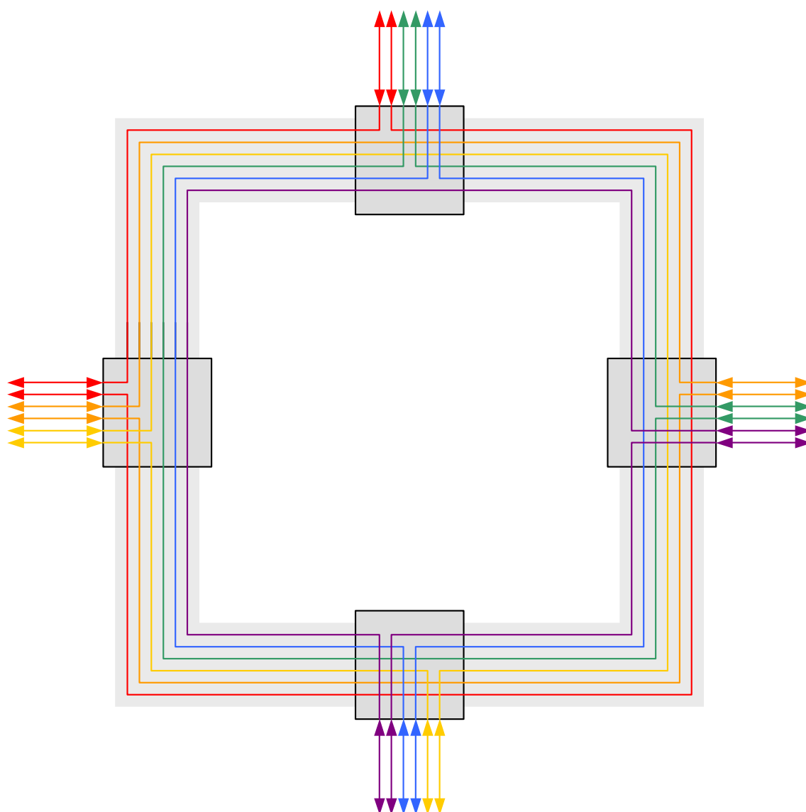
Figure III.2/G.695 – Complex example of ring black-link topology
