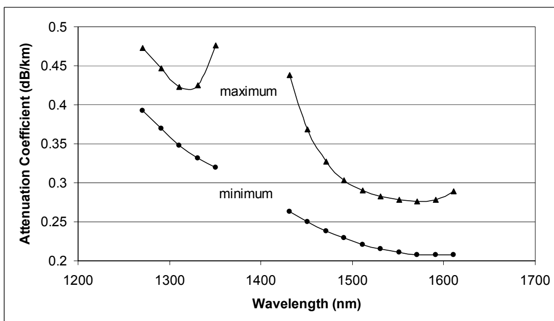
Figure I.1/G.695 – Assumed attenuation coefficient values for G.652.A&B cable
