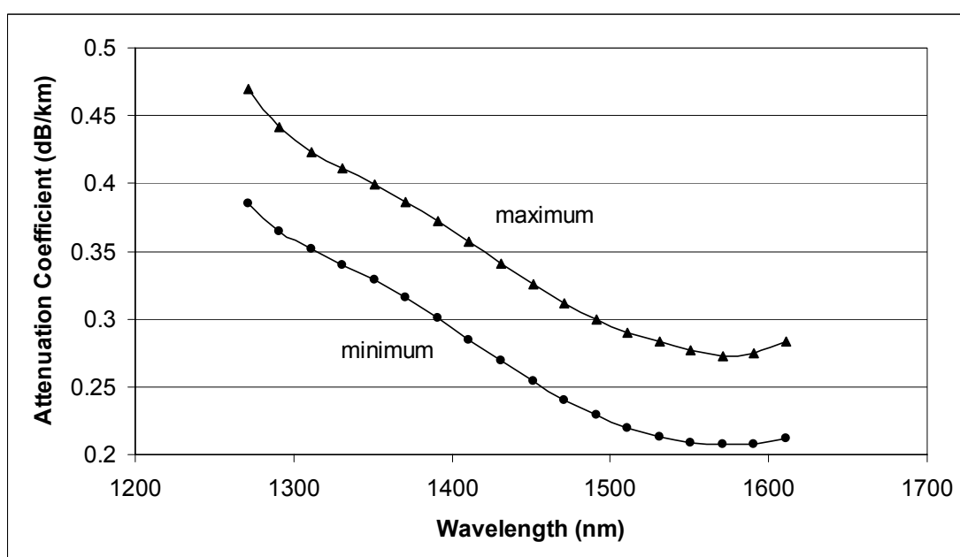
Figure I.2/G.695 – Assumed attenuation coefficient values for G.652.C&D cable
