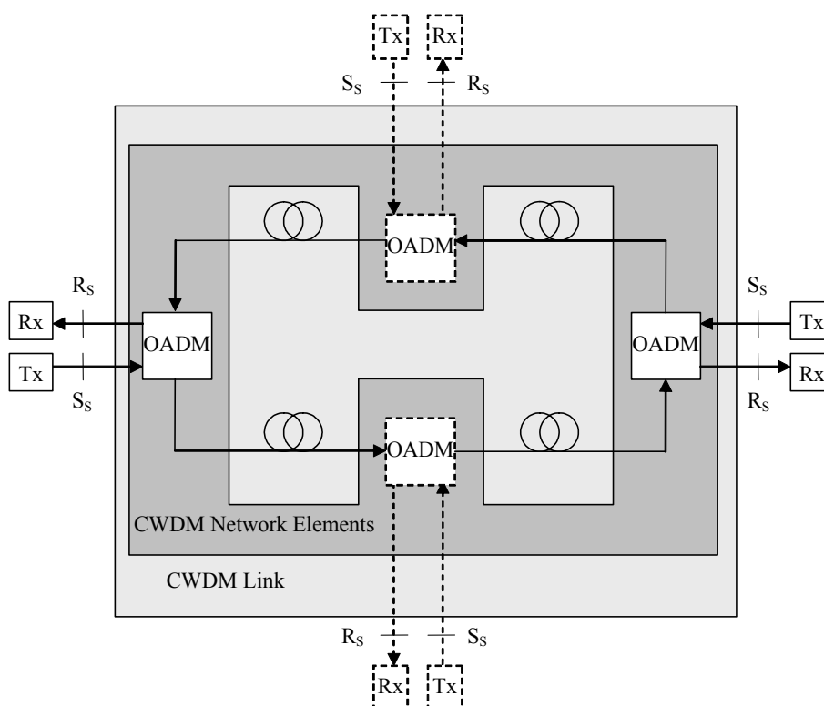
Figure 5-3/G.695 – Ring “black-link” approach
