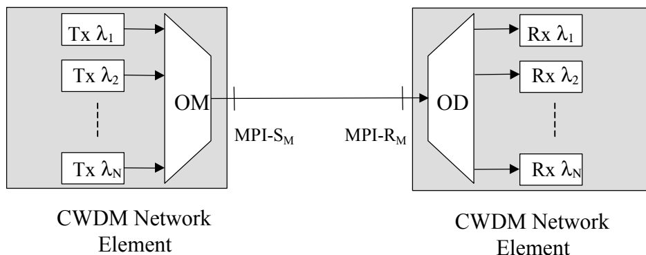
Figure 5-1/G.695 – “Black-box” approach
