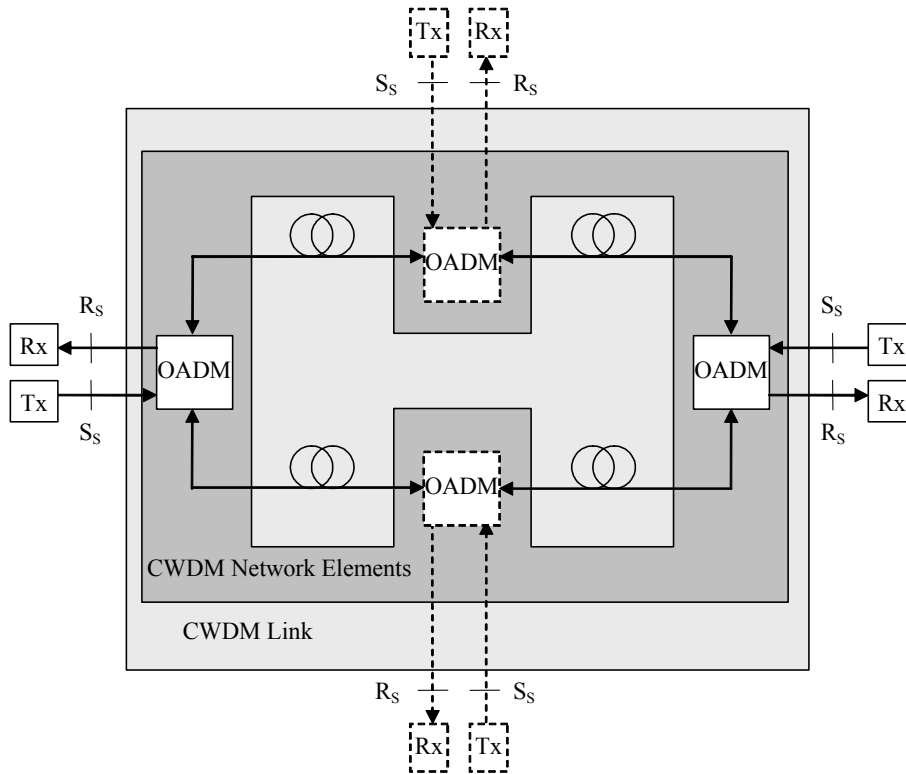
Figure 5-6/G.695 – Ring “black-link” approach for bidirectional applications
