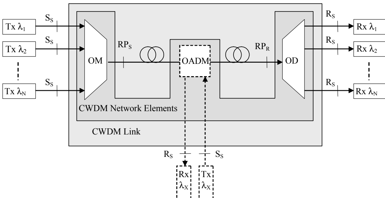
Figure 5-2/G.695 – Linear “black-link” approach
