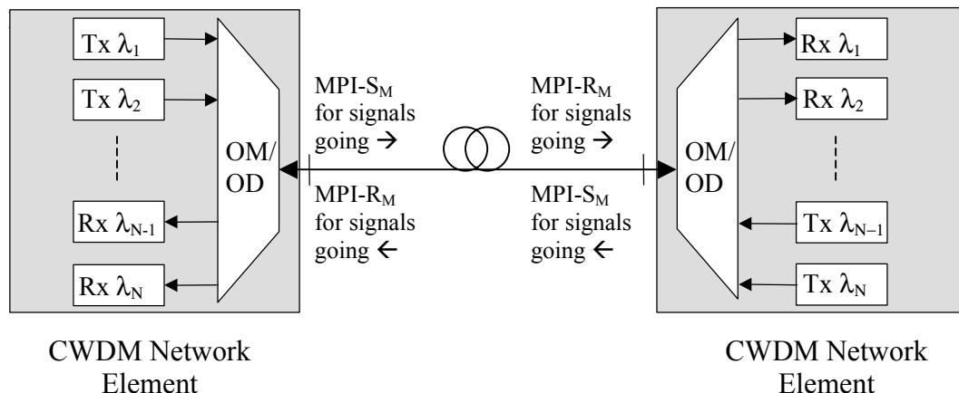
Figure 5-4/G.695 “Black Box” Approach for Bidirectional Applications
