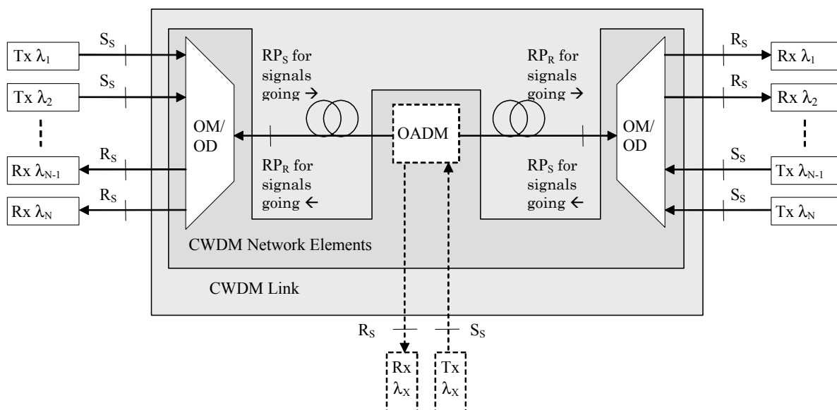
Figure 5-5/G.695 Linear “black Link” Approach for Bidirectional Applications
